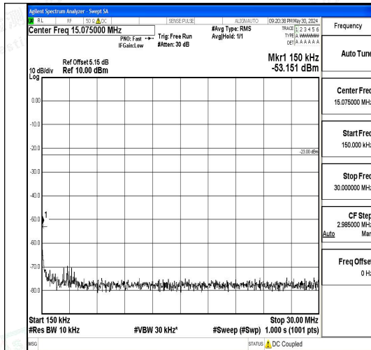
Band5_3MHz_16QAM_20525_1RB#0_0.15~30_0.15~30
