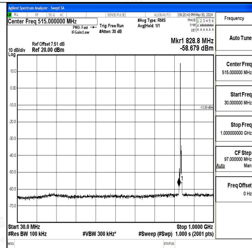
Band5_3MHz_16QAM_20525_1RB#0_30~1000_0~1000
