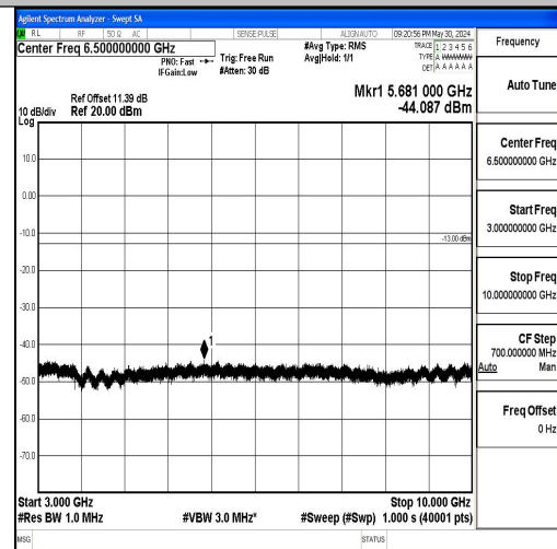
Band5_3MHz_16QAM_20525_1RB#0_3000~1000_0_3000~10000
