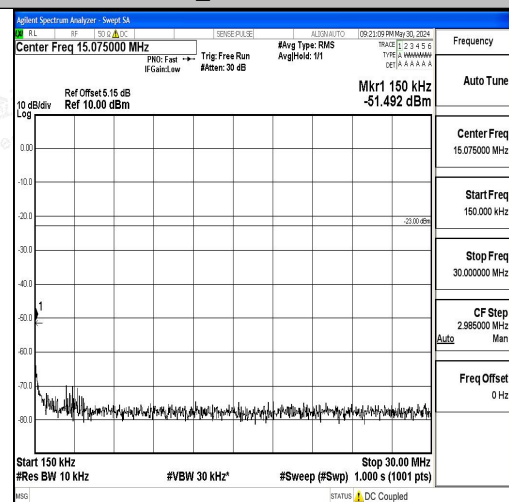
Band5_3MHz_QPSK_20635_1RB#0_0.15~30_0.1_5~30
