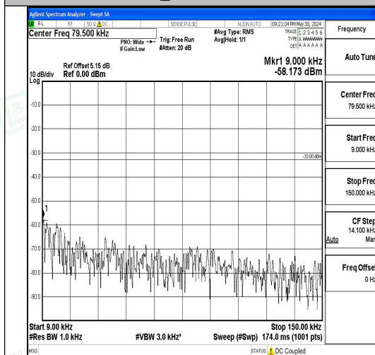
Band5_3MHz_QPSK_20635_1RB#0_0.009~0.15_0.009~0.15
