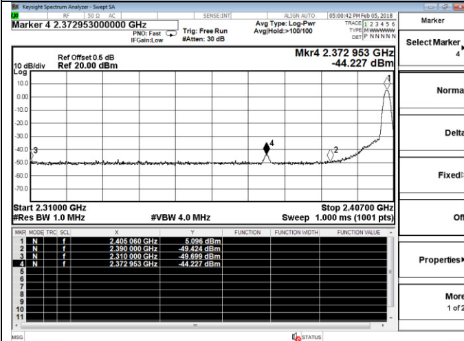
Channel 0 / 2405 MHz – Peak
