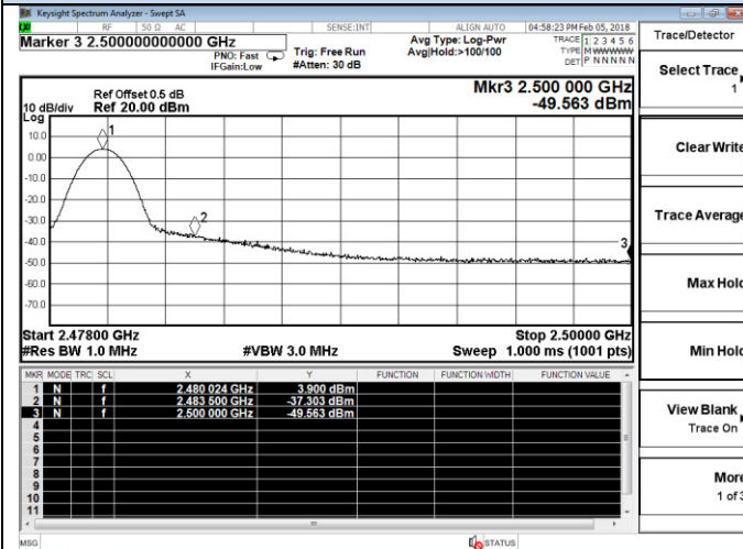
Channel 15 / 2480 MHz – Peak
