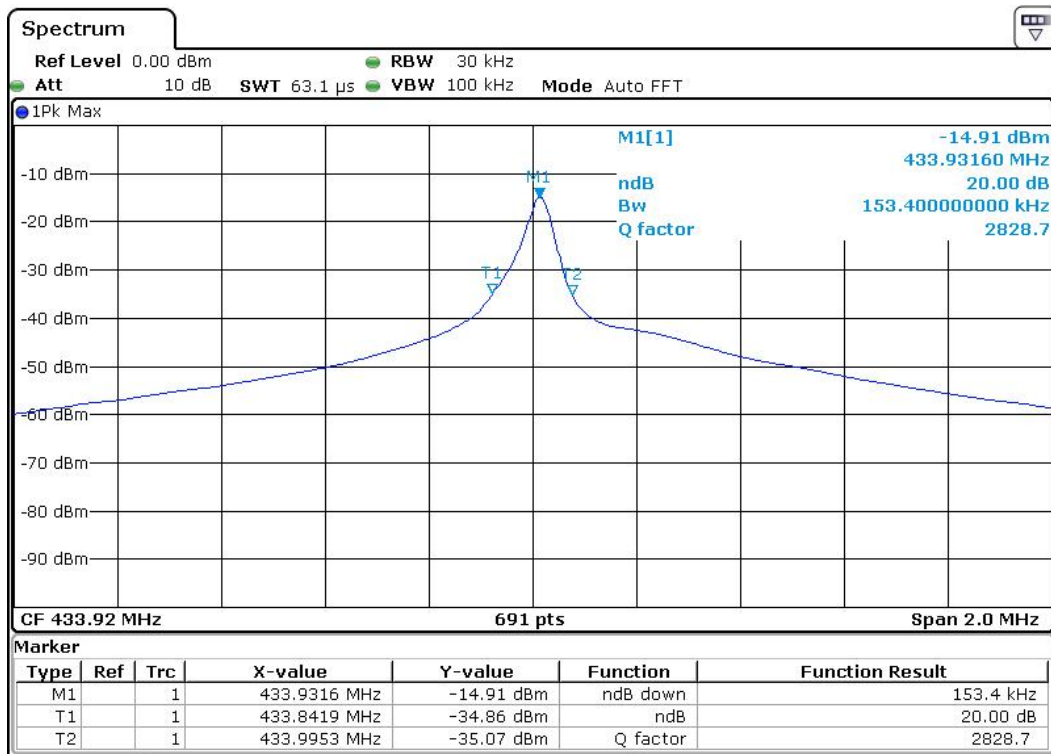
Channel 01: 433.92MHz
