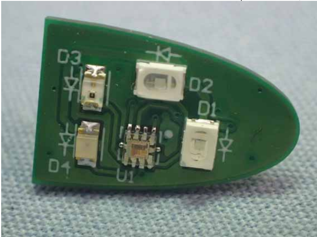
Figure 13 Internal View (Sensor Board, Back View)
