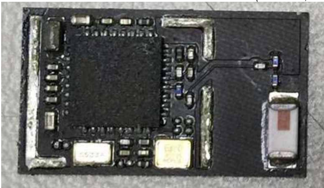
Figure 14 Internal View (RF Module, Front View)
