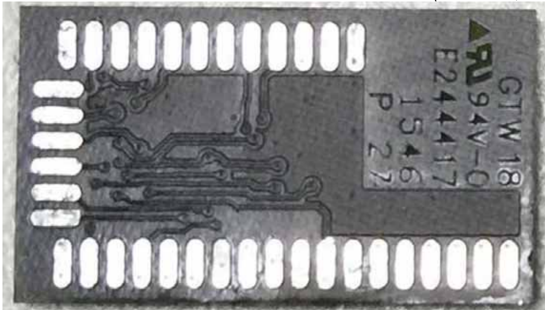
Figure 15 Internal View (RF Module, Back View)
