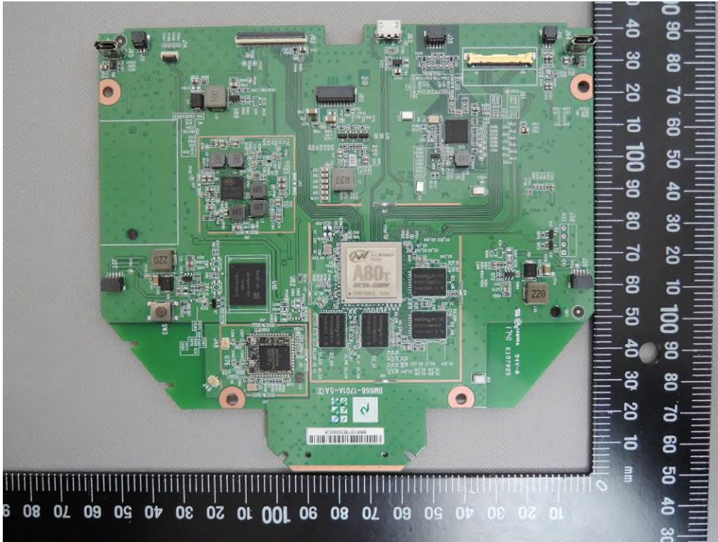
Internal View of EUT-4(A80T)
