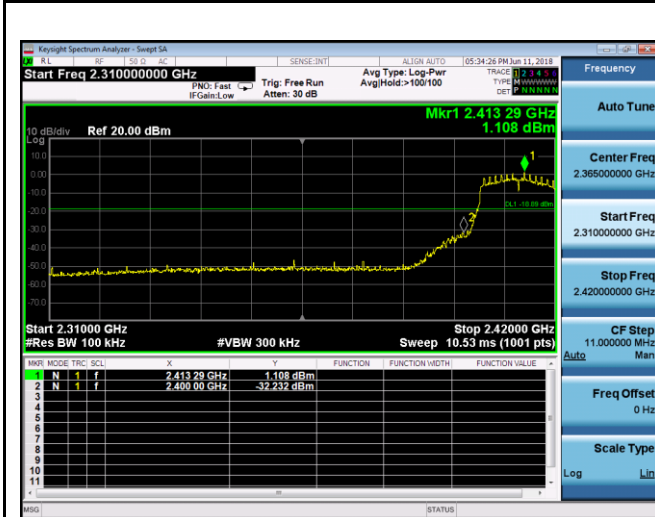
Band Edge, Left Side - 802.11b
