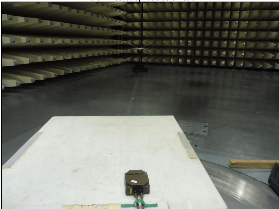
Photo 2: Test setup for radiated emission testing
