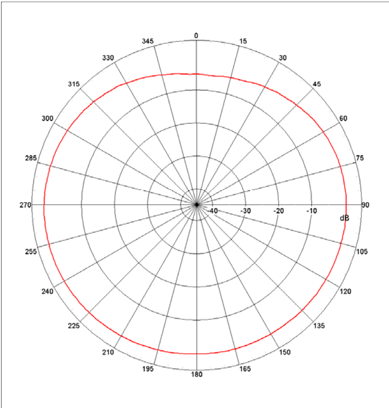
Far-field Power Distribution(H+V) on X-Y Plane Plot Peak Gain(H+V)= 1.3 dBi; Plot AvgGain(H+V)= -0.48dBi @2.44000 GHz
