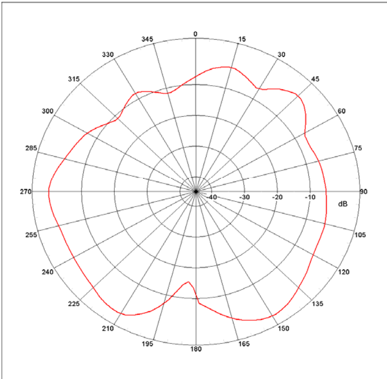
Far-field Power Distribution(H+V) on X-Z Plane Plot Peak Gain(H+V)= 1.1 dBi; Plot AvgGain(H+V)= -3.83dBi @2.44000 GHz
