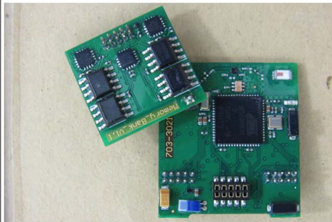
VIEW B.8
