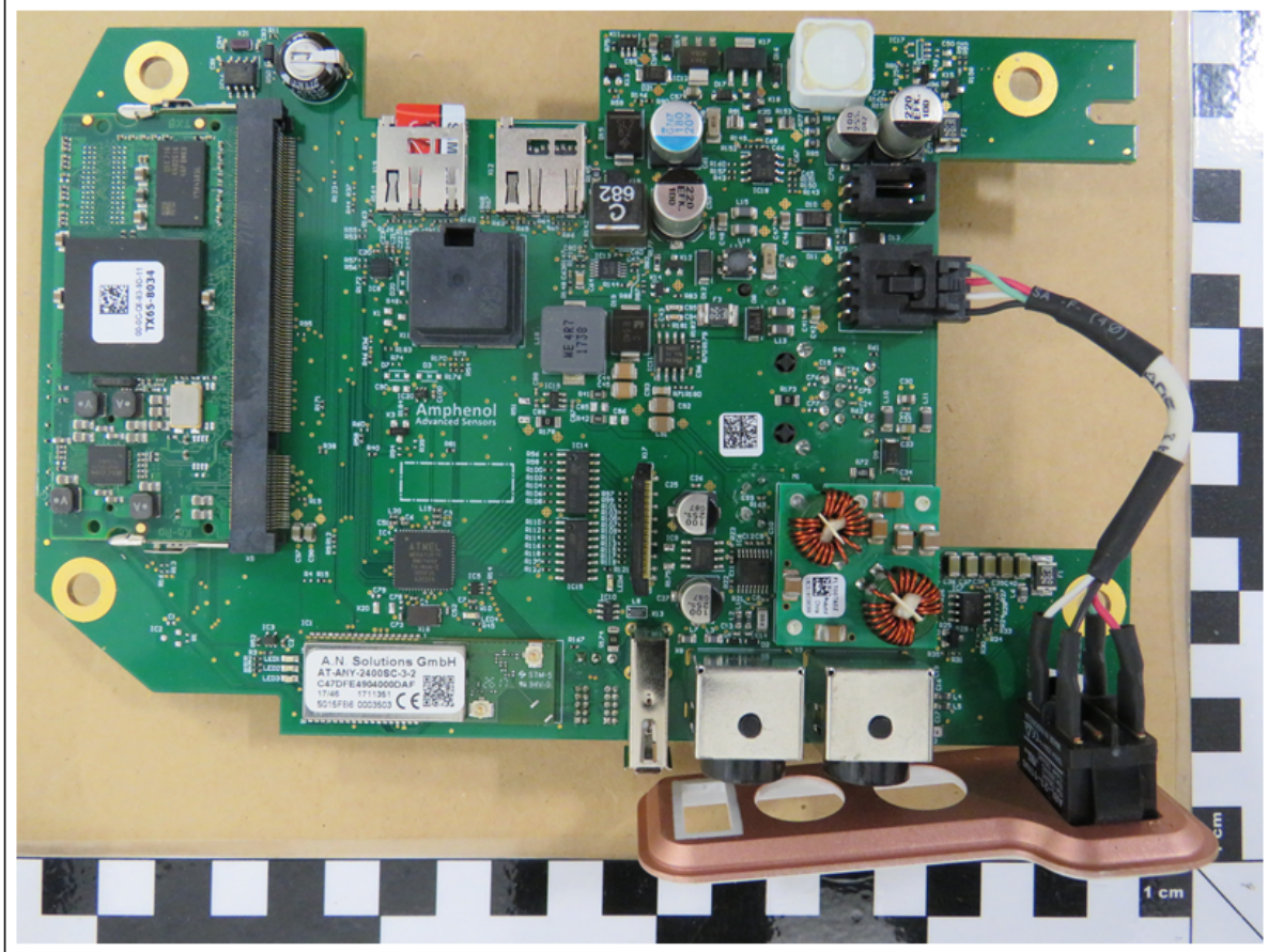
VIEW B.1
