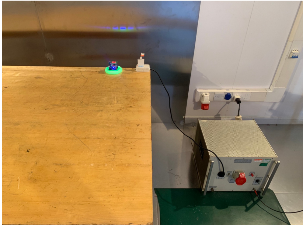
Conducted Emission
