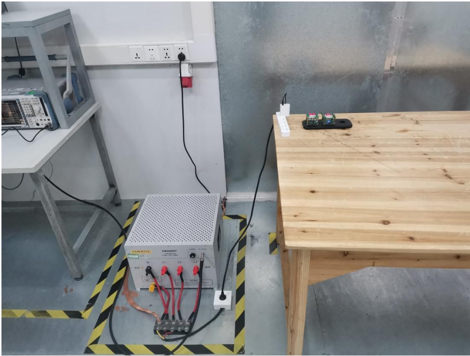
FCC ID: 2AJQ7-IJWC2104 Photo of Conducted Emission Measurement
