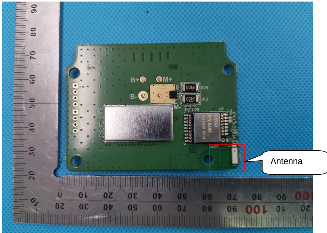
INTERNAL VIEW OF EUT (FIGURE 8)
