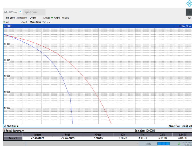
Band13-10MHz-QPSK-23230-50RB#0
