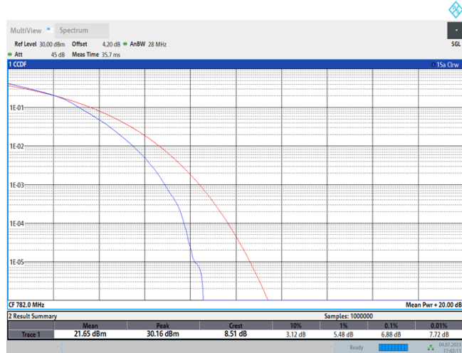
Band13-10MHz-16QAM-23230-27RB#0
