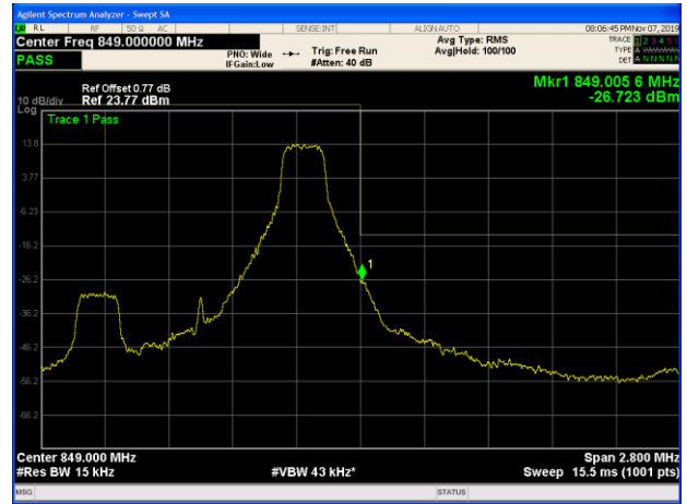
LTE Band 26 QPSK 1.4MHz CH-High 100%RB
