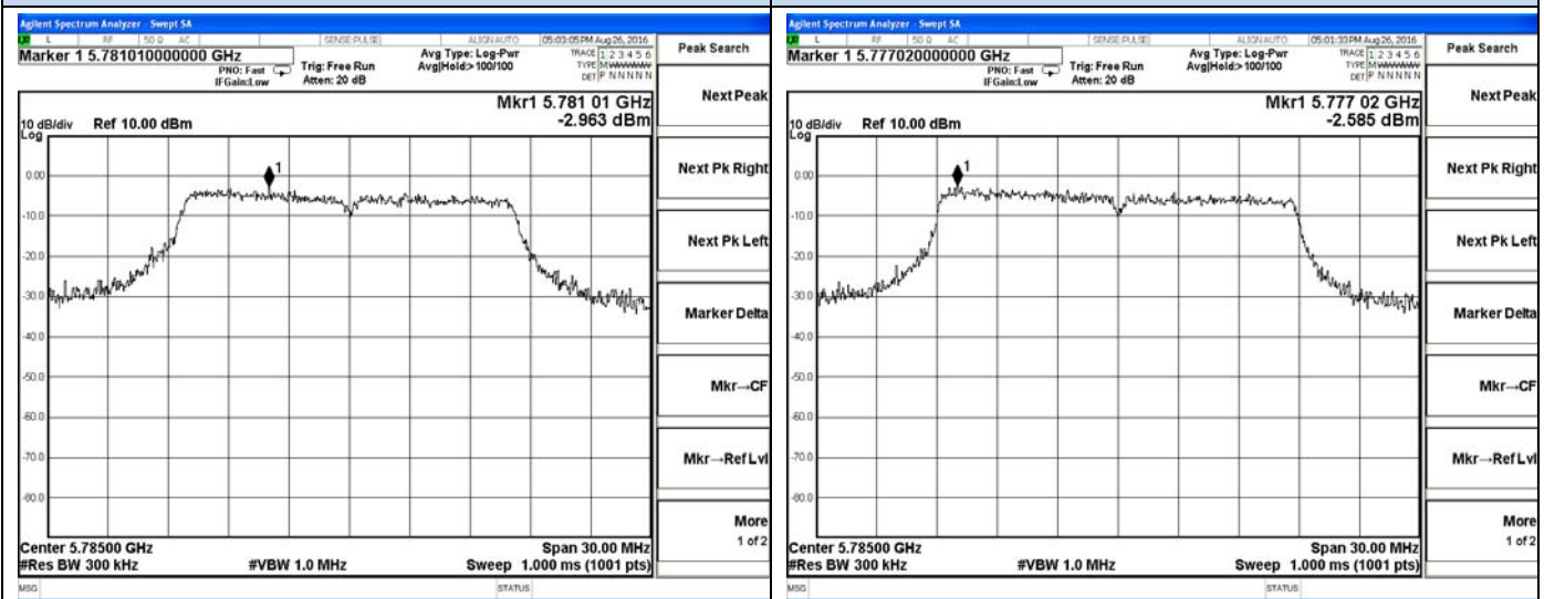
802.11a-5785MHz
