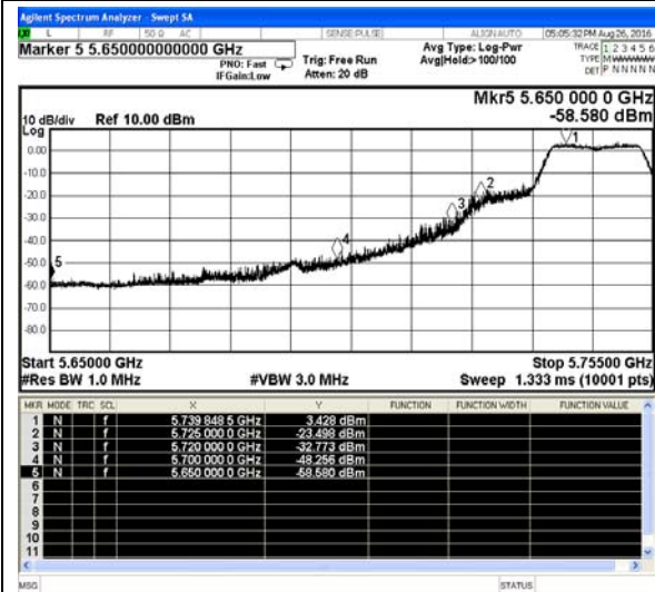
802.11a-Low channel(Peak)
