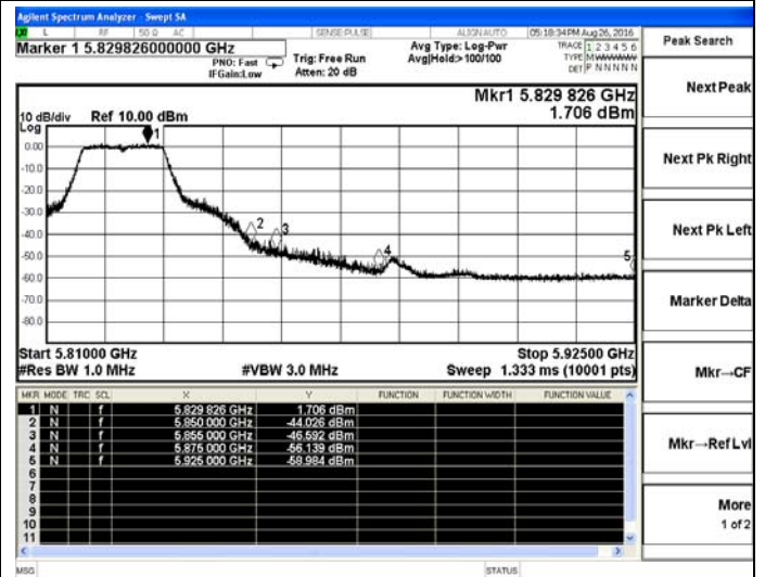
802.11a-High channel(Peak)
