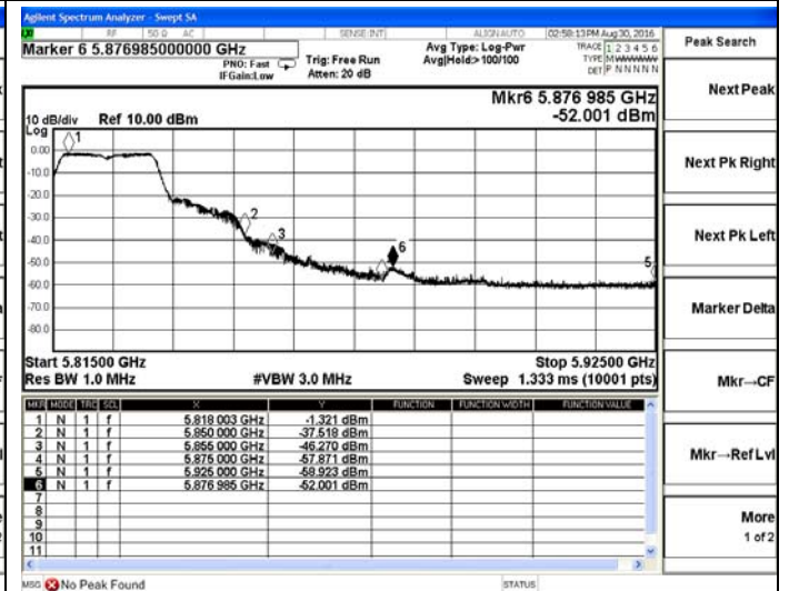
802.11ac20-High channel(Peak)
