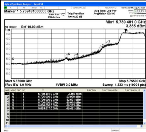
802.11n-HT20-Low channel(Peak)
