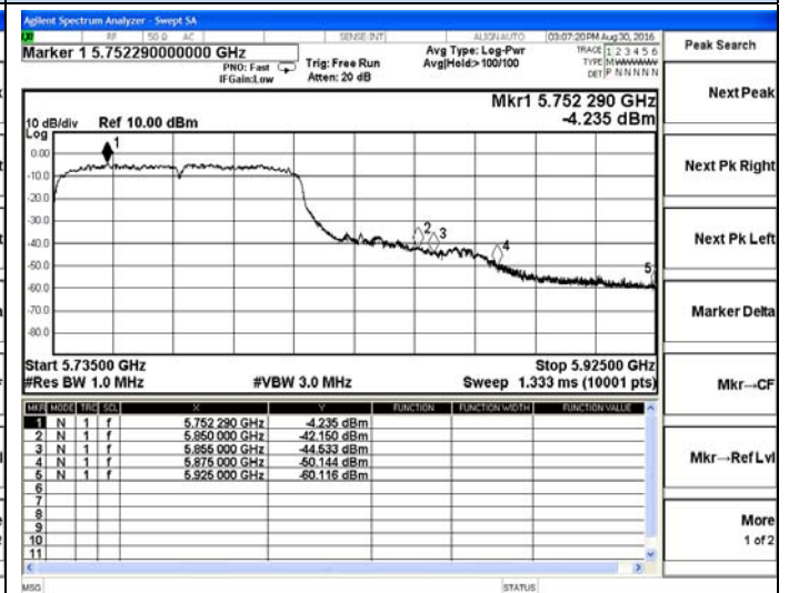
802.11ac80-High channel(Peak)
