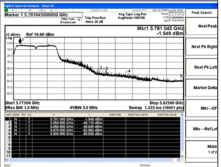
802.11n-HT40-High channel(Peak)
