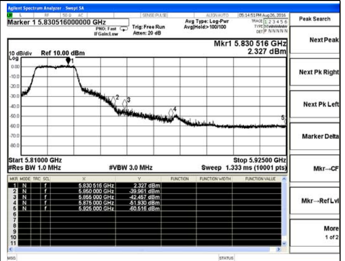
802.11n-HT20-High channel(Peak)
