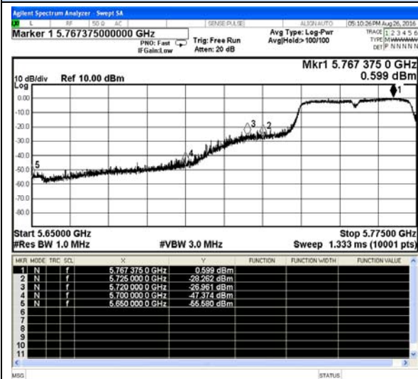
802.11n-HT40-Low channel(Peak)
