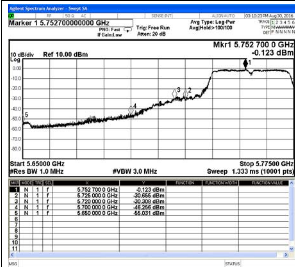
802.11ac40-Low channel(Peak)
