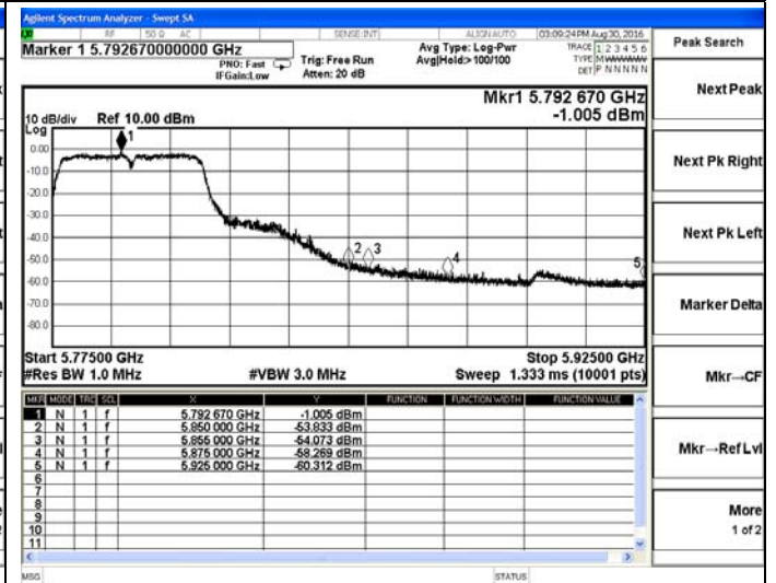
802.11ac40-High channel(Peak)
