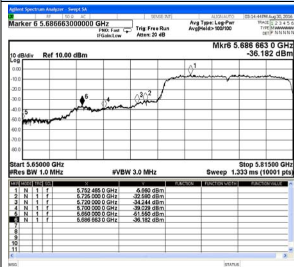
802.11ac80-Low channel(Peak)
