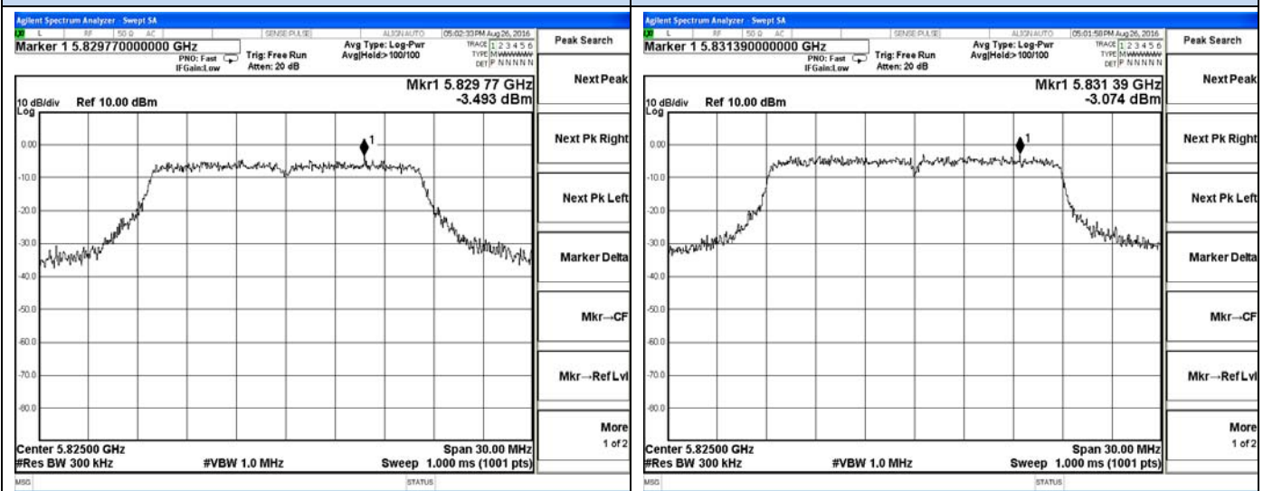
802.11a-5825MHz
