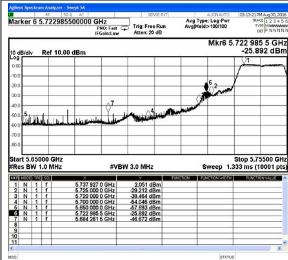
802.11ac20-Low channel(Peak)
