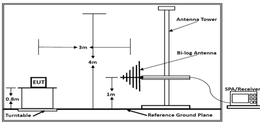
Below 1GHz
