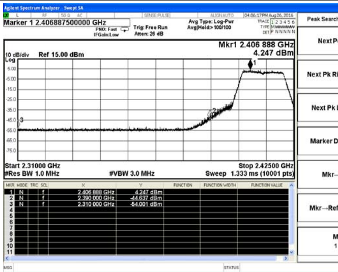
802.11n(HT20)-Low channel(Peak)
