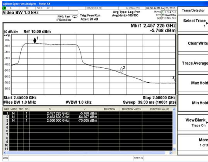
802.11g-High channel(Average)
