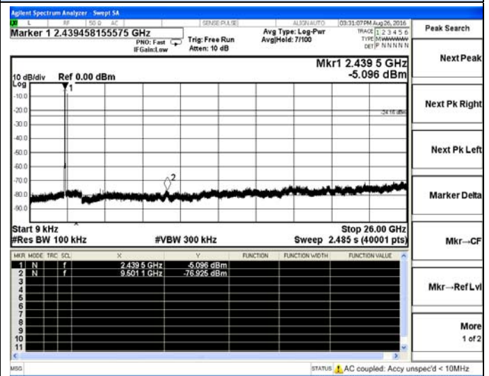
802.11n(HT20)-Middle channel
