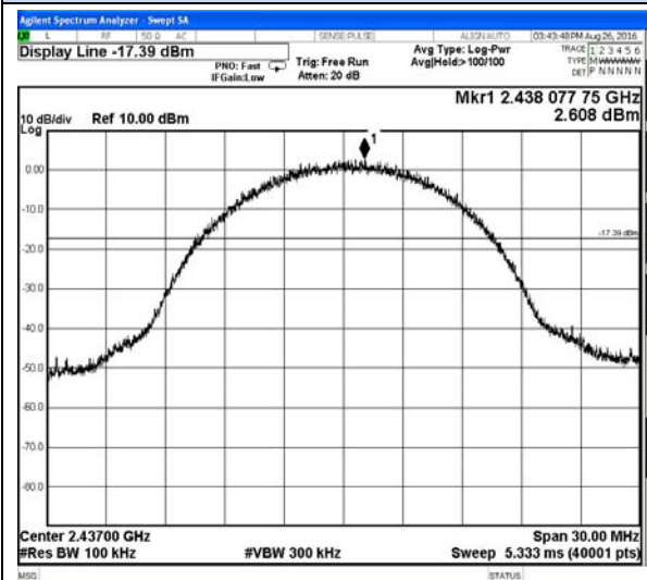
802.11b-Middle channel
