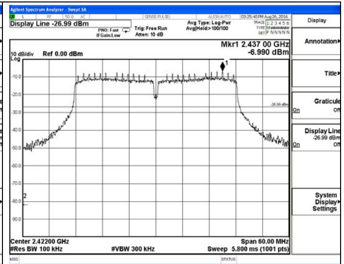
802.11n(HT40)-Low channel
