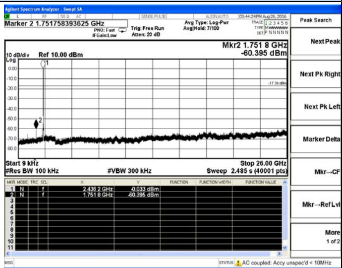
802.11b-Middle channel
