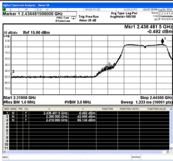
802.11n(HT40)-Low channel(Peak)
