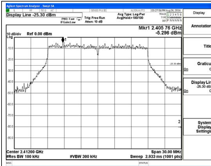
802.11n(HT20)-Low channel
