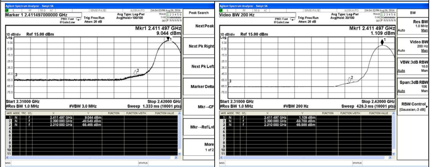
802.11b-Low channel(Peak)
