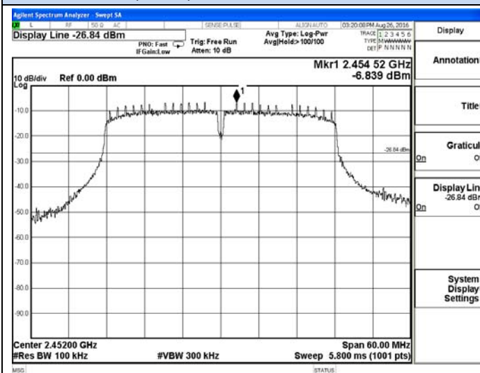
802.11n(HT40)-High channel Reference
