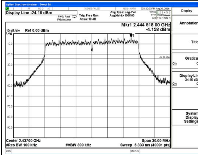
802.11n(HT20)-Middle channel
