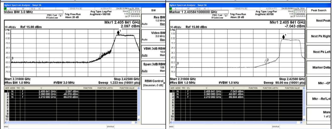
802.11g-Low channel(Peak)
