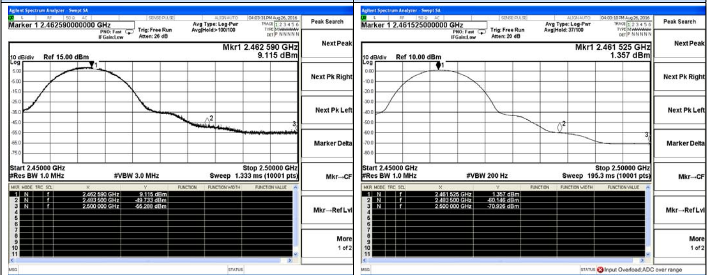
802.11b-High channel(Peak)
