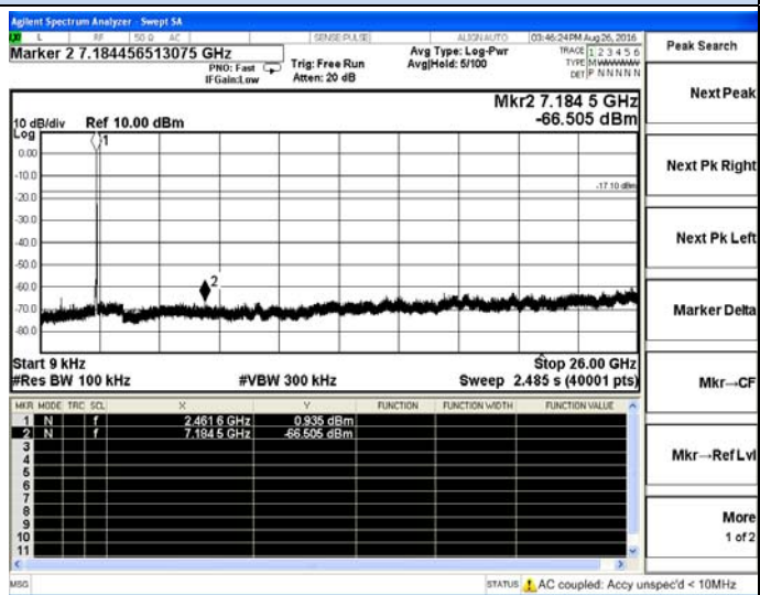
802.11b-High channel
