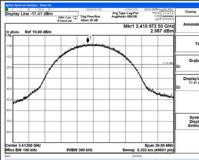
802.11b-Low channel Reference
