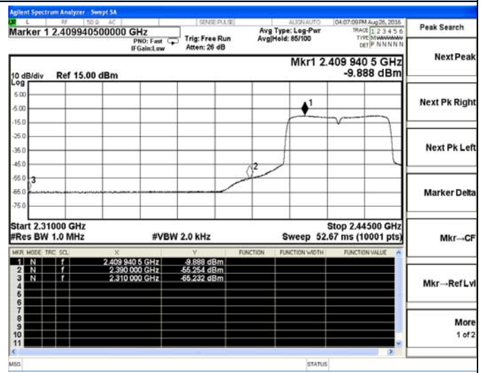
802.11n(HT40)-Low channel(Average)
