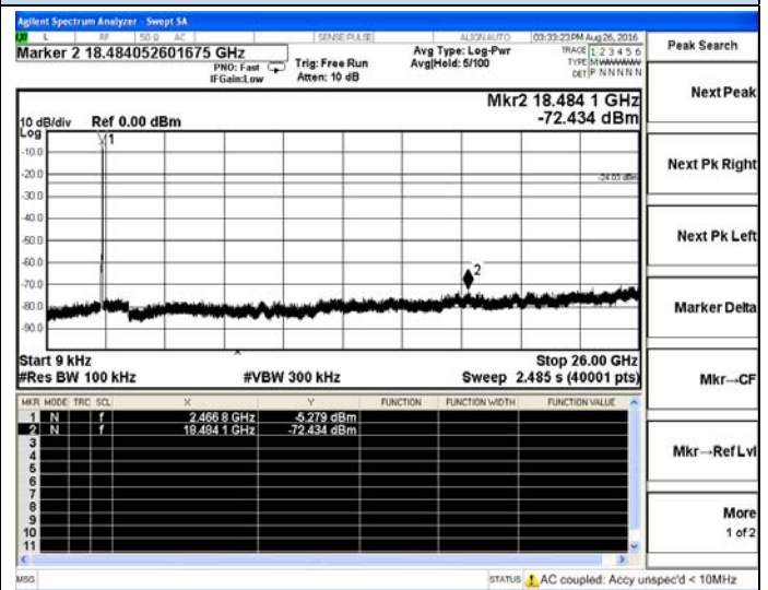
802.11n(HT20)-High channel
