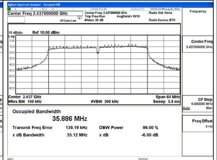
802.11n(HT40)-Middle channel
