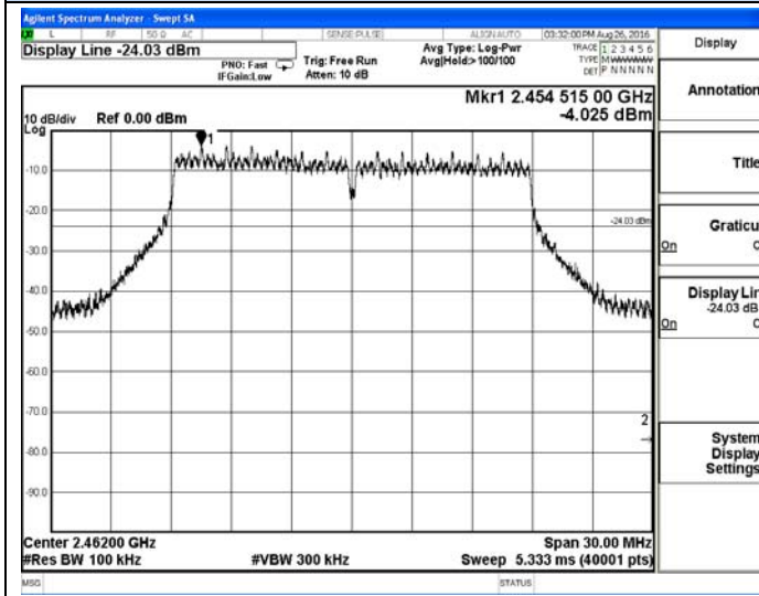
802.11n(HT20)-High channel
