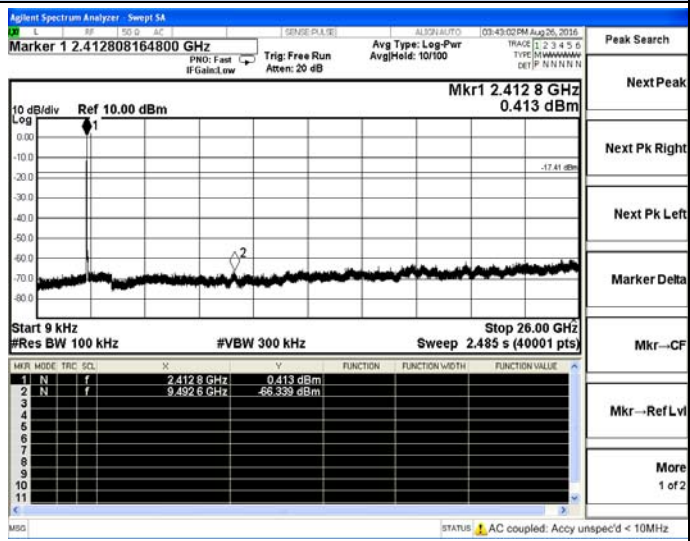
802.11b-Low channel
