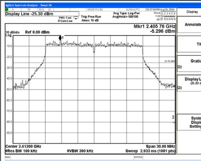
802.11n(HT20)-Low channel Reference
