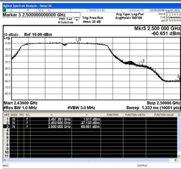
802.11n(HT40)-High channel(Peak)
