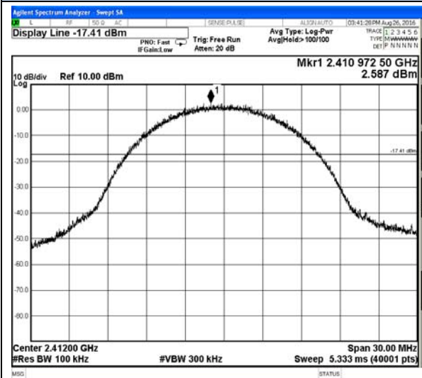
802.11b-Low channel
