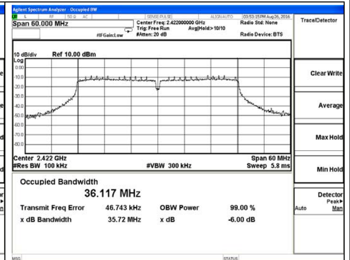
802.11n(HT40)-Low channel
