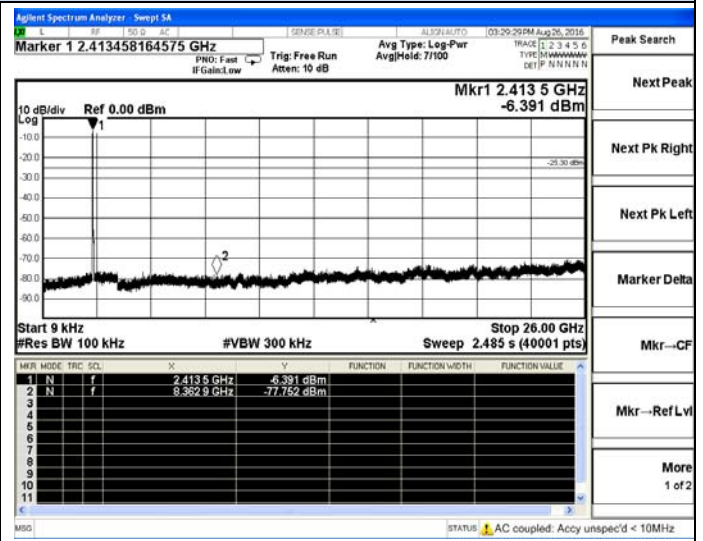
802.11n(HT20)-Low channel
