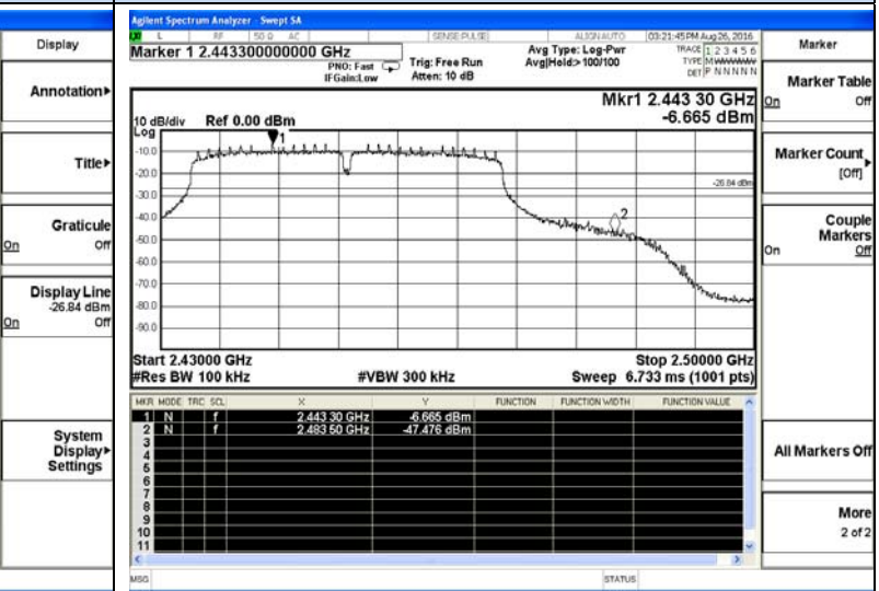
802.11n(HT40)-High channel
