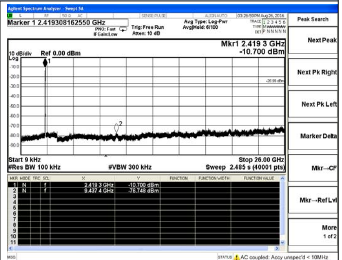
802.11n(HT40)-Low channel
