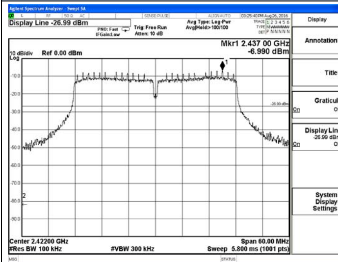
802.11n(HT40)-Low channel Reference
