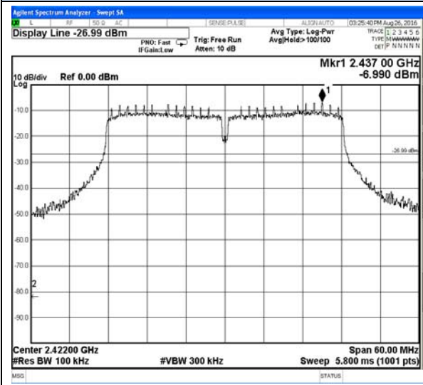
802.11n(HT40)-Low channel Reference
