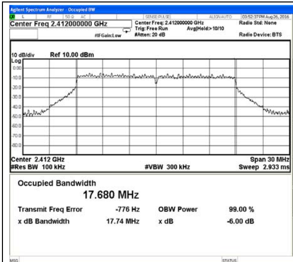
802.11n(HT20)-Low channel
