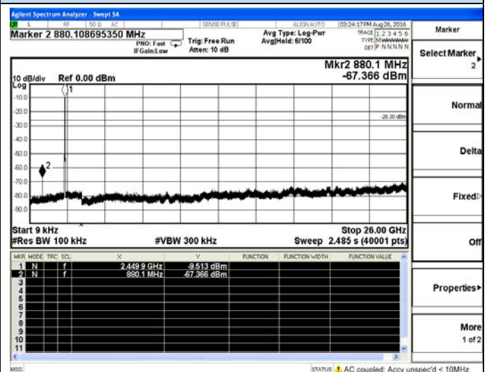
802.11n(HT40)-Middle channel
