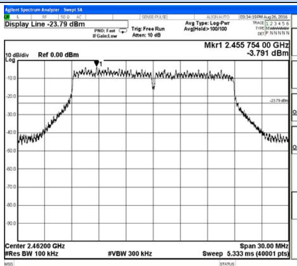
802.11g-High channel
