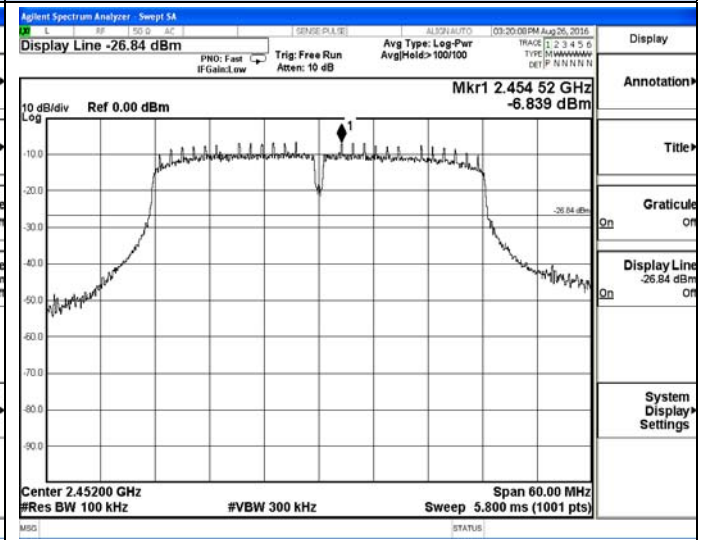
802.11n(HT40)-High channel
