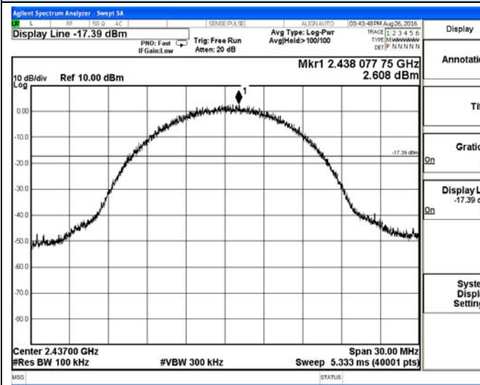
802.11b-Middle Run channel Reference
