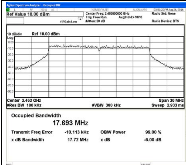
802.11n(HT20)-High channel
