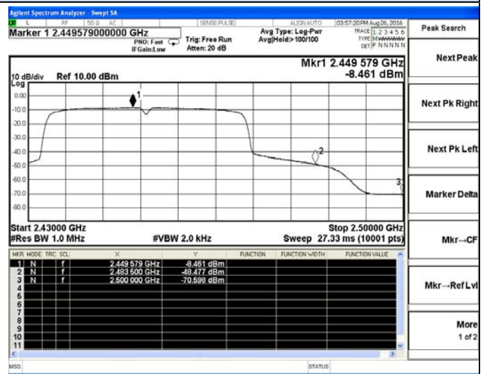
802.11n(HT40)-High channel(Average)
