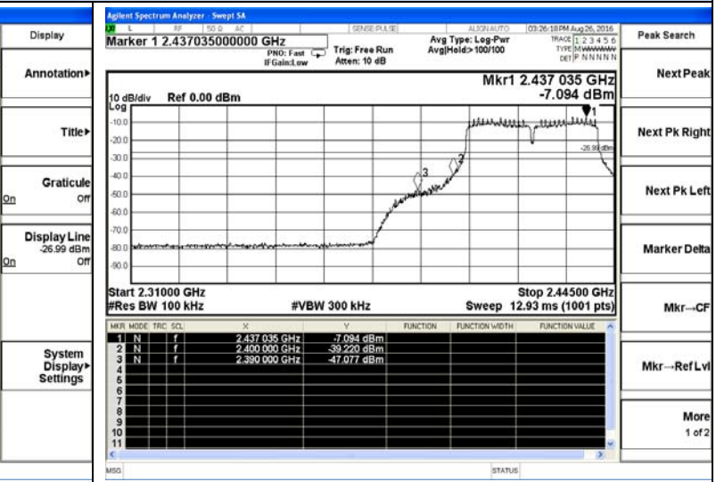
802.11n(HT40)-Low channel
