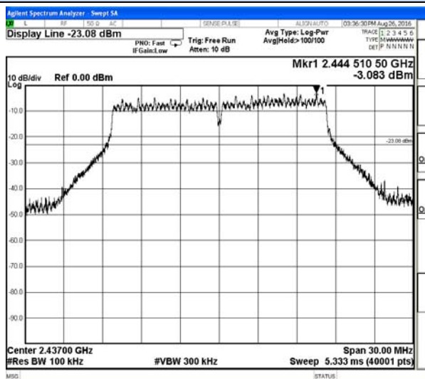
802.11g-Middle channel
