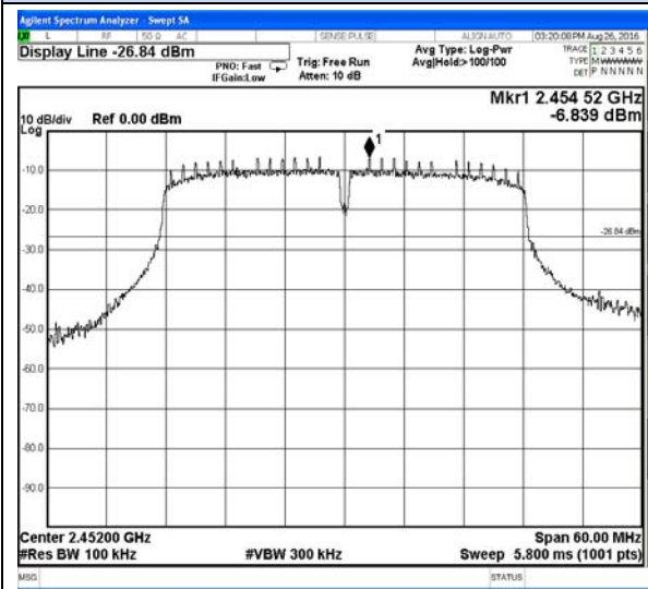
802.11n(HT40)-High channel Reference
