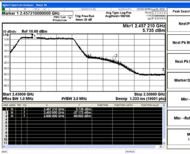
802.11n(HT20)-High channel(Peak)
