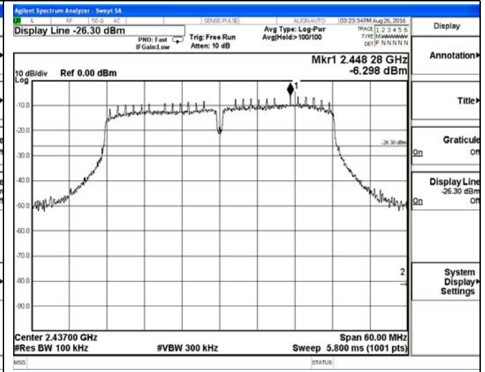
802.11n(HT40)-Middle channel
