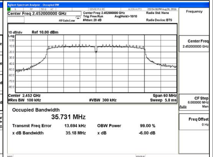
802.11n(HT40)-High channel
