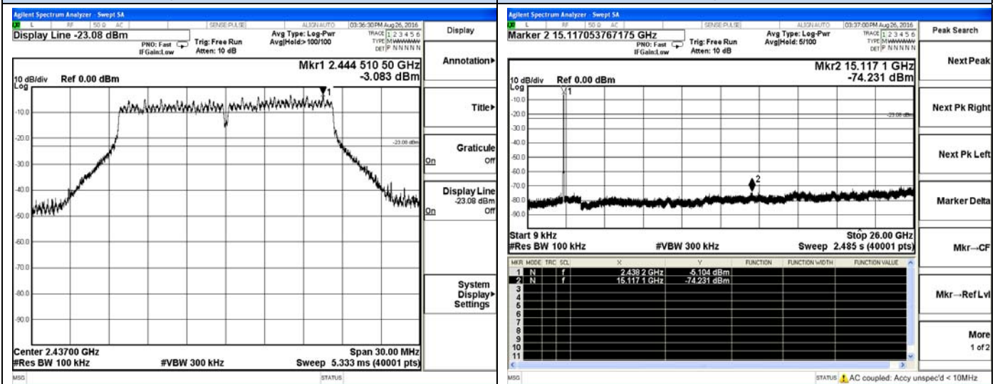
802.11g-Middle Run channel Reference
