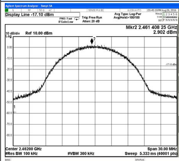
802.11b-High channel
