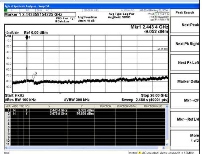
802.11n(HT40)-High channel
