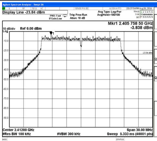
802.11g-Low channel
