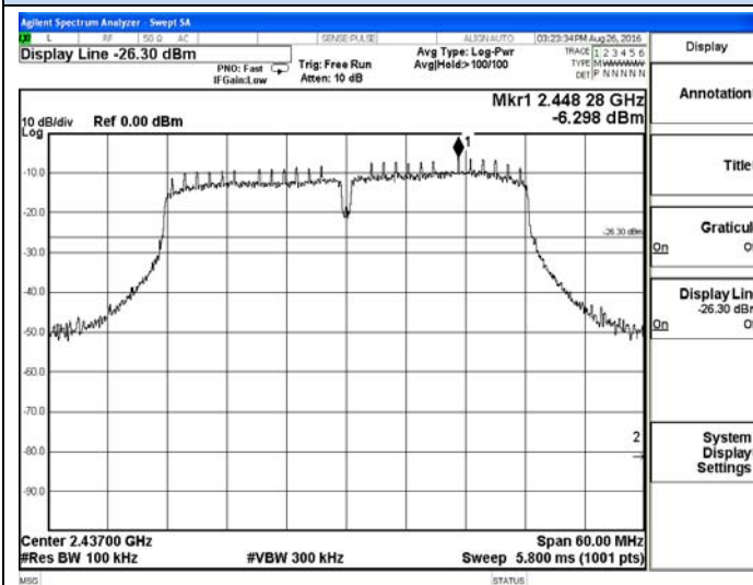
802.11n(HT40)-Middle channel Reference
