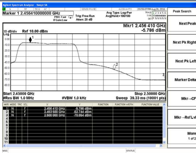
802.11n(HT20)-High channel(Average)
