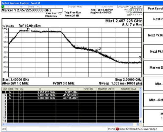
802.11g-High channel(Peak)
