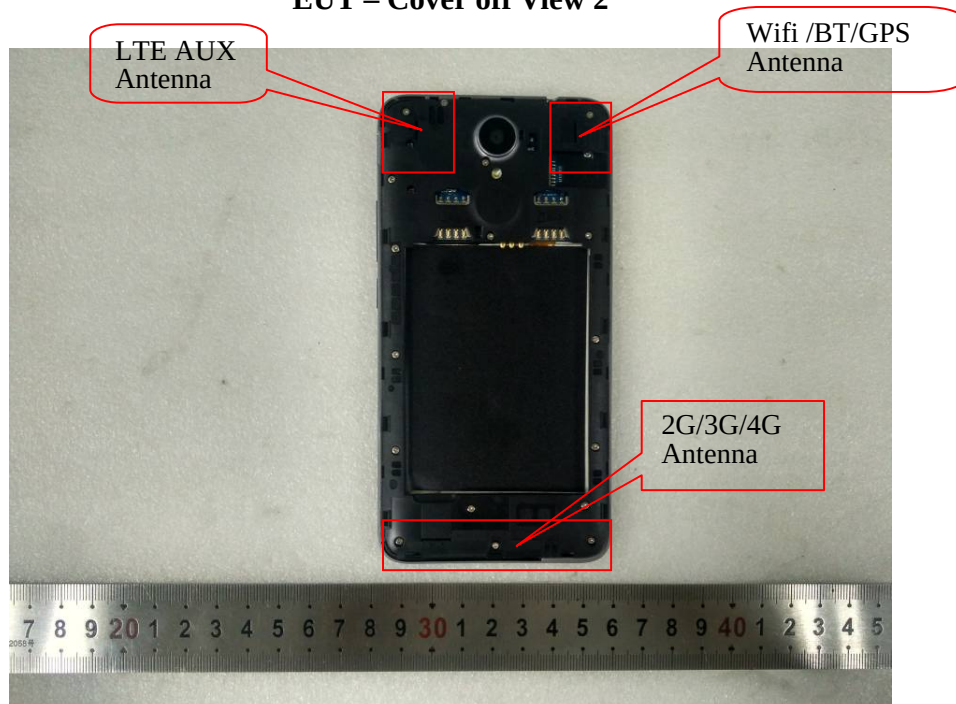
EUT – Cover off View 2
