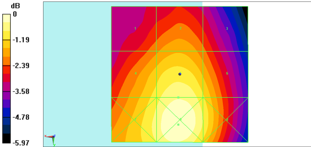
Fig B.5 HAC RF E-Field WIFI2.4G
