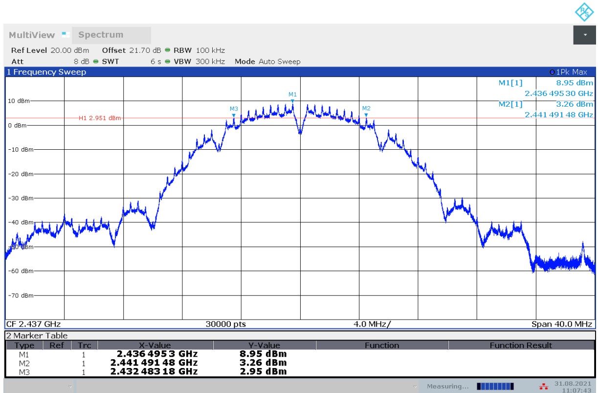
Fig.A.4.2 Occupied 6dB Bandwidth (802.11b, Ch 6)
