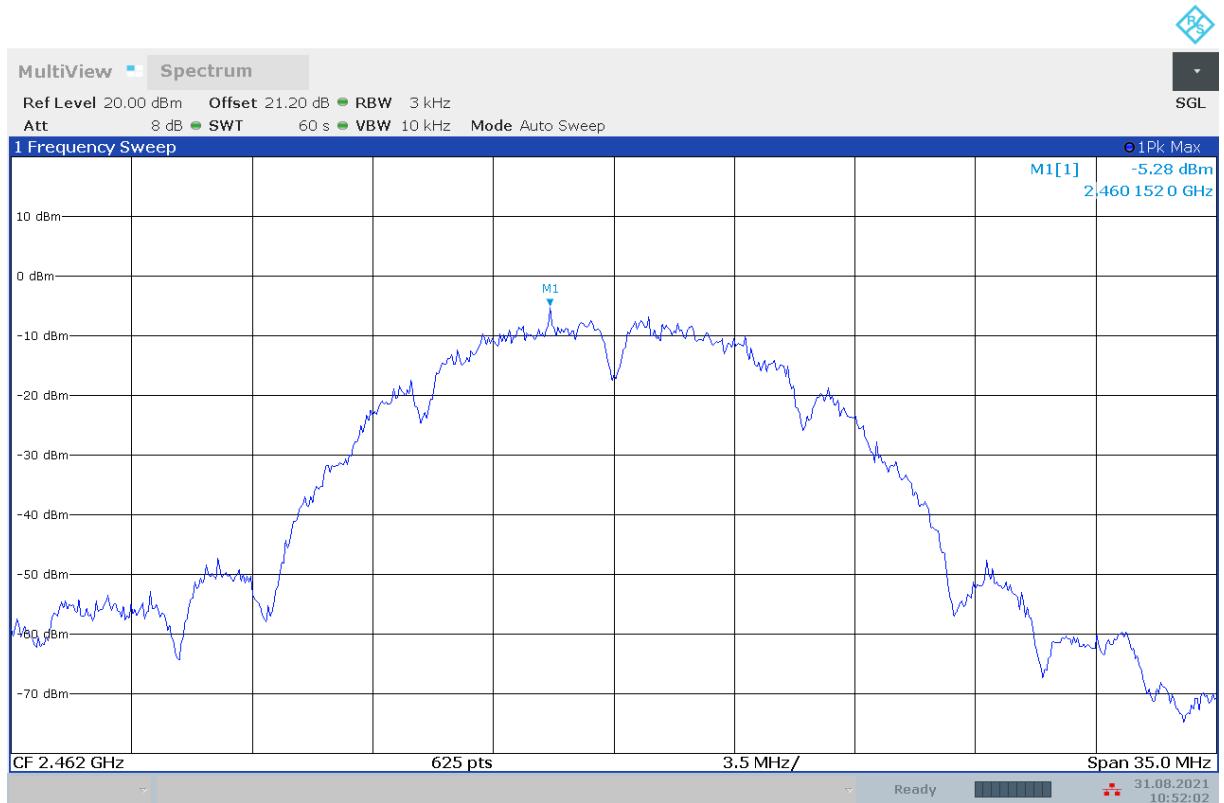
Fig.A.3.3 Power Spectral Density (802.11b, Ch 11)
