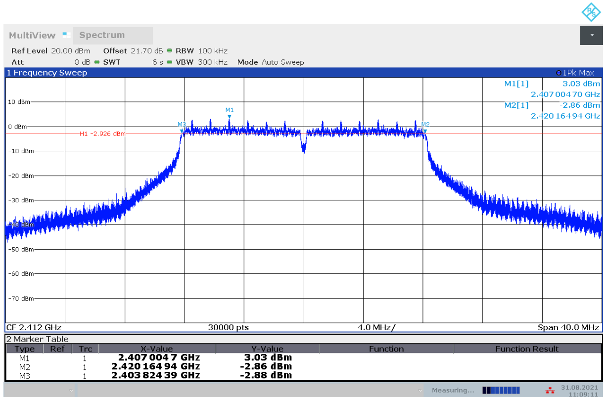
Fig.A.4.4 Occupied 6dB Bandwidth (802.11g, Ch 1)
