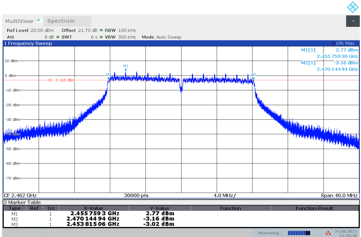
Fig.A.4.6 Occupied 6dB Bandwidth (802.11g, Ch 11)
