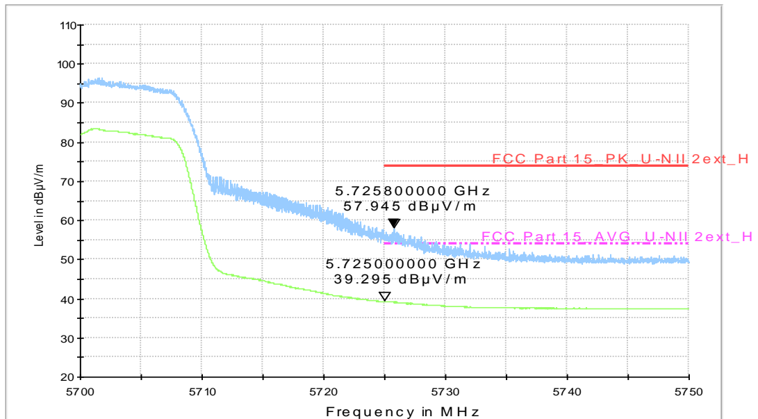
RE - Power-5.7GHz-5.75GHz
