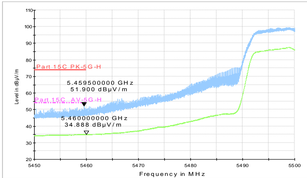
RE - Power-5.45GHz-5.50GHz
