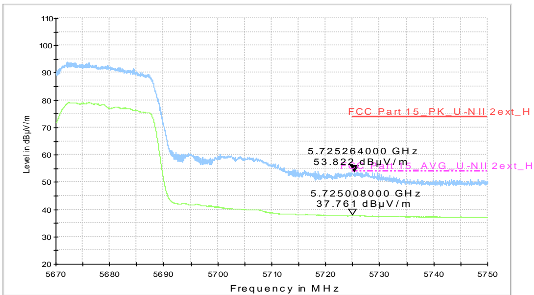
RE - Power-5.7GHz-5.75GHz
