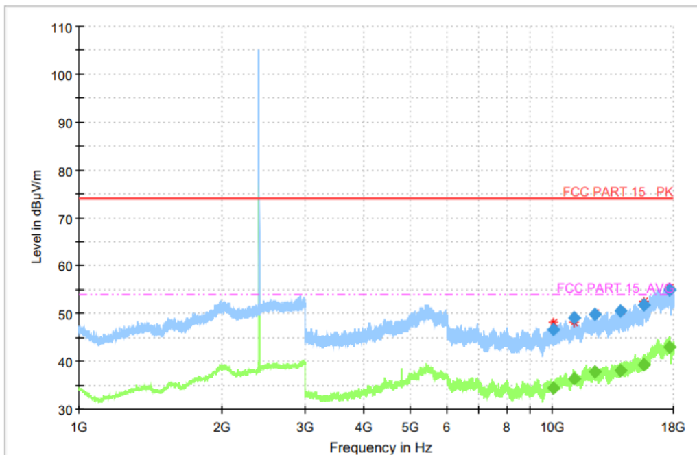
Fig. 38 Radiated Spurious Emission ( \pi/4 DQPSK, Ch0, 1GHz ~ 18GHz)
