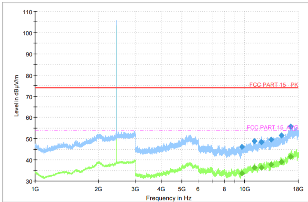
Fig. 44 Radiated Spurious Emission (8DPSK, Ch39, 1GHz ~ 18GHz)
