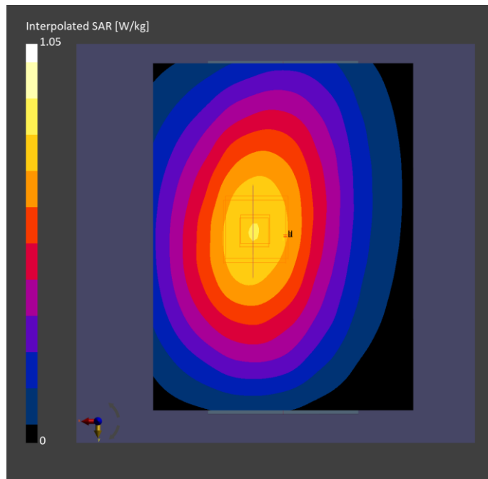
Fig.2 GSM 850 Body
