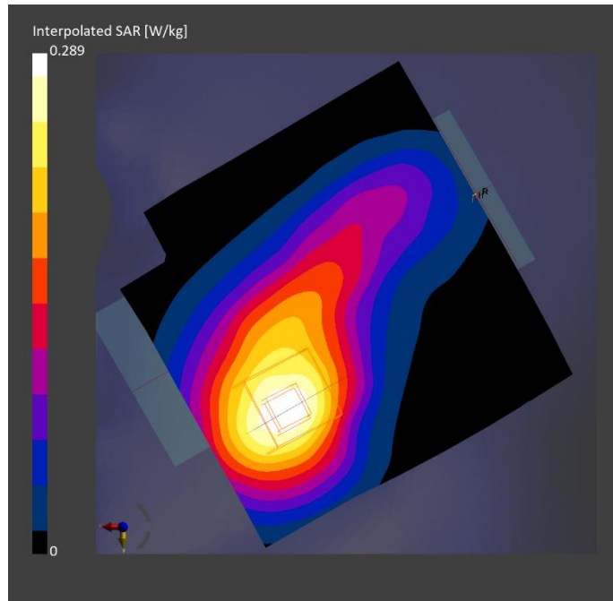
Fig.3 GSM 1900 Head
