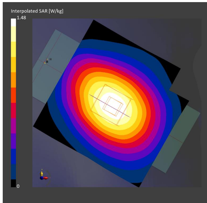
Fig.13 LTE Band 5 Head
