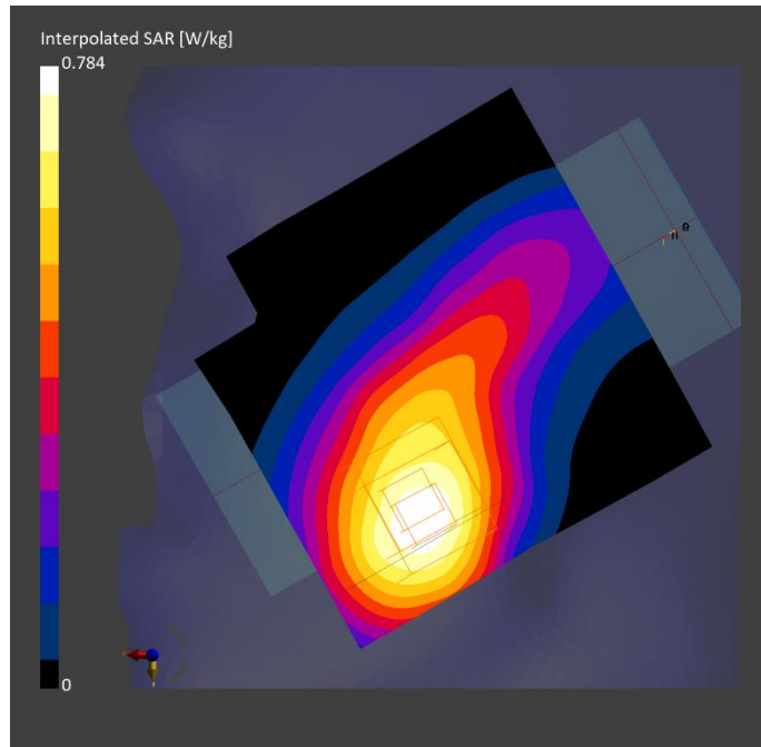
Fig.11 LTE Band 2 Head
