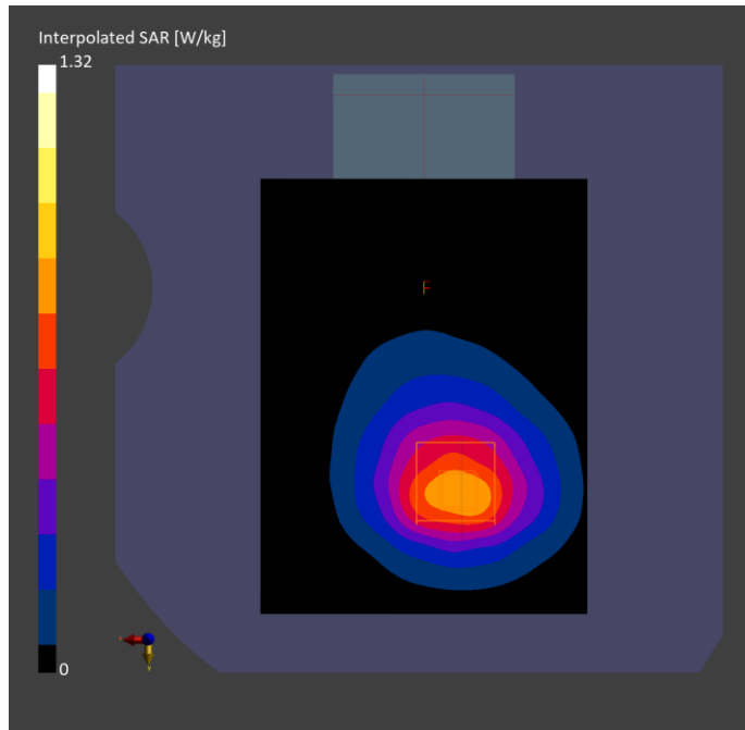
Fig.8 WCDMA Band 4 Body
