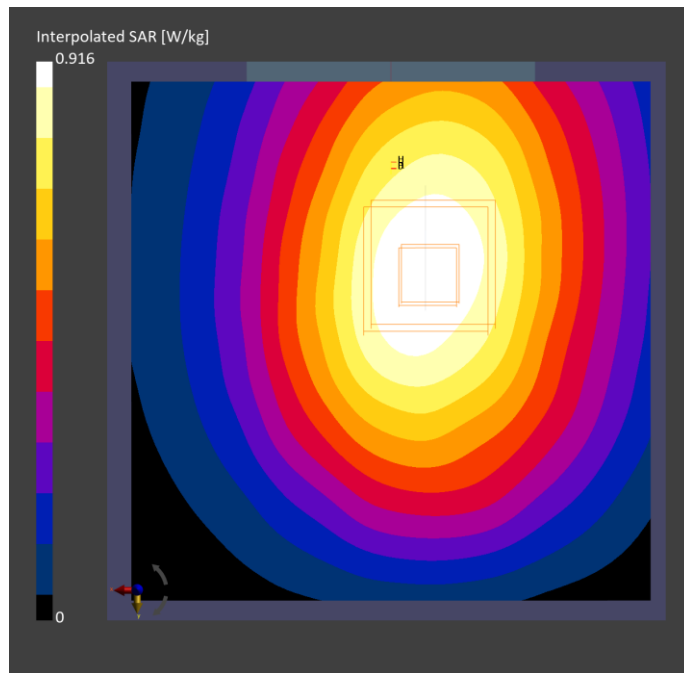
Fig.14 LTE Band 5 Body
