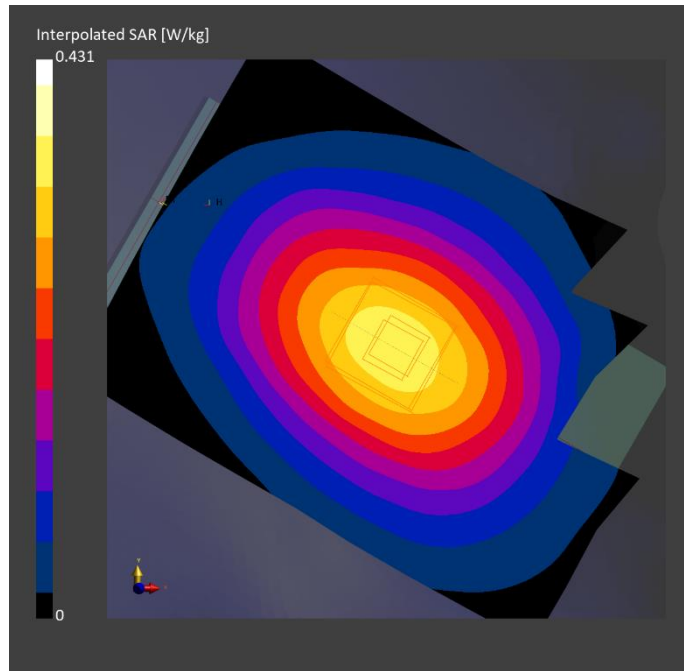
Fig.17 LTE Band 12 Head
