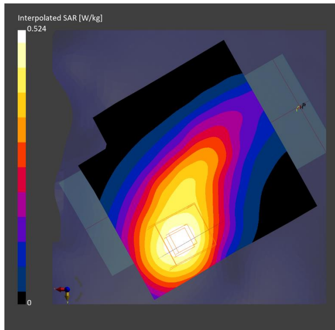
Fig.7 WCDMA Band 4 Head
