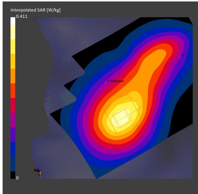
Fig.21 LTE Band 66 Head
