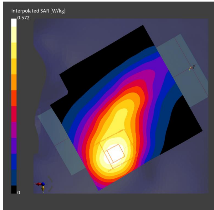
Fig.5 WCDMA Band 2 Head
