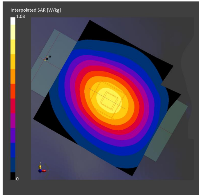
Fig.9 WCDMA Band 5 Head
