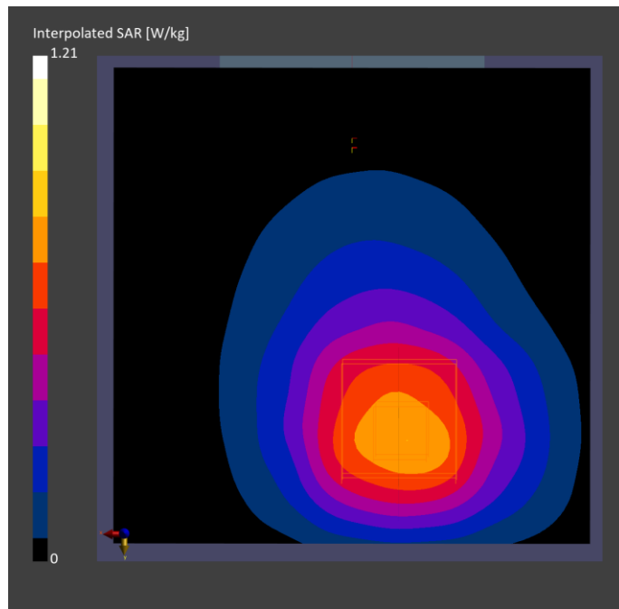
Fig.22 LTE Band 66 Body
