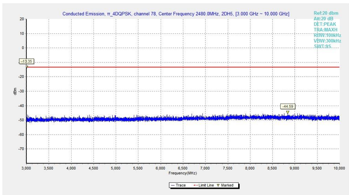
Fig. 24 Conducted Spurious Emission ( \pi/4 DQPSK, Ch78, 3GHz-10GHz)
