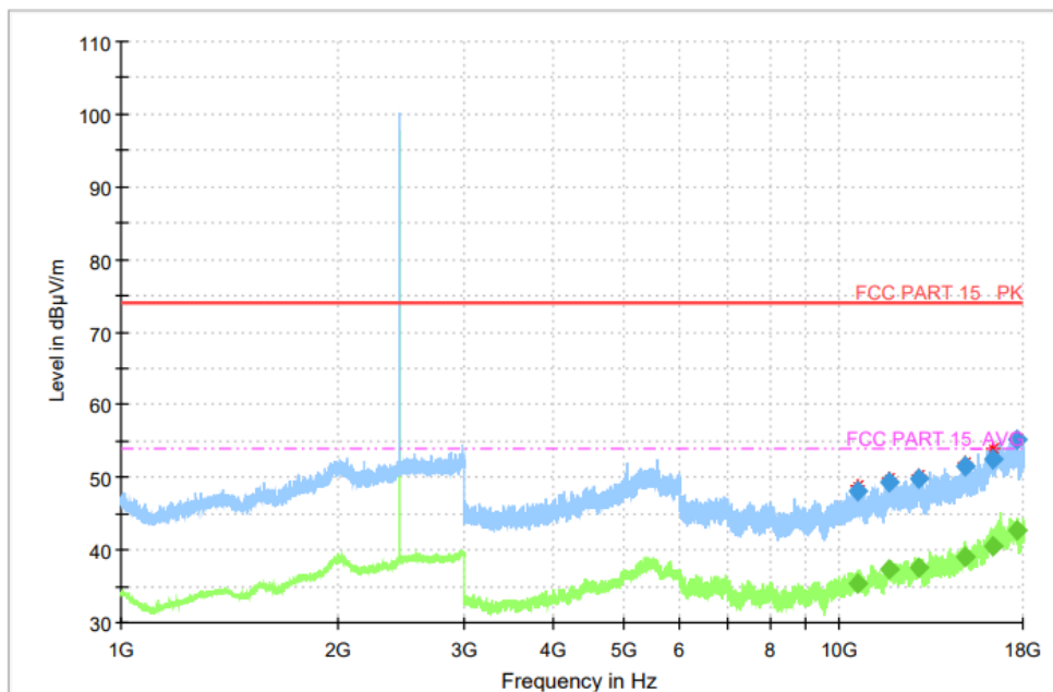
Fig. 44 Radiated Spurious Emission (8DPSK, Ch39, 1GHz ~ 18GHz)
