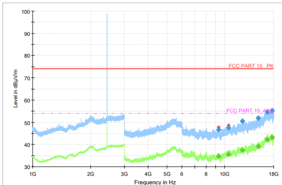
Fig. 34 Radiated Spurious Emission (GFSK, Ch39, 1GHz ~ 18GHz)
