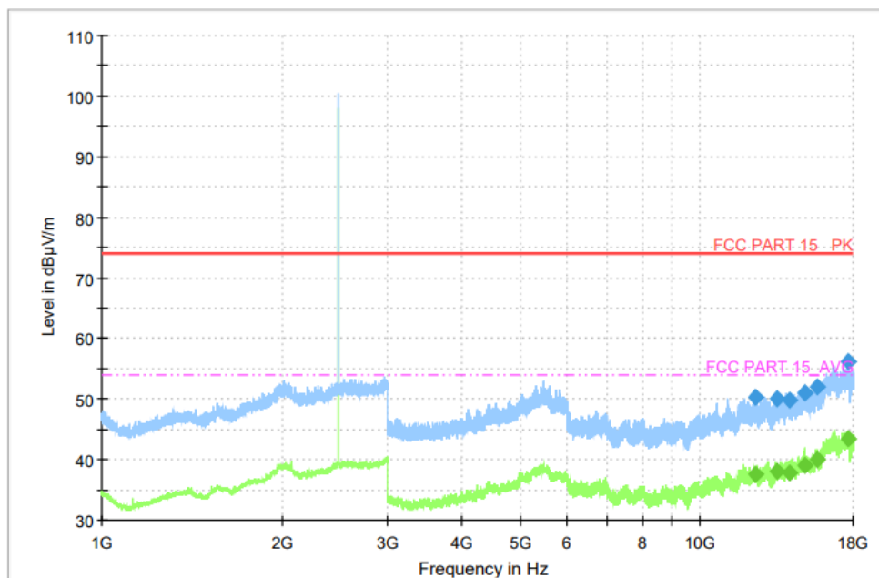
Fig. 35 Radiated Spurious Emission (GFSK, Ch78, 1GHz ~ 18GHz)
