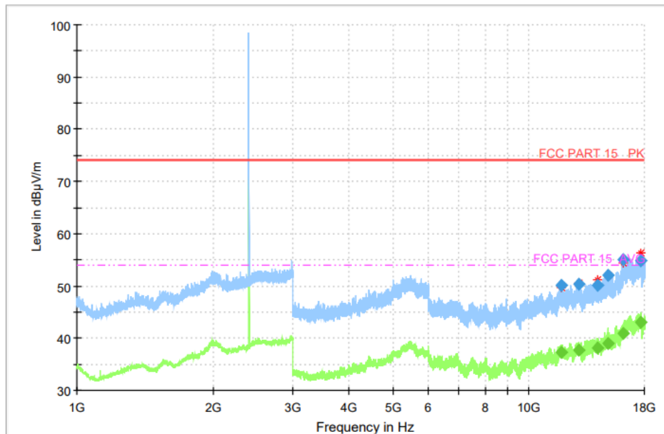
Fig. 43 Radiated Spurious Emission (8DPSK, Ch0, 1GHz ~ 18GHz)
