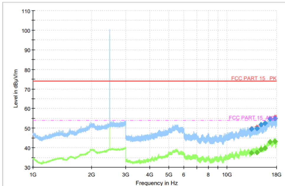
Fig. 45 Radiated Spurious Emission (8DPSK, Ch78, 1GHz ~ 18GHz)
