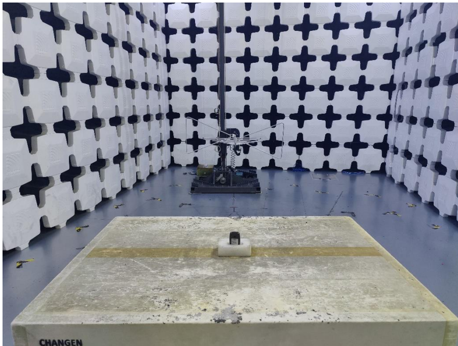
8. Radiated Emissions (Part 15C, 30MHz-1GHz)
