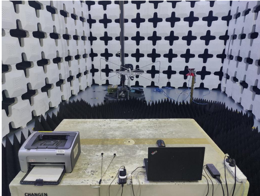
5. Radiated Emissions (Part 15B Data transfer, 1GHz-18GHz)
