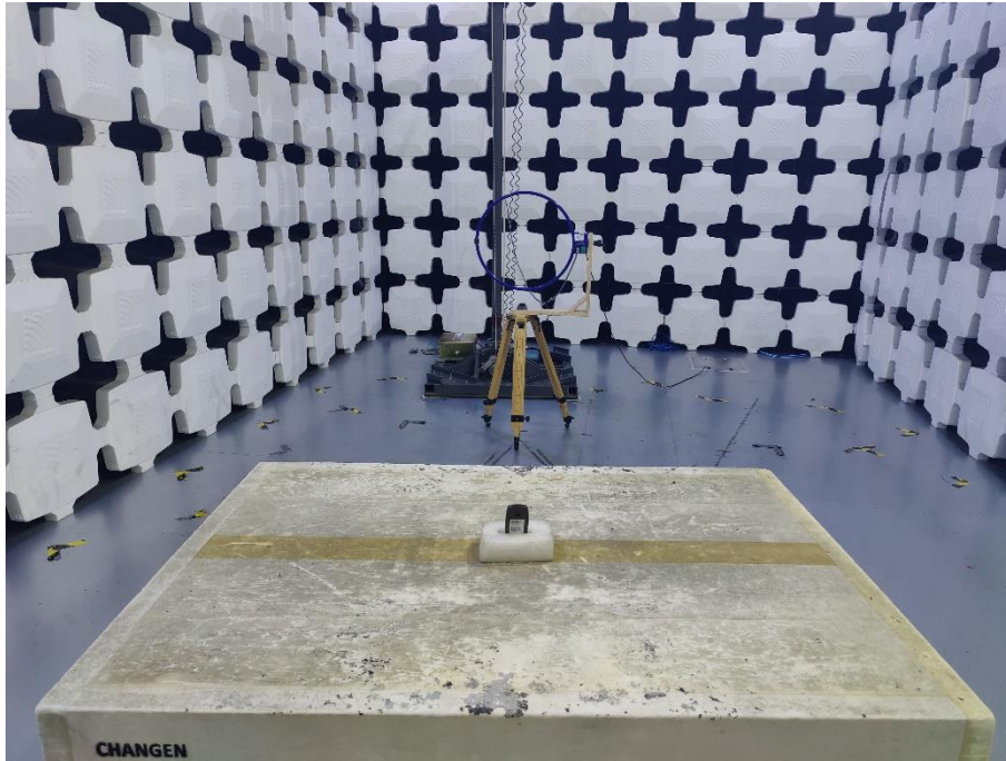
7. Radiated Emissions (Part 15C, 9kHz-30MHz)
