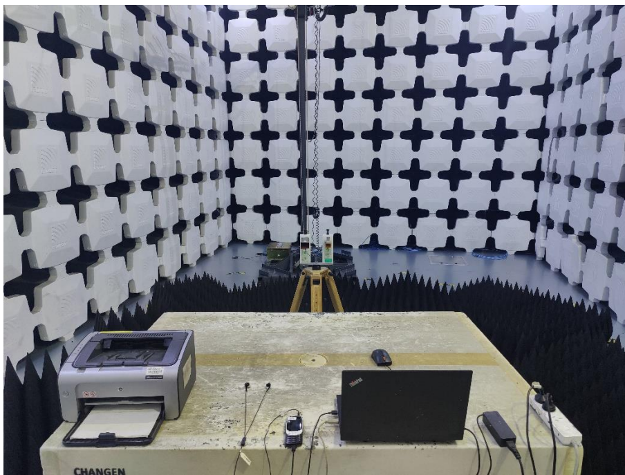
6. Radiated Emissions (Part 15B Data transfer, 18GHz-26.5GHz)
