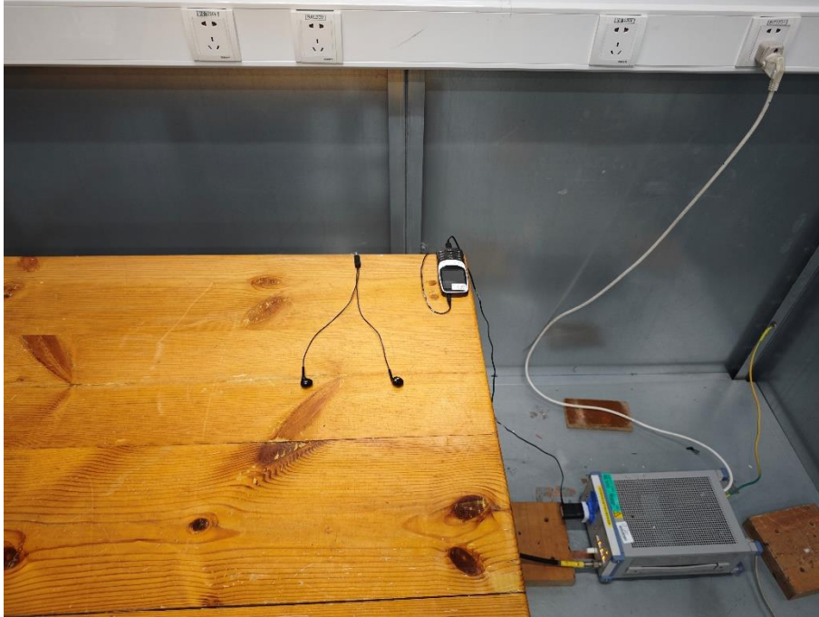
13. Conducted Emission (Part 15B, GSM receiver/WCDMA receiver /LTE receiver/Video Player/FM receiver/Camera)
