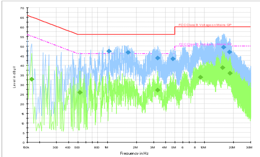
Fig.B.8.1 AC Powerline Conducted Emission-blutetooth
