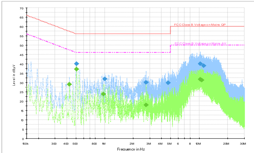
Fig.B.10.1 AC Powerline Conducted Emission-blutetooth
