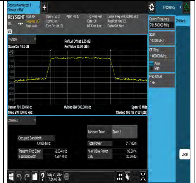
Band12-5MHz-16QAM-23035-25RB#0-PASS
