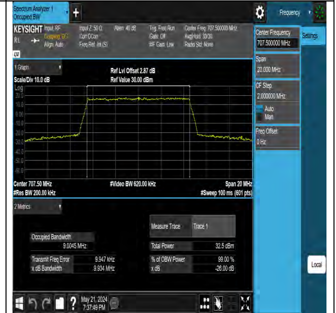
Band12-10MHz-QPSK-23095-50RB#0-PASS
