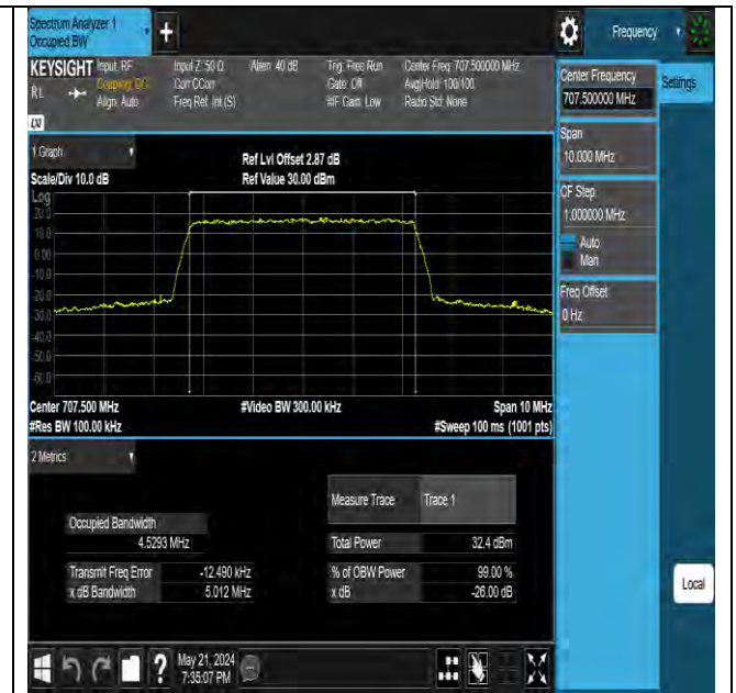
Band12-5MHz-QPSK-23095-25RB#0-PASS
