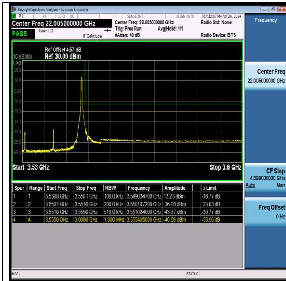
NTNV-N78-3450-3550-PC2-30-20-H-DFT-QPSK-Edge_1RB_Right-Ant6-PASS
