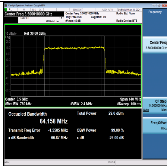
NTNV-N78-3450-3550-PC2-30-70-M-DFT-256QA M-Outer_Full-Ant6-PASS
