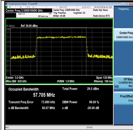
NTNV-N78-3450-3550-PC2-30-60-M-DFT-16QAM -Outer_Full-Ant6-PASS
