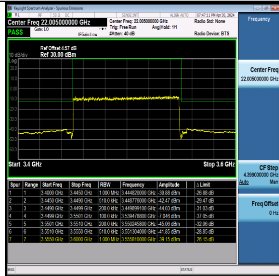
NTNV-N78-3450-3550-PC2-30-100-H-DFT-QPSK-Outer_Full-Ant6-PASS
