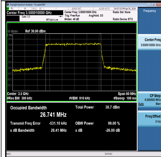
NTNV-N78-3450-3550-PC2-30-30-M-DFT-QPSK-Outer_Full-Ant6-PASS
