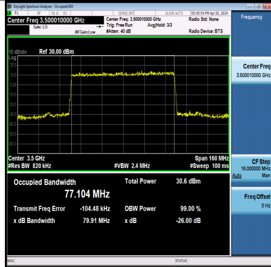
NTNV-N78-3450-3550-PC2-30-80-M-DFT-QPSK- Outer_Full-Ant6-PASS
