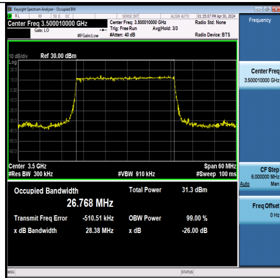
NTNV-N78-3450-3550-PC2-30-30-M-DFT-PI2BPS K-Outer_Full-Ant6-PASS
