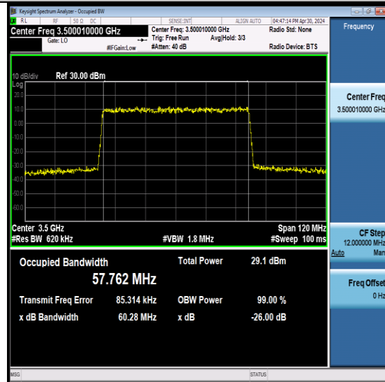
NTNV-N78-3450-3550-PC2-30-60-M-DFT-64QAM -Outer_Full-Ant6-PASS
