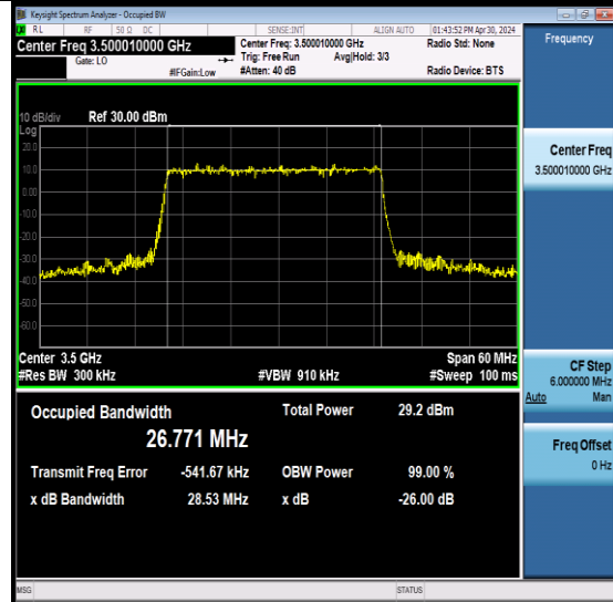
NTNV-N78-3450-3550-PC2-30-30-M-DFT-64QAM -Outer_Full-Ant6-PASS
