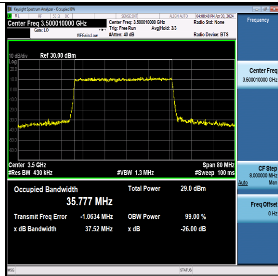
NTNV-N78-3450-3550-PC2-30-40-M-DFT-64QAM -Outer_Full-Ant6-PASS
