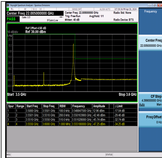
NTNV-N78-3450-3550-PC2-30-50-H-DFT-QPSK-Edge_1RB_Right-Ant6-PASS
