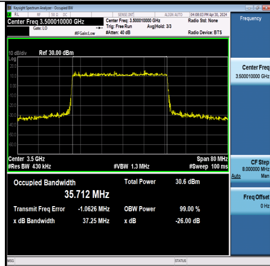
NTNV-N78-3450-3550-PC2-30-40-M-DFT-QPSK-Outer_Full-Ant6-PASS
