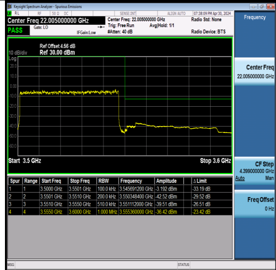
NTNV-N78-3450-3550-PC2-30-50-H-DFT-QPSK-Outer_Full-Ant6-PASS
