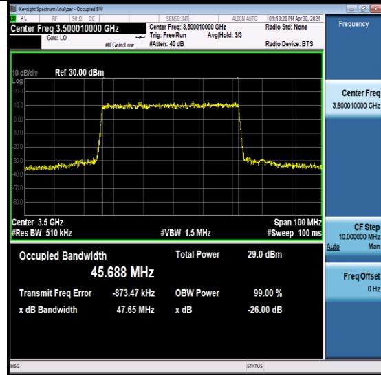
NTNV-N78-3450-3550-PC2-30-50-M-DFT-256QAM M-Outer_Full-Ant6-PASS
