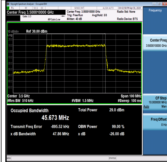
NTNV-N78-3450-3550-PC2-30-50-M-DFT-64QAM-Outer_Full-Ant6-PASS
