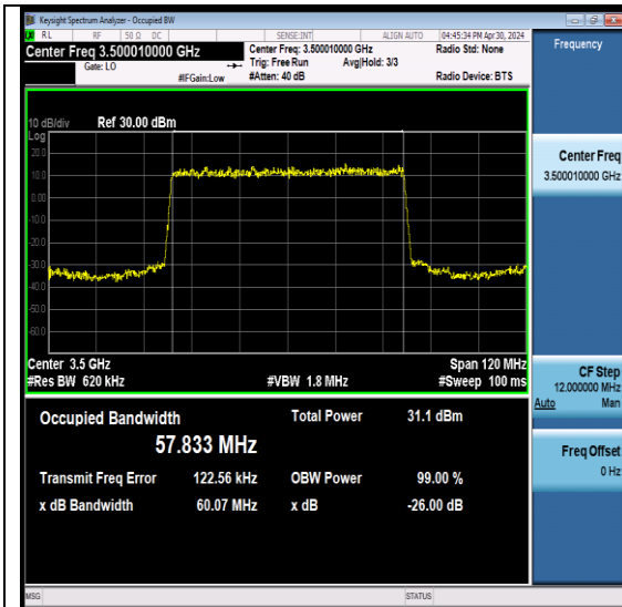
NTNV-N78-3450-3550-PC2-30-60-M-DFT-PI2BPS K-Outer_Full-Ant6-PASS
