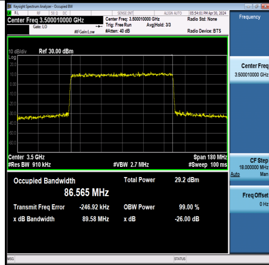
NTNV-N78-3450-3550-PC2-30-90-M-DFT-256QAM-M-Outer_Full-Ant6-PASS
