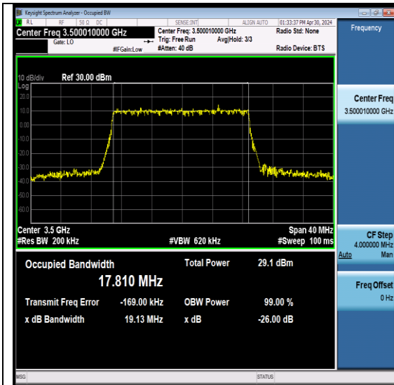
NTNV-N78-3450-3550-PC2-30-20-M-DFT-256QA M-Outer_Full-Ant6-PASS
