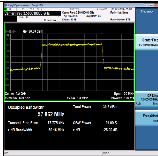
NTNV-N78-3450-3550-PC2-30-60-M-DFT-QPSK- Outer_Full-Ant6-PASS
