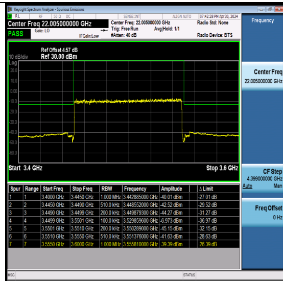
NTNV-N78-3450-3550-PC2-30-100-L-DFT-QPSK-Outer_Full-Ant6-PASS
