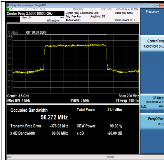
NTNV-N78-3450-3550-PC2-30-100-M-DFT-PI2BP SK-Outter_Full-Ant6-PASS
