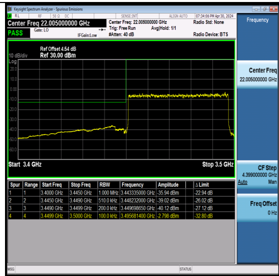
NTNV-N78-3450-3550-PC2-30-50-L-DFT-QPSK-Outer_Full-Ant6-PASS
