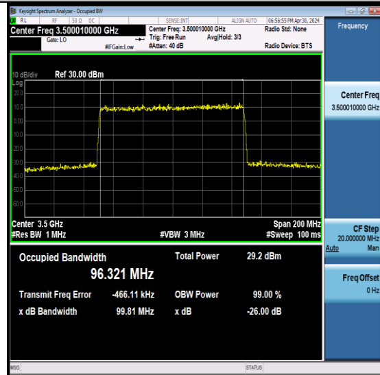
NTNV-N78-3450-3550-PC2-30-100-M-DFT-64QA M-Outter_Full-Ant6-PASS
