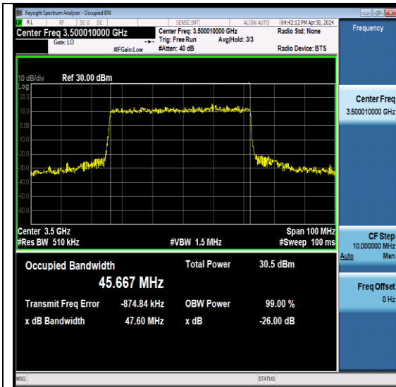
NTNV-N78-3450-3550-PC2-30-50-M-DFT-QPSK-Outer_Full-Ant6-PASS
