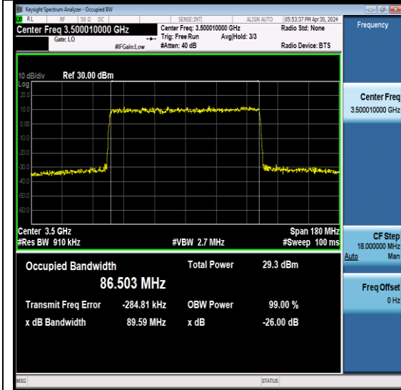
NTNV-N78-3450-3550-PC2-30-90-M-DFT-64QAM-Outer_Full-Ant6-PASS
