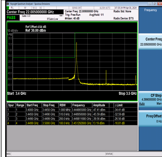
NTNV-N78-3450-3550-PC2-30-50-L-DFT-QPSK-Edge_1RB_Left-Ant6-PASS
