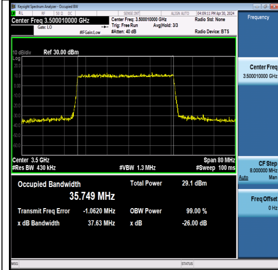
NTNV-N78-3450-3550-PC2-30-40-M-DFT-256QA M-Outer_Full-Ant6-PASS
