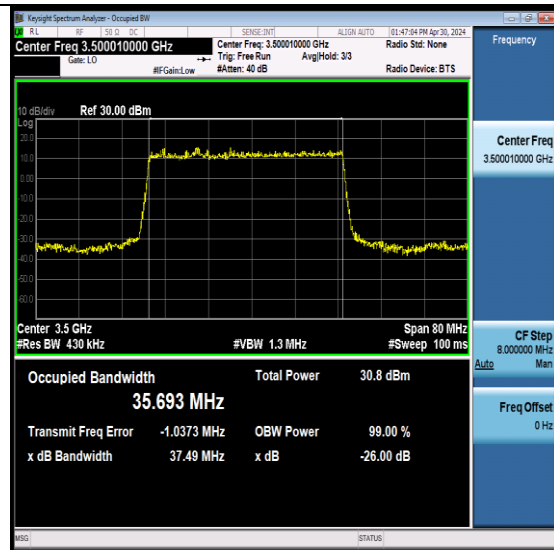
NTNV-N78-3450-3550-PC2-30-40-M-DFT-PI2BPS K-Outer_Full-Ant6-PASS
