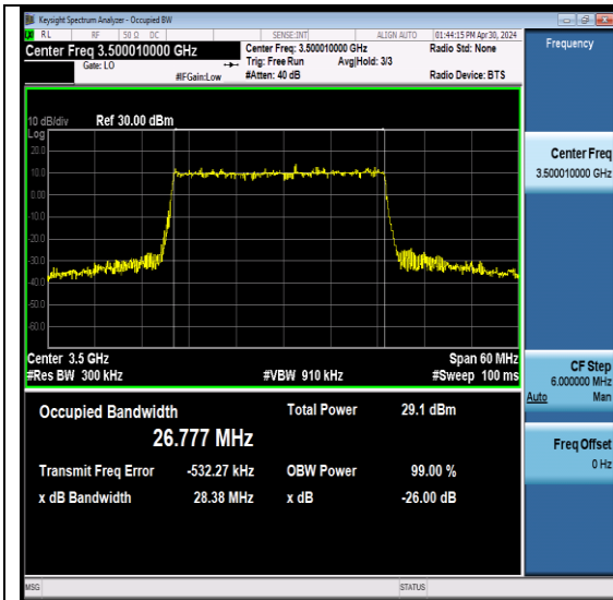
NTNV-N78-3450-3550-PC2-30-30-M-DFT-256QA M-Outer_Full-Ant6-PASS
