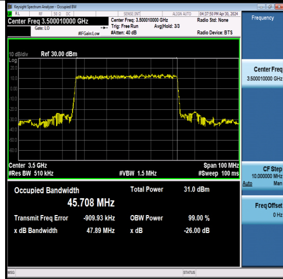
NTNV-N78-3450-3550-PC2-30-50-M-DFT-PI2BPS K-Outer_Full-Ant6-PASS
