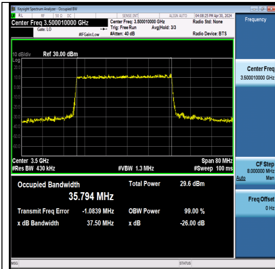
NTNV-N78-3450-3550-PC2-30-40-M-DFT-16QAM -Outer_Full-Ant6-PASS
