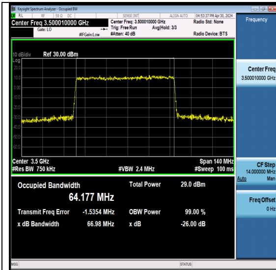
NTNV-N78-3450-3550-PC2-30-70-M-DFT-64QAM -Outer_Full-Ant6-PASS
