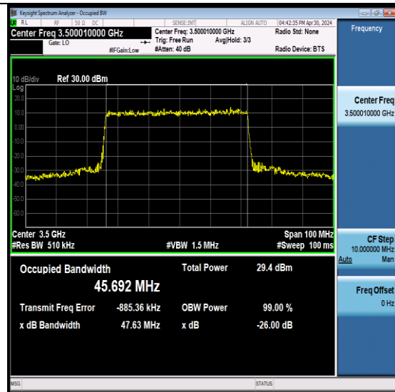
NTNV-N78-3450-3550-PC2-30-50-M-DFT-16QAM-Outer_Full-Ant6-PASS
