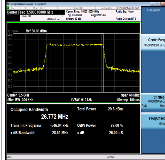
NTNV-N78-3450-3550-PC2-30-30-M-DFT-16QAM -Outer_Full-Ant6-PASS
