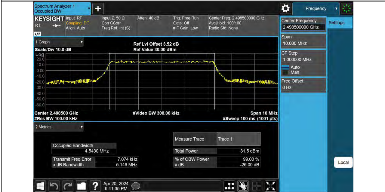
Band41-5MHz-16QAM-39675-25RB#0-PASS
