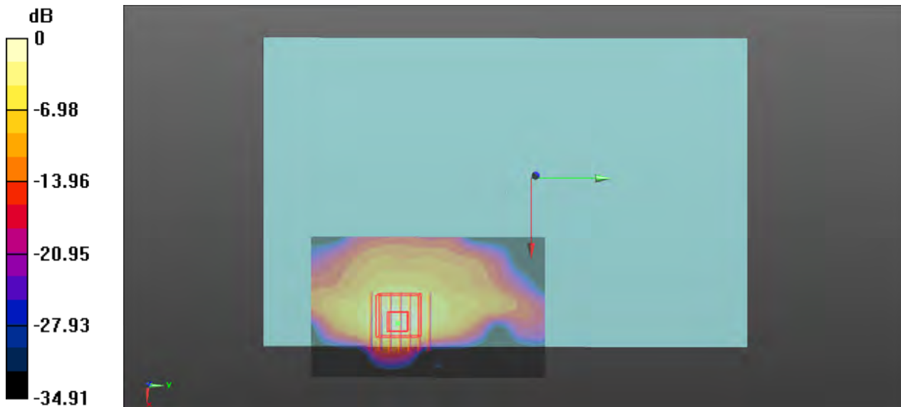
0 dB = 0.270 W/kg
