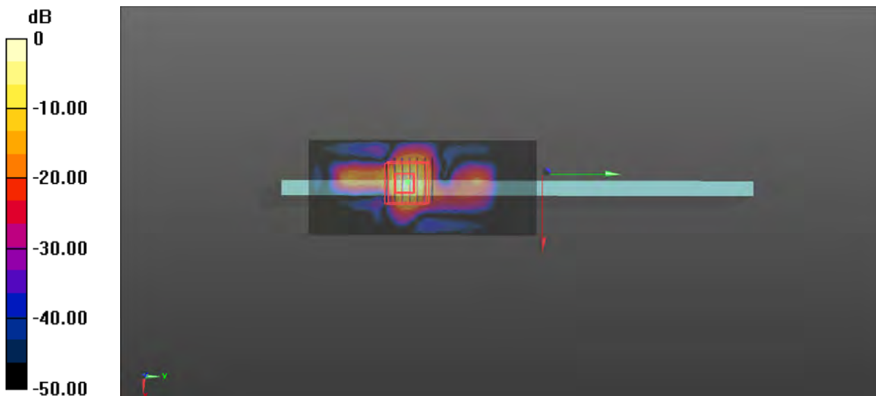
0 dB = 2.67 W/kg
