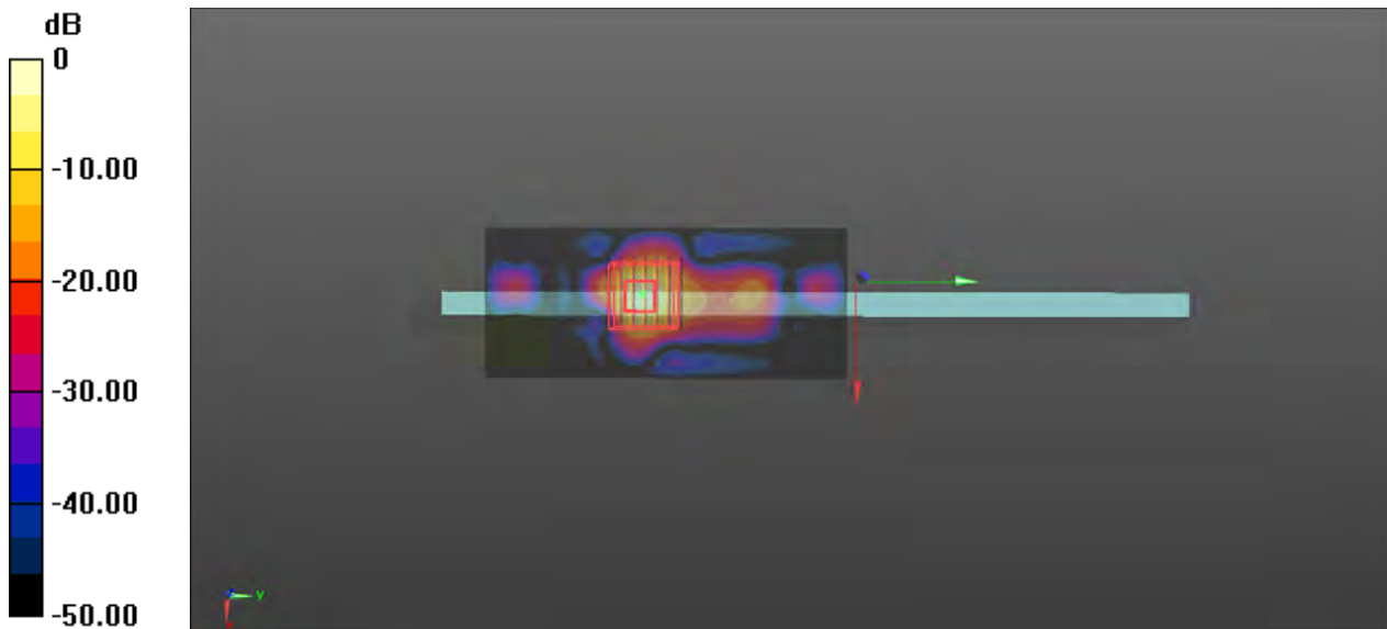
0 dB = 2.45 W/kg
