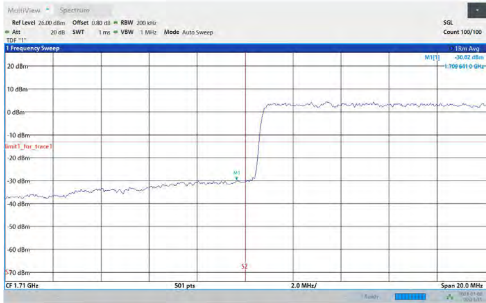
Band66-15MHz-64QAM-132047-1RB#0
