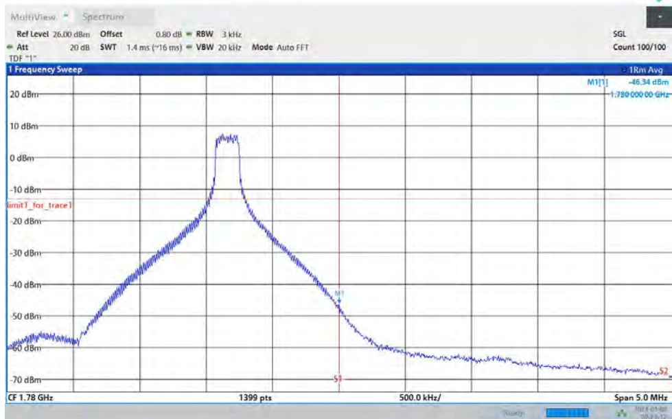
Band66-15MHz-QPSK-132597-75RB#0
