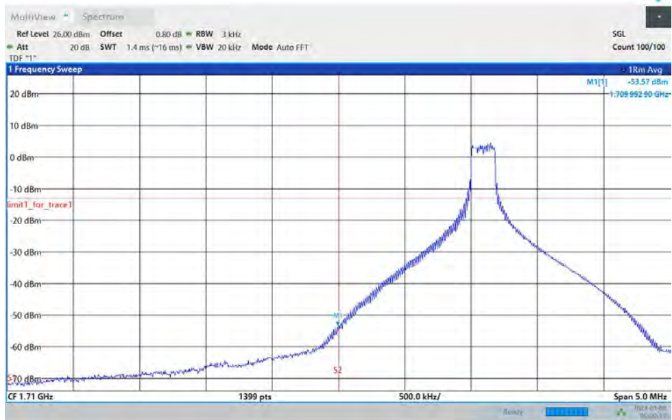
Band66-20MHz-64QAM-132072-100RB#0
