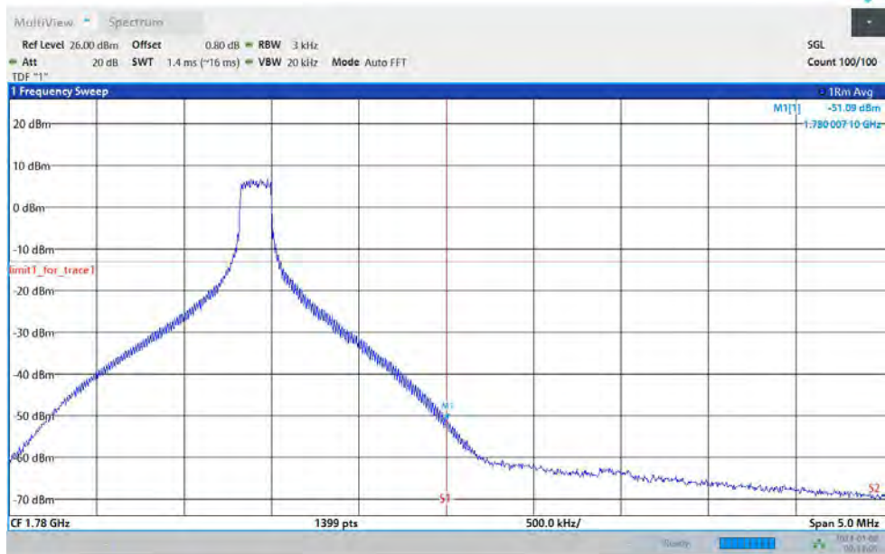
Band66-20MHz-16QAM-132572-100RB#0
