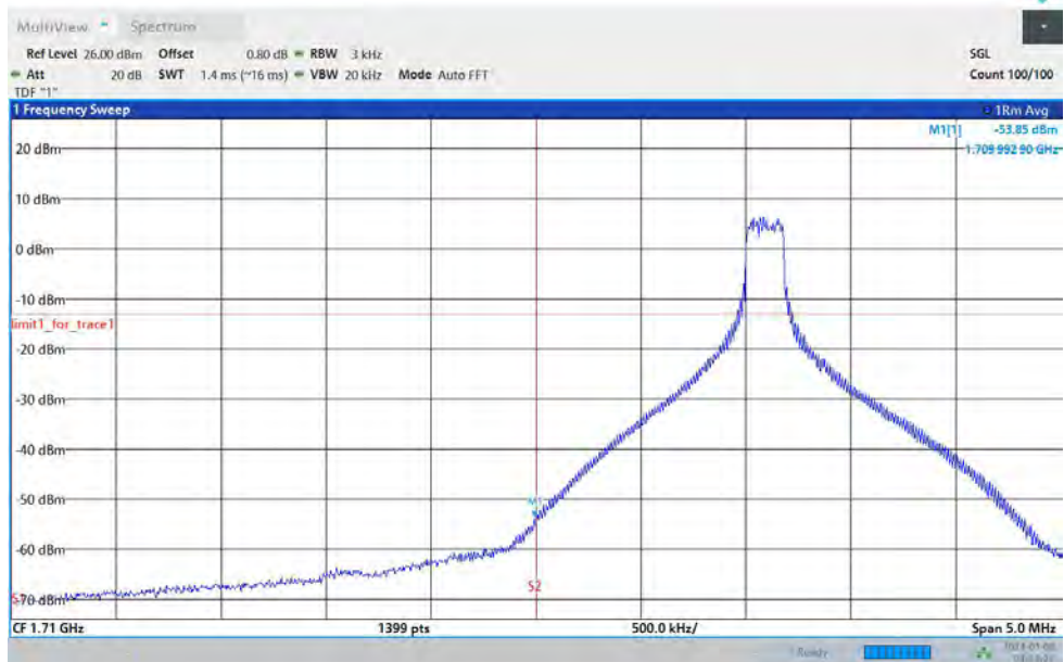
Band66-20MHz-QPSK-132072-100RB#0
