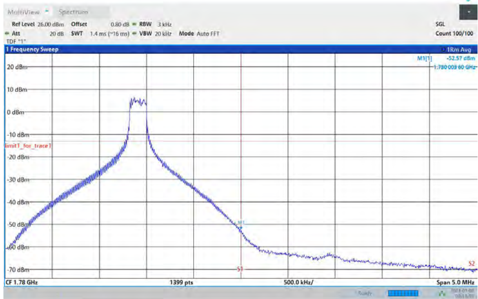
Band66-20MHz-64QAM-132572-100RB#0
