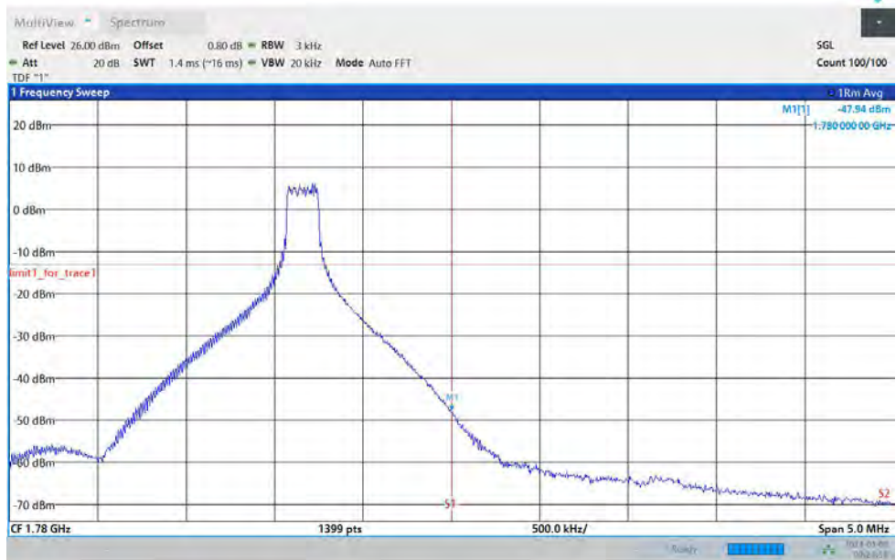
Band66-15MHz-64QAM-132597-75RB#0
