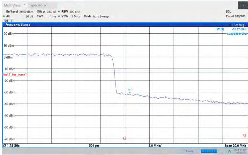
Band66-20MHz-64QAM-132572-1RB#99
