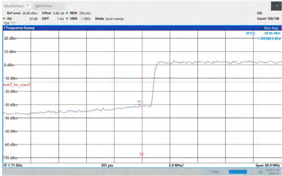
Band66-20MHz-64QAM-132072-1RB#0
