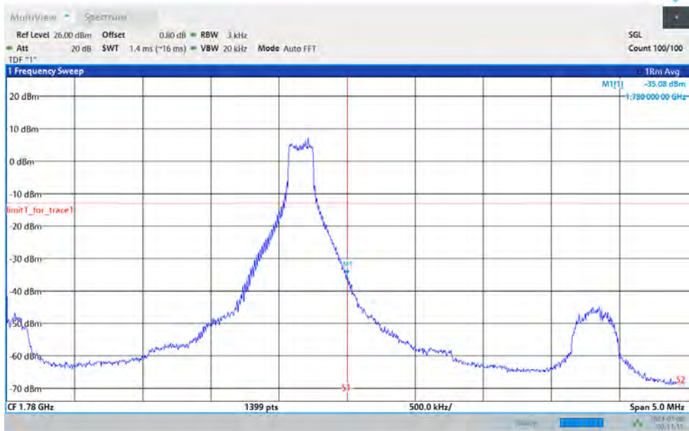
Band66-5MHz-64QAM-132647-25RB#0
