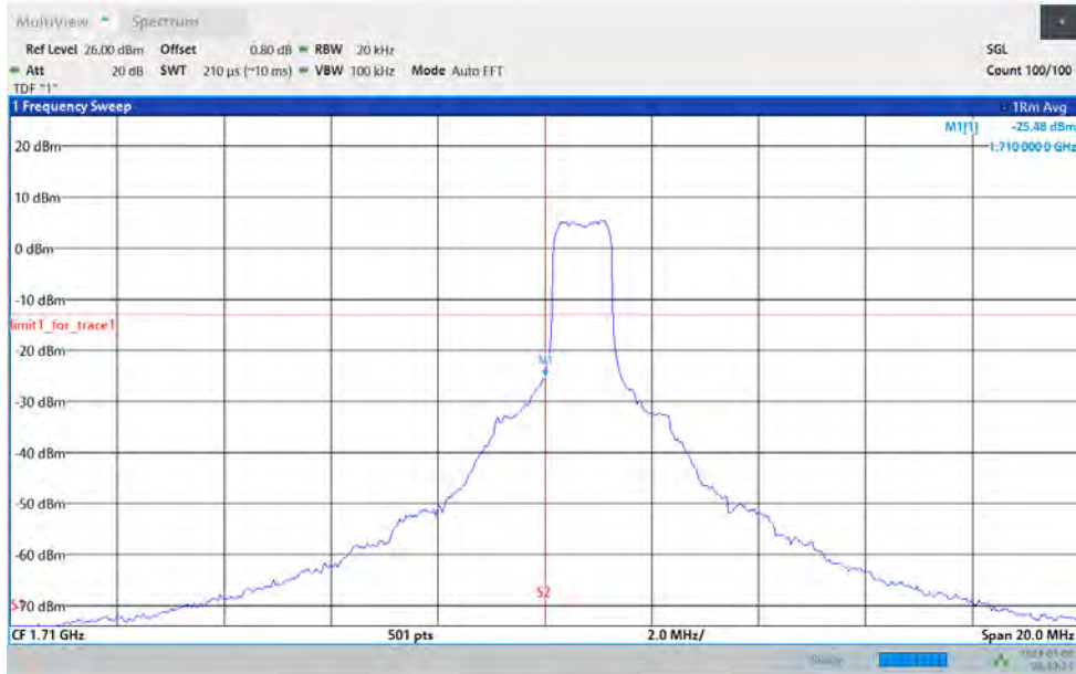
Band66-1.4MHz-16QAM-131979-1RB#0
