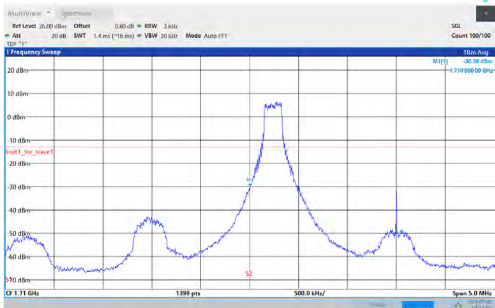
Band66-3MHz-16QAM-131987-15RB#0
