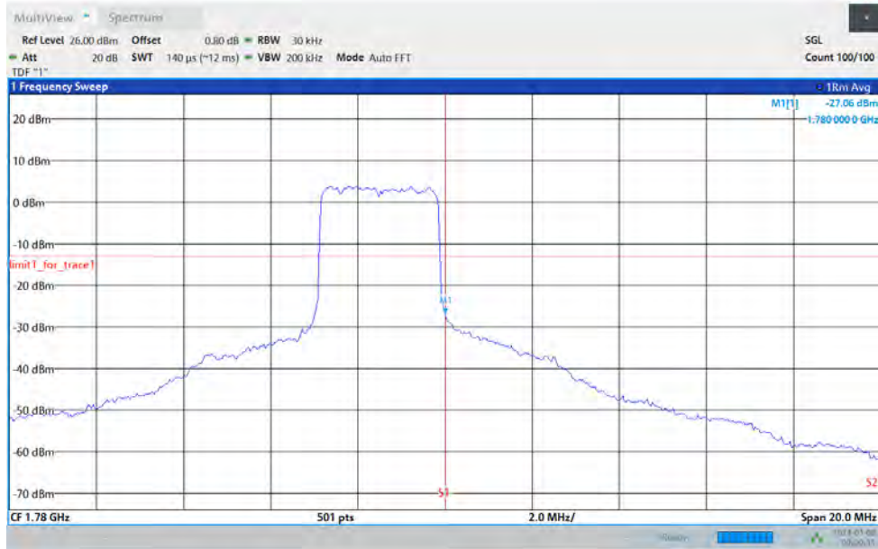
Band66-3MHz-16QAM-132657-1RB#14
