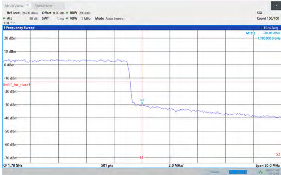
Band66-20MHz-16QAM-132572-1RB#99
