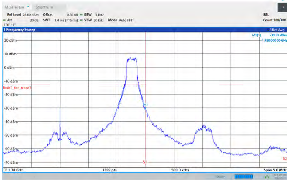
Band66-3MHz-QPSK-132657-15RB#0
