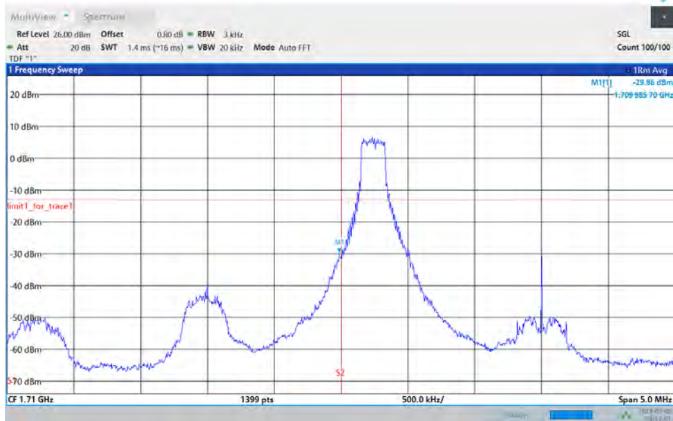
Band66-3MHz-QPSK-131987-15RB#0
