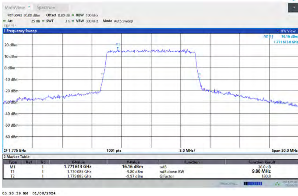
Band66-10MHz-16QAM-132622-50RB#0
