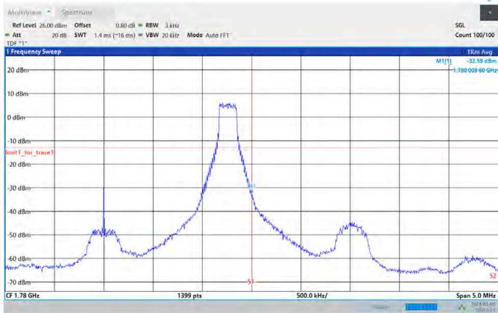
Band66-3MHz-64QAM-132657-15RB#0
