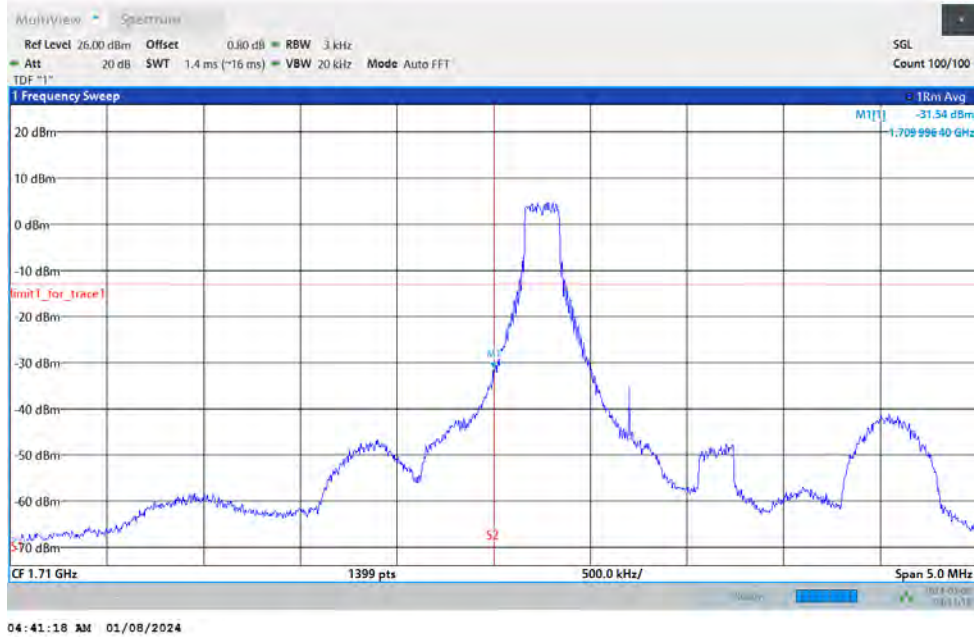
Band66-1.4MHz-64QAM-131979-6RB#0
