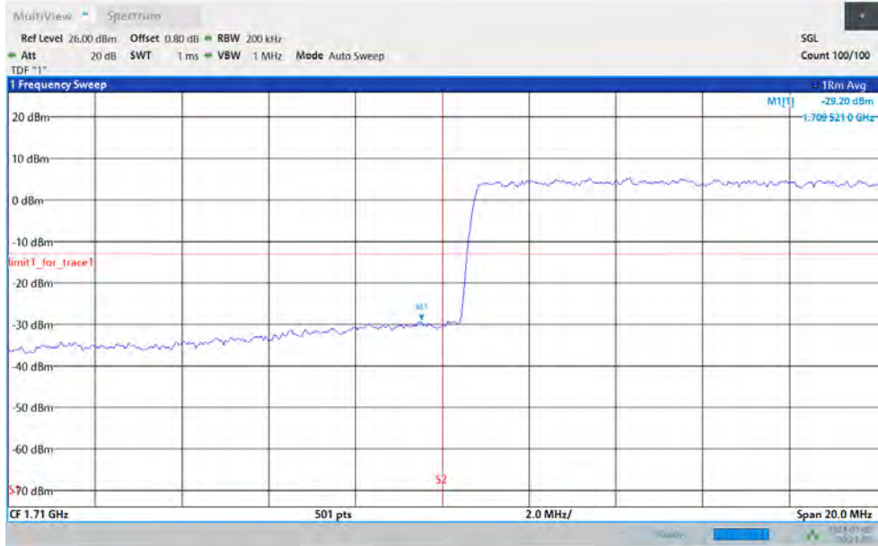
Band66-15MHz-16QAM-132047-1RB#0
