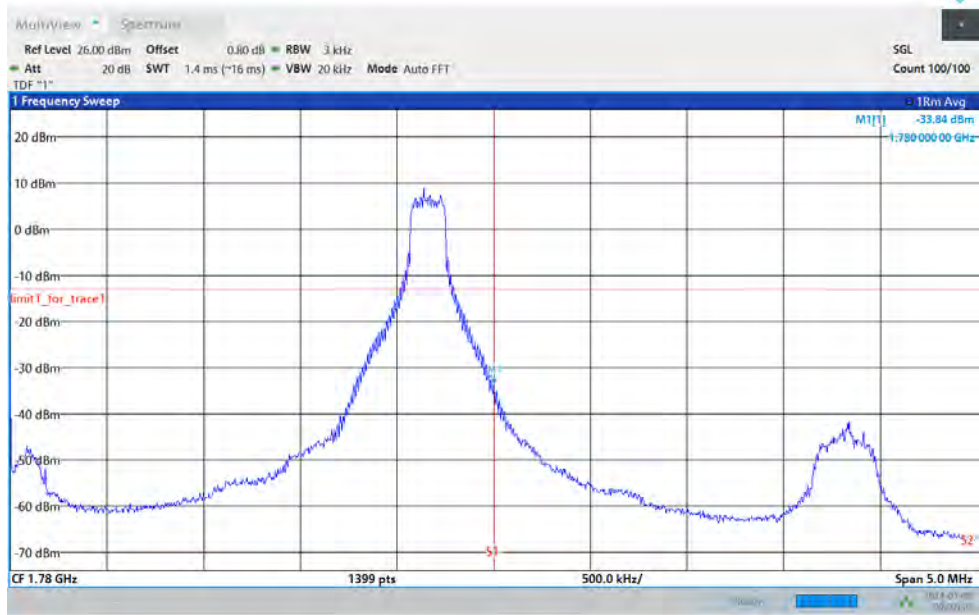
Band66-5MHz-QPSK-132647-25RB#0
