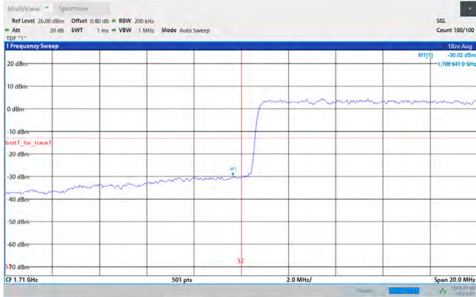
Band66-15MHz-64QAM-132047-1RB#0
