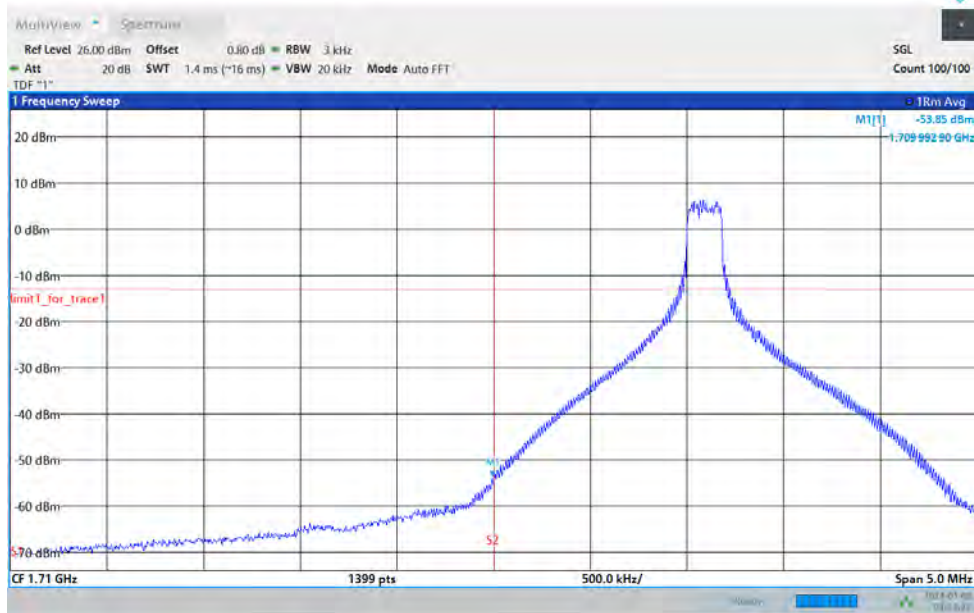
Band66-20MHz-QPSK-132072-100RB#0
