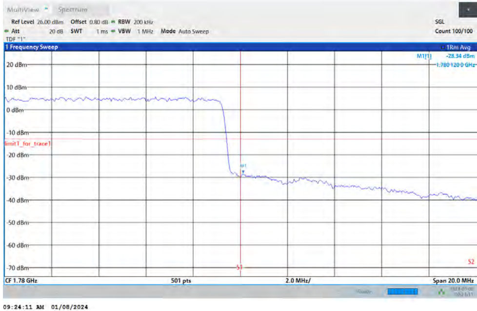
Band66-15MHz-16QAM-132597-1RB#74
