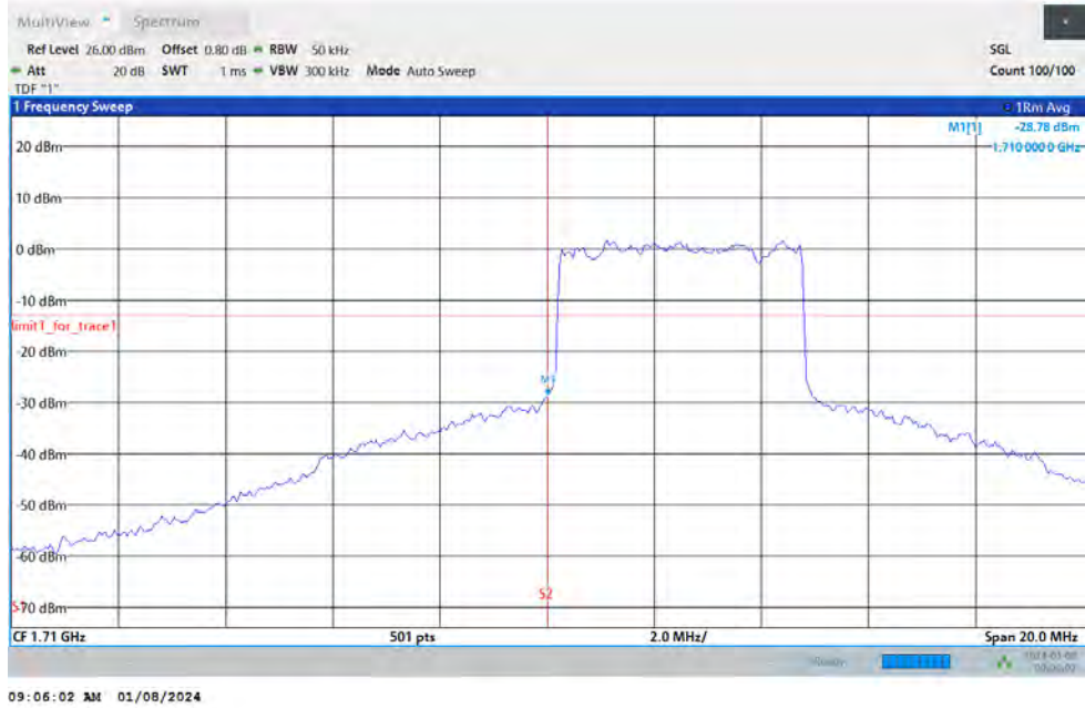
Band66-5MHz-64QAM-131997-1RB#0
