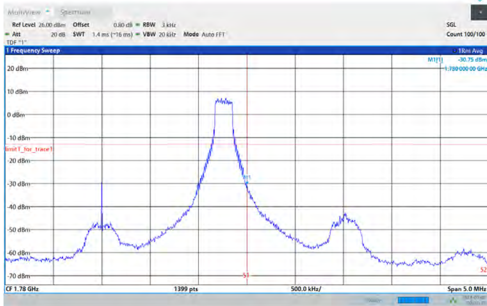
Band66-3MHz-16QAM-132657-15RB#0
