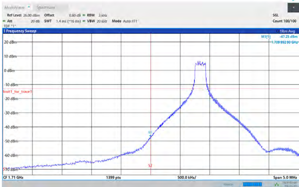
Band66-15MHz-16QAM-132047-75RB#0
