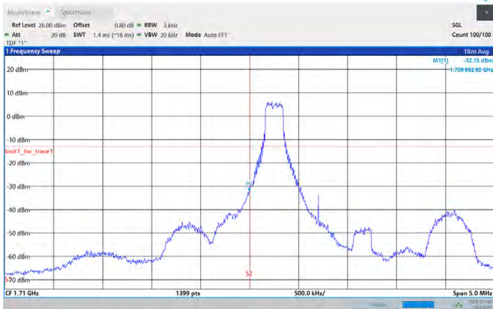
Band66-1.4MHz-16QAM-131979-6RB#0
