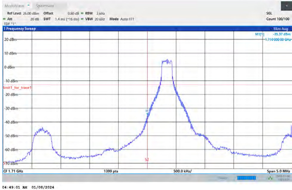
Band66-5MHz-64QAM-131997-25RB#0
