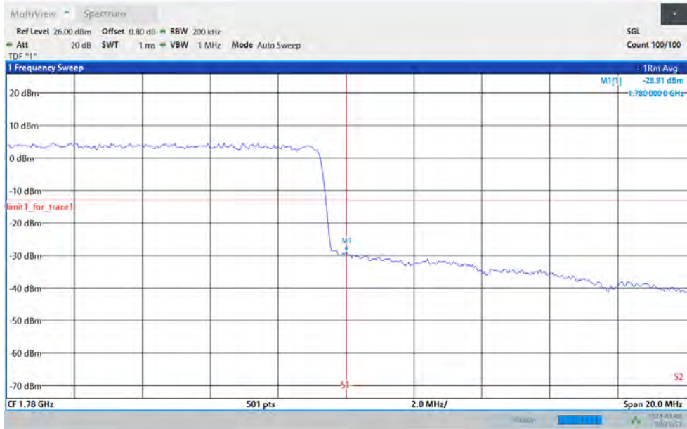
Band66-15MHz-64QAM-132597-1RB#74
