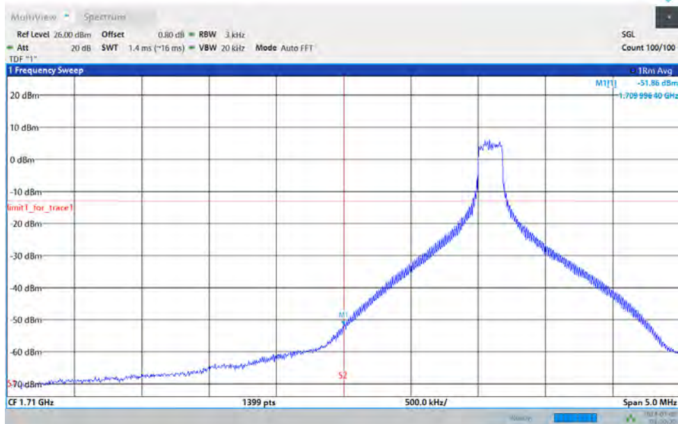
Band66-20MHz-16QAM-132072-100RB#0
