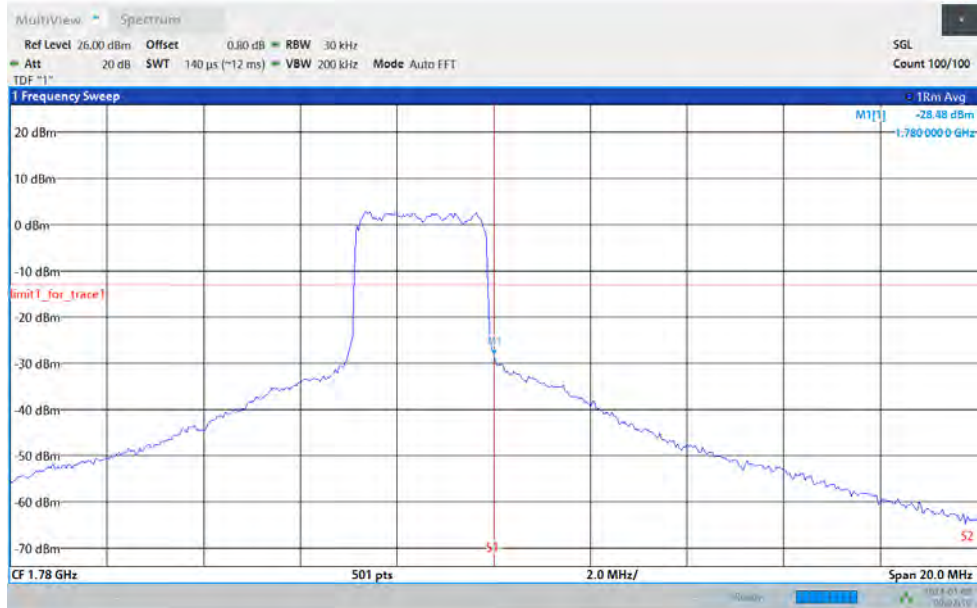
Band66-3MHz-64QAM-132657-1RB#14
