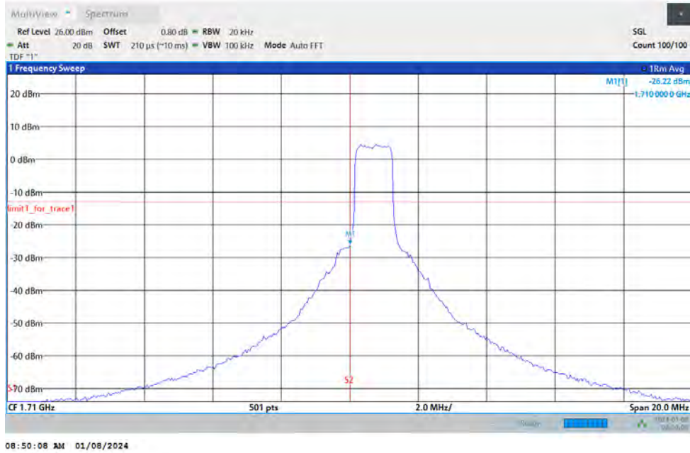
Band66-1.4MHz-64QAM-131979-1RB#0
