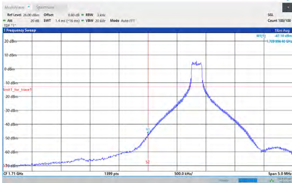
Band66-15MHz-64QAM-132047-75RB#0
