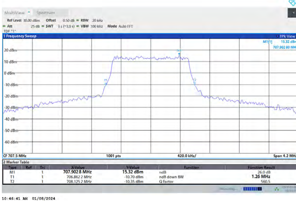
Band12-1.4MHz-64QAM-23095-6RB#0
