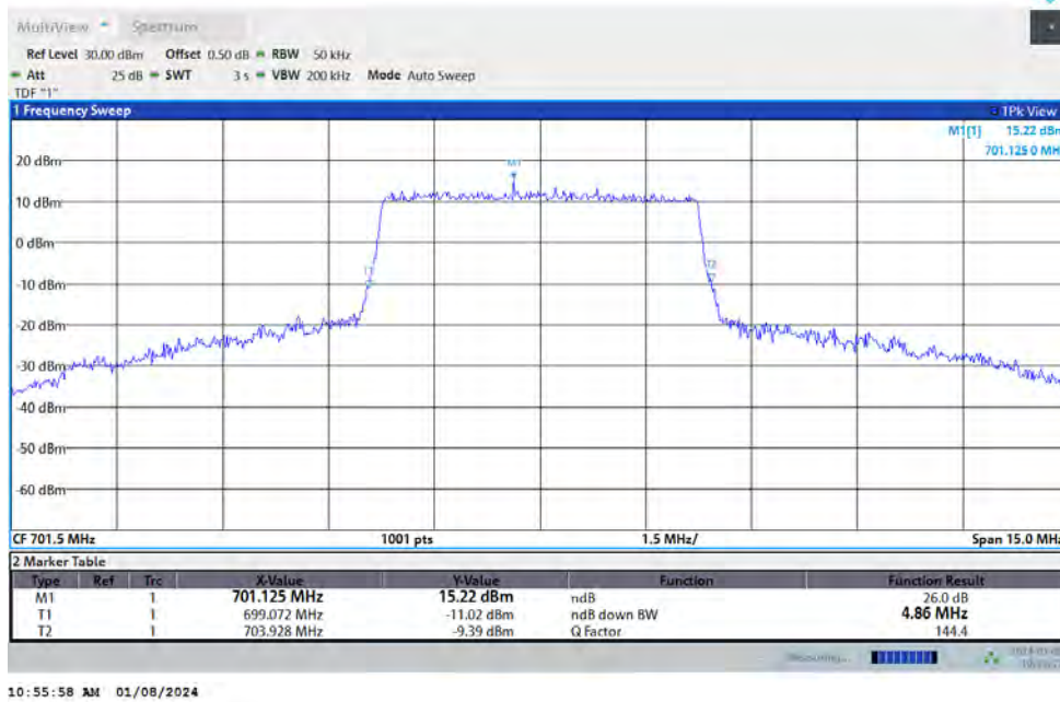
Band12-5MHz-64QAM-23035-25RB#0
