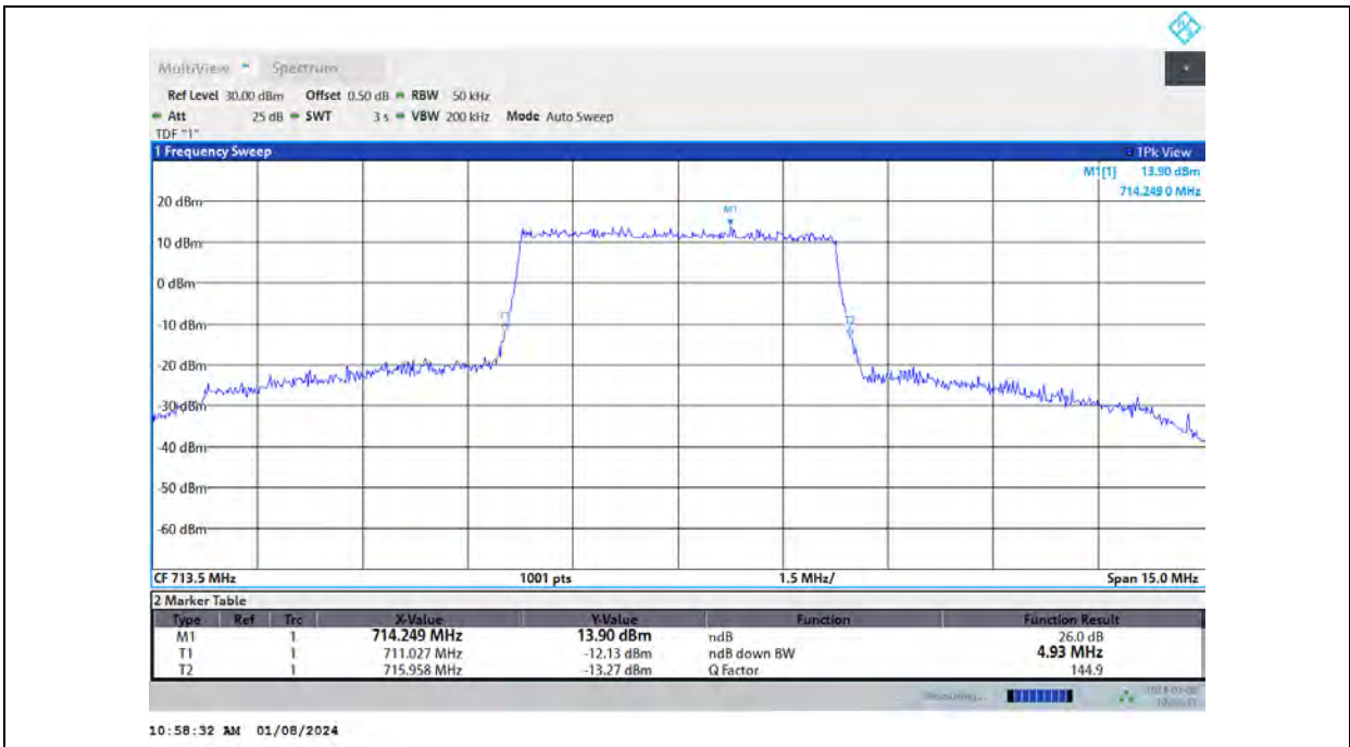
Band12-5MHz-16QAM-23155-25RB#0
