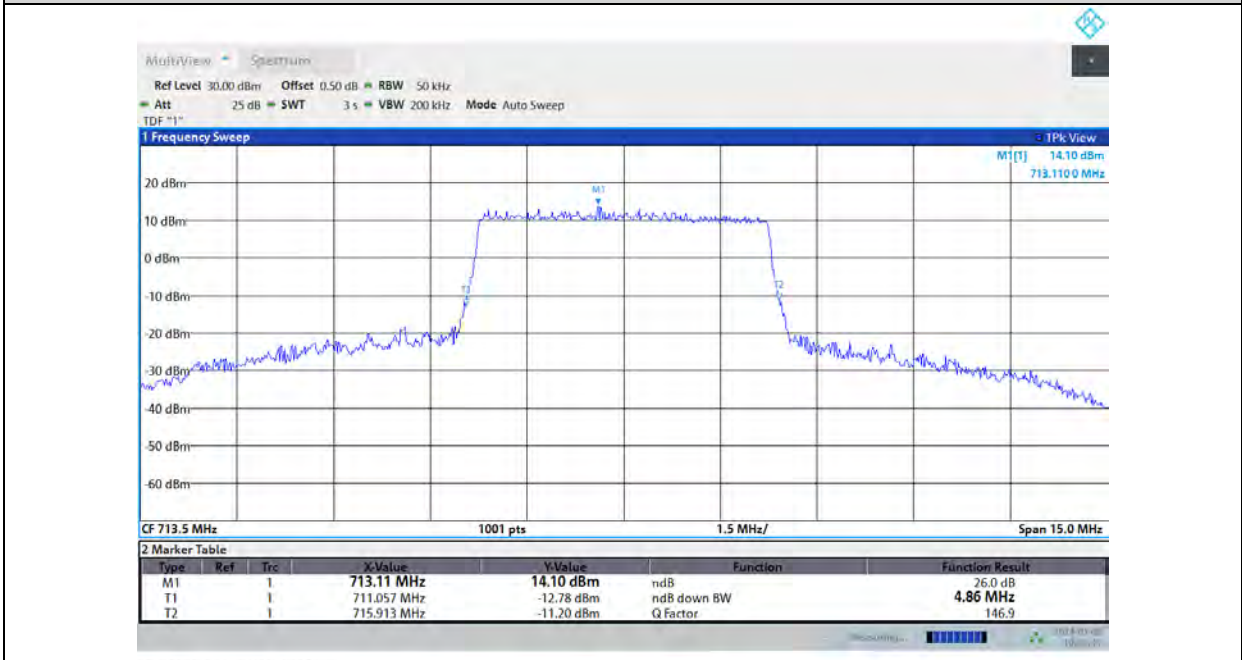
Band12-5MHz-64QAM-23155-25RB#0
