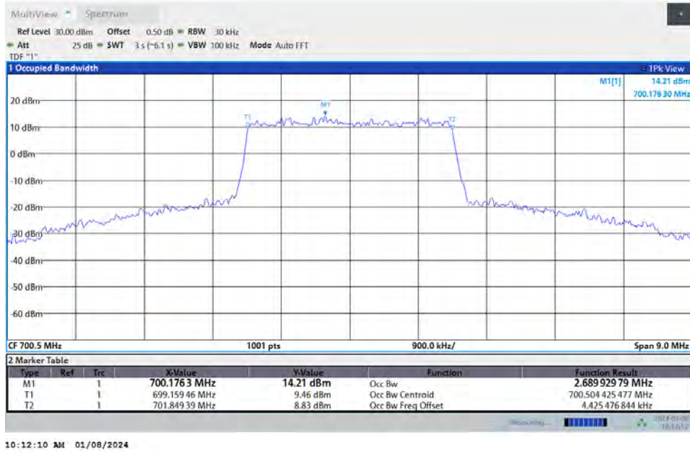
Band12-3MHz-64QAM-23025-15RB#0
