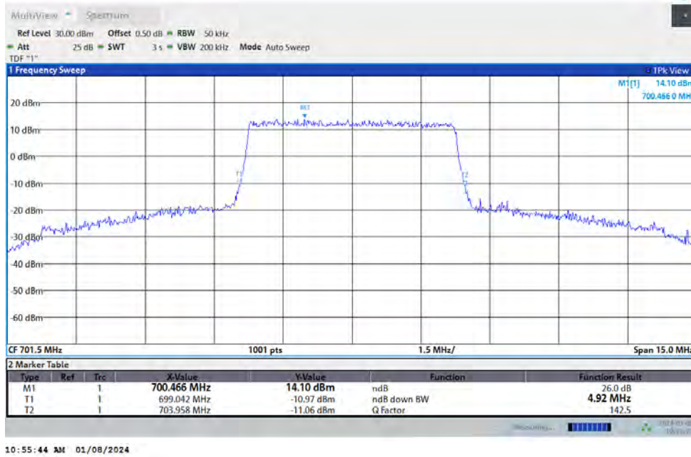
Band12-5MHz-16QAM-23035-25RB#0
