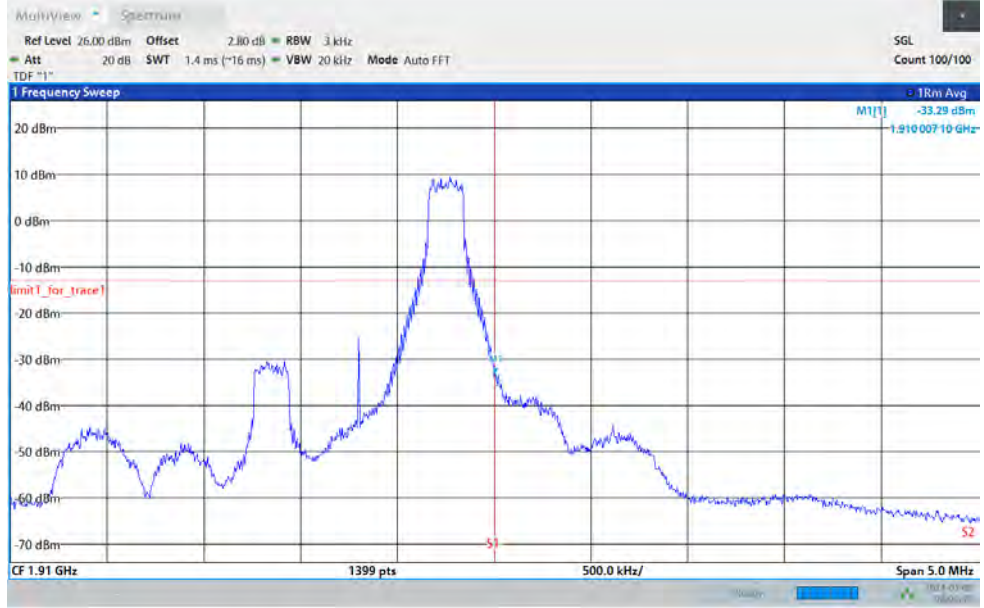
Band2-1.4MHz-16QAM-19193-6RB#0
