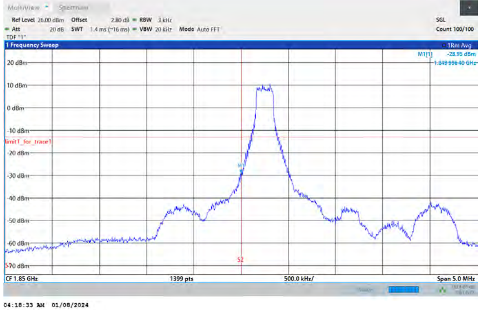
Band2-1.4MHz-64QAM-18607-6RB#0
