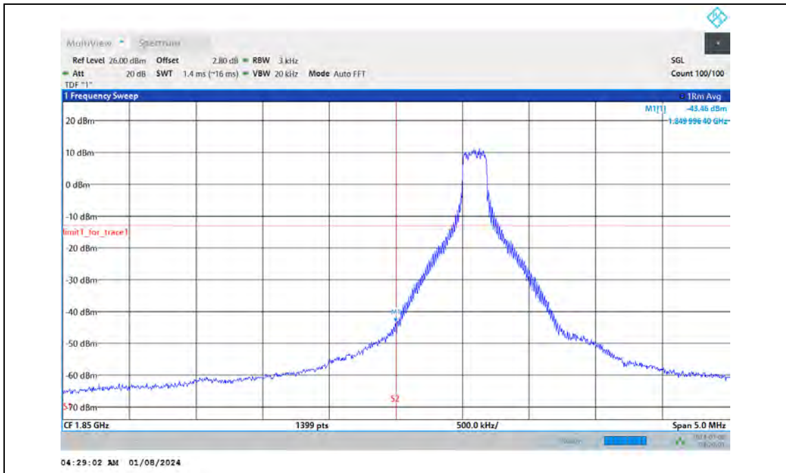
Band2-10MHz-16QAM-18650-50RB#0
