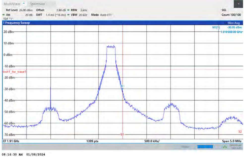
Band2-3MHz-64QAM-19185-15RB#0
