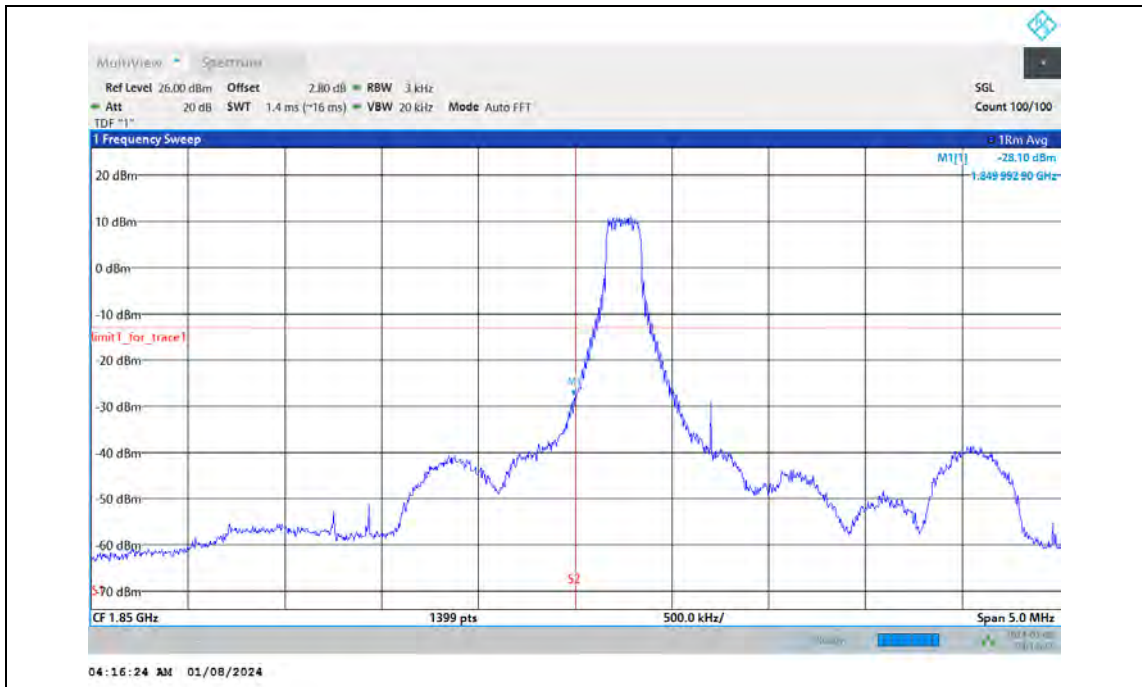
Band2-1.4MHz-QPSK-18607-6RB#0
