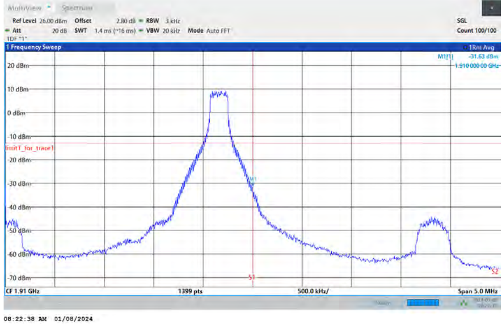
Band2-5MHz-16QAM-19175-25RB#0
