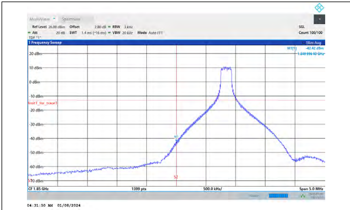
Band2-15MHz-QPSK-18675-75RB#0
