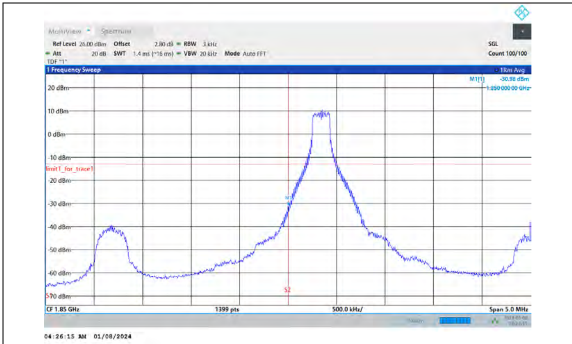
Band2-5MHz-64QAM-18625-25RB#0
