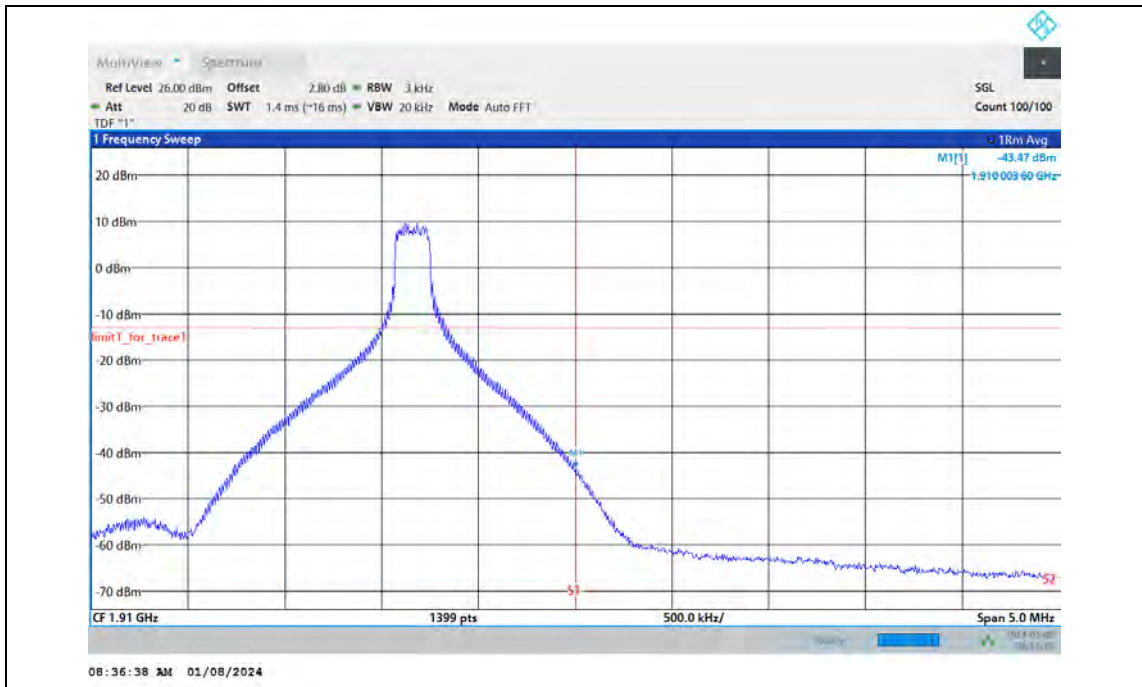
Band2-15MHz-QPSK-19125-75RB#0
