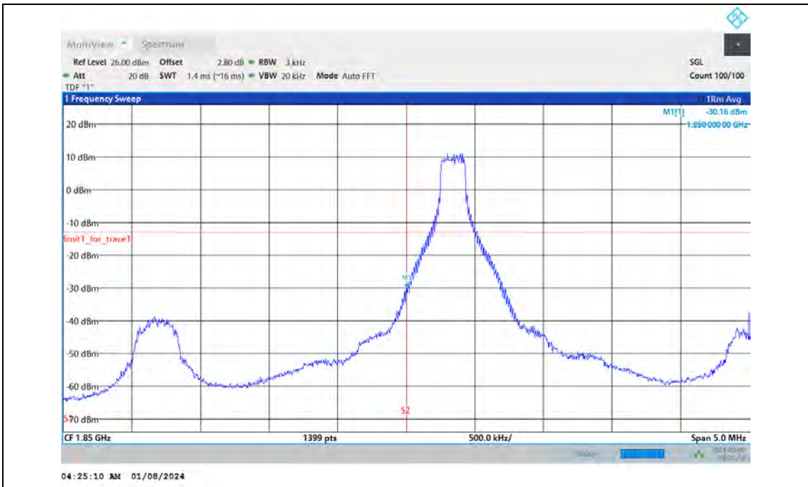
Band2-5MHz-16QAM-18625-25RB#0
