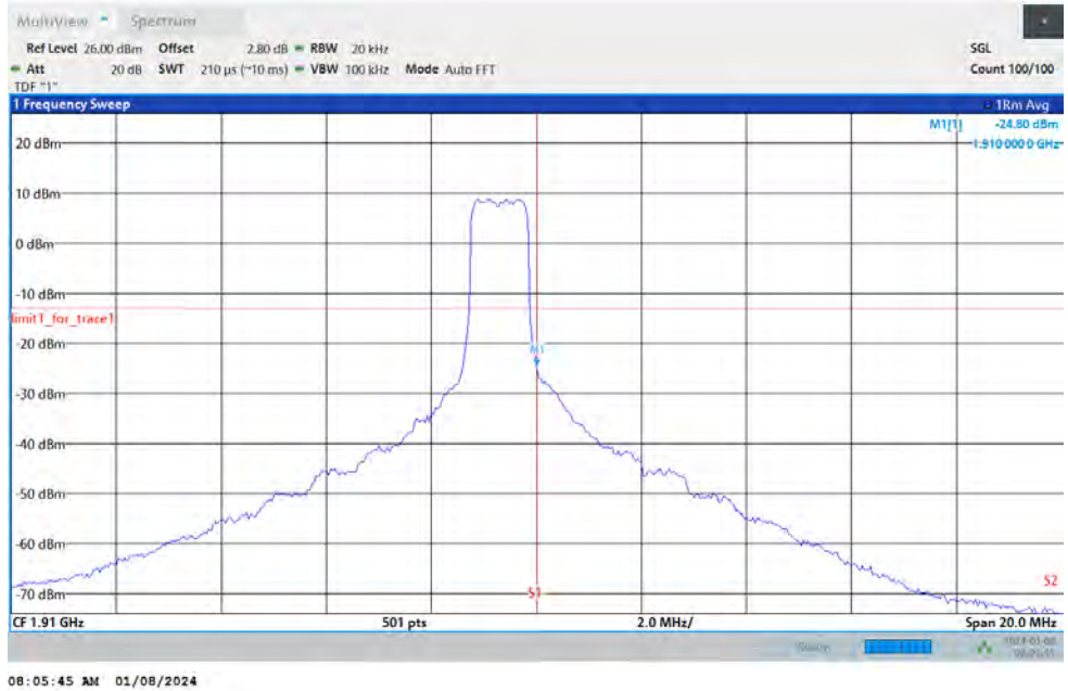
Band2-1.4MHz-16QAM-18607-1RB#0
