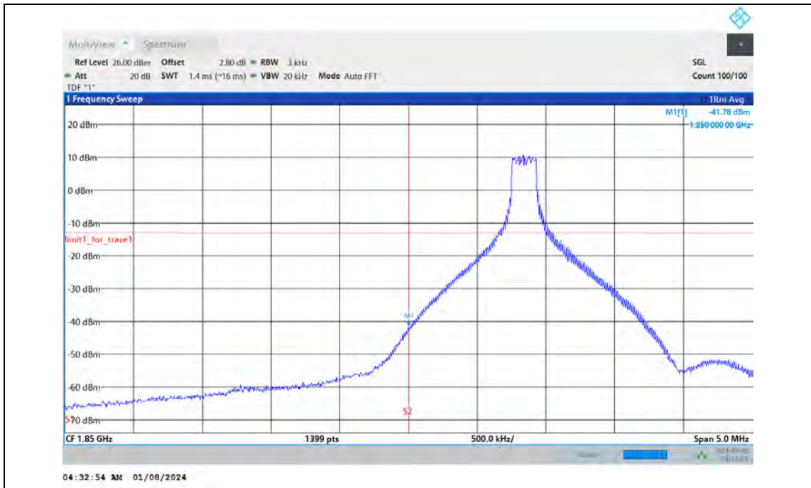
Band2-15MHz-16QAM-18675-75RB#0
