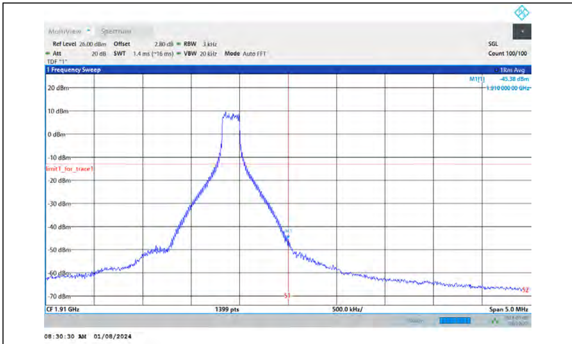
Band2-10MHz-16QAM-19150-50RB#0
