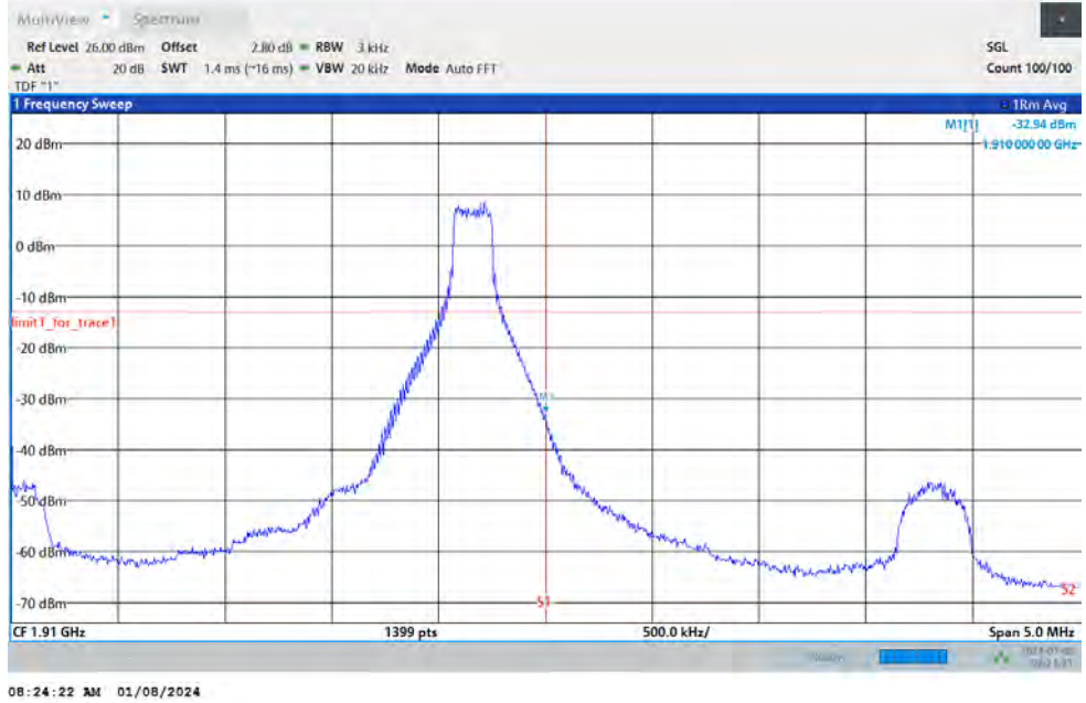
Band2-5MHz-64QAM-19175-25RB#0
