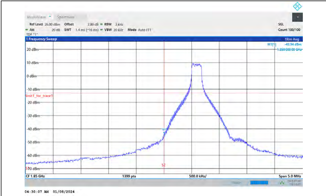
Band2-10MHz-64QAM-18650-50RB#0
