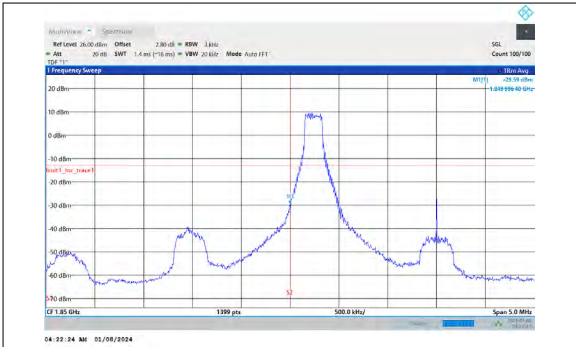
Band2-3MHz-64QAM-18615-15RB#0
