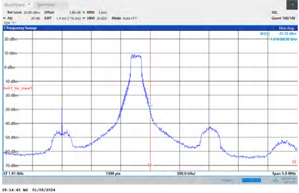
Band2-3MHz-16QAM-19185-15RB#0
