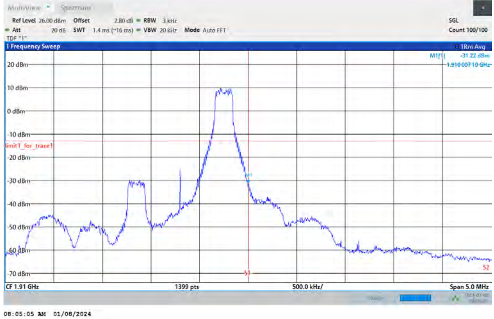
Band2-1.4MHz-QPSK-19193-6RB#0
