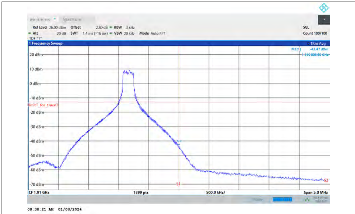
Band2-15MHz-16QAM-19125-75RB#0
