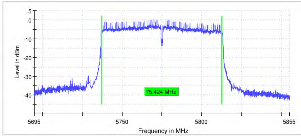
6 dB Bandwidth
