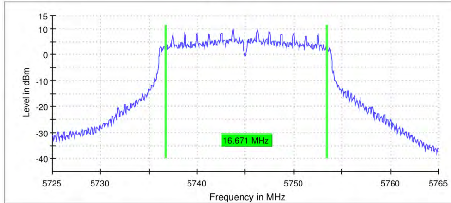
6 dB Bandwidth
