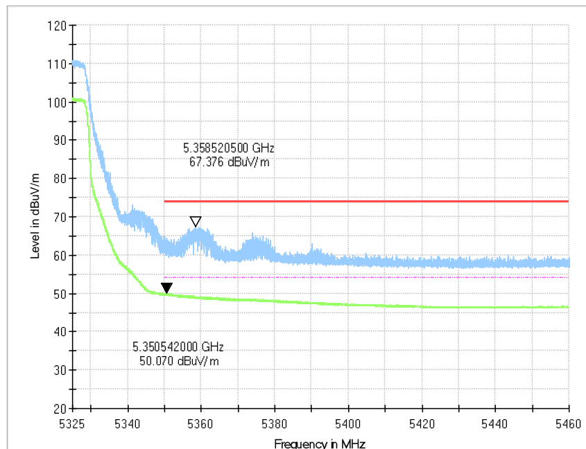
Fig.39 Band Edges (802.11n-HT20 Ch64, 5320MHz)
