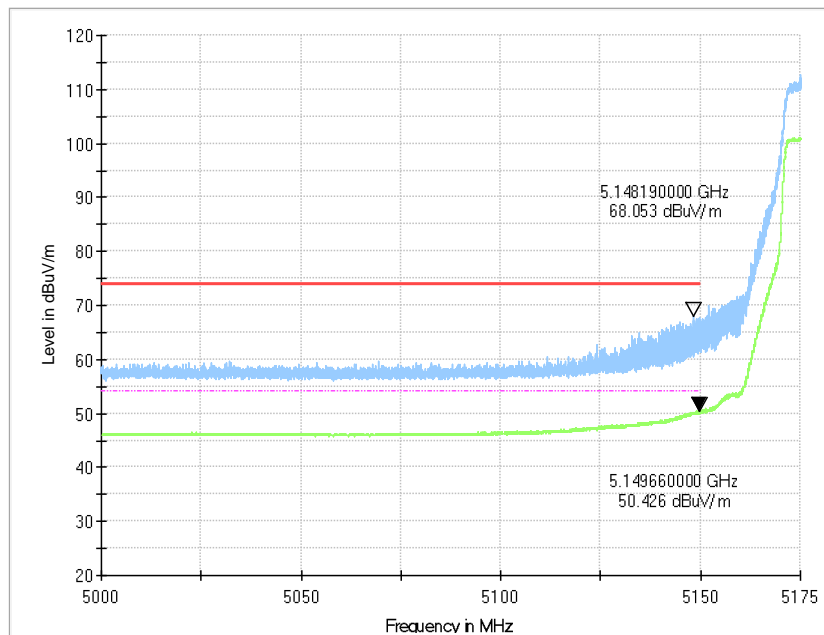
Fig.38 Band Edges (802.11n-HT20 Ch36, 5180MHz)
