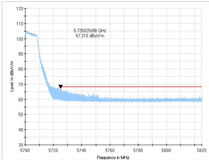
Fig.41 Band Edges (802.11n-HT20 Ch140, 5700MHz)
