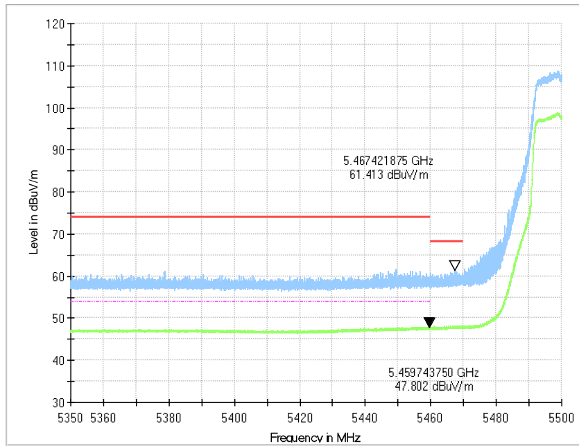
Fig.36 Band Edges (802.11a Ch100, 5500MHz)
