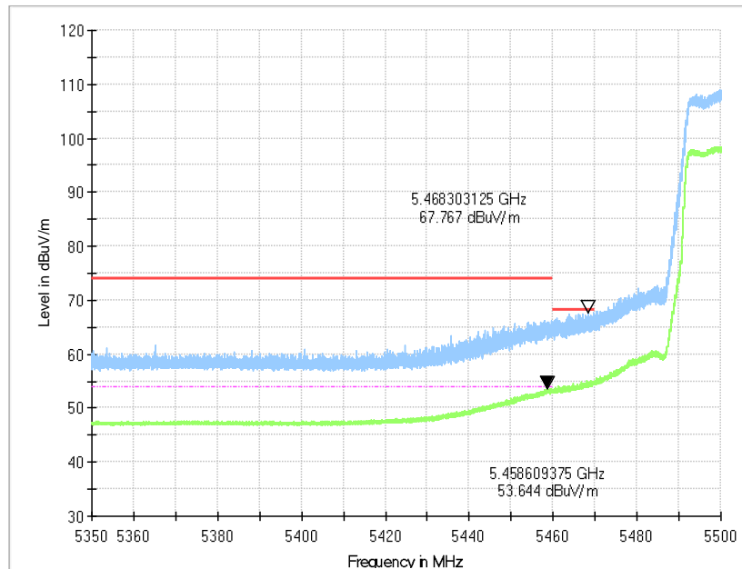
Fig.44 Band Edges (802.11n-HT40 Ch102, 5510MHz)
