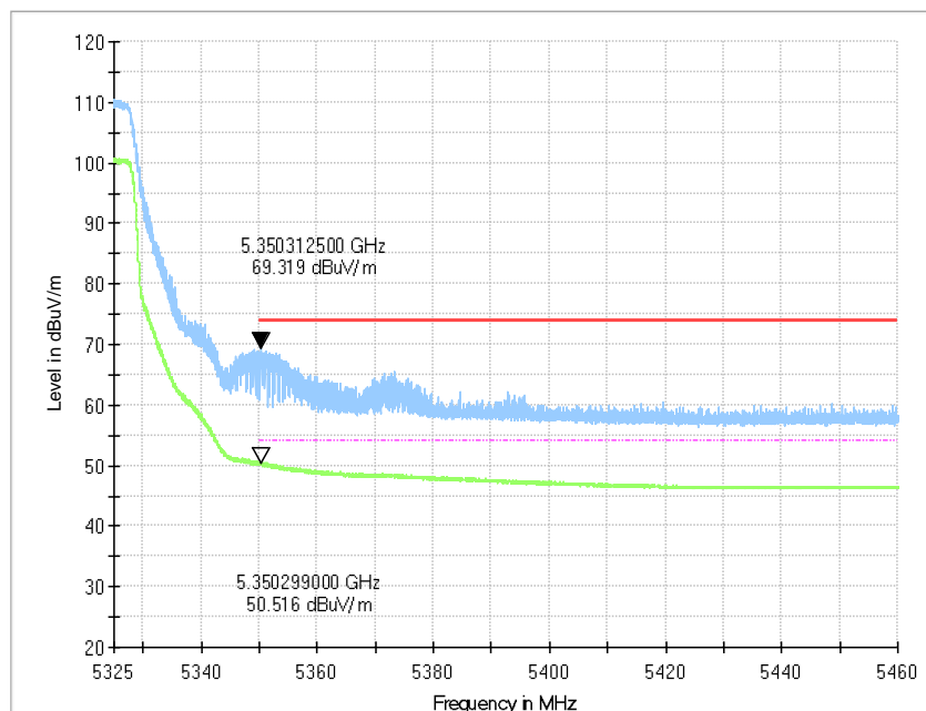
Fig.35 Band Edges (802.11a Ch64, 5320MHz)
