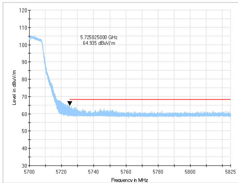
Fig.37 Band Edges (802.11a Ch140, 5700MHz)
