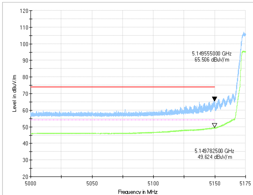
Fig.42 Band Edges (802.11n-HT40 Ch38, 5190MHz)
