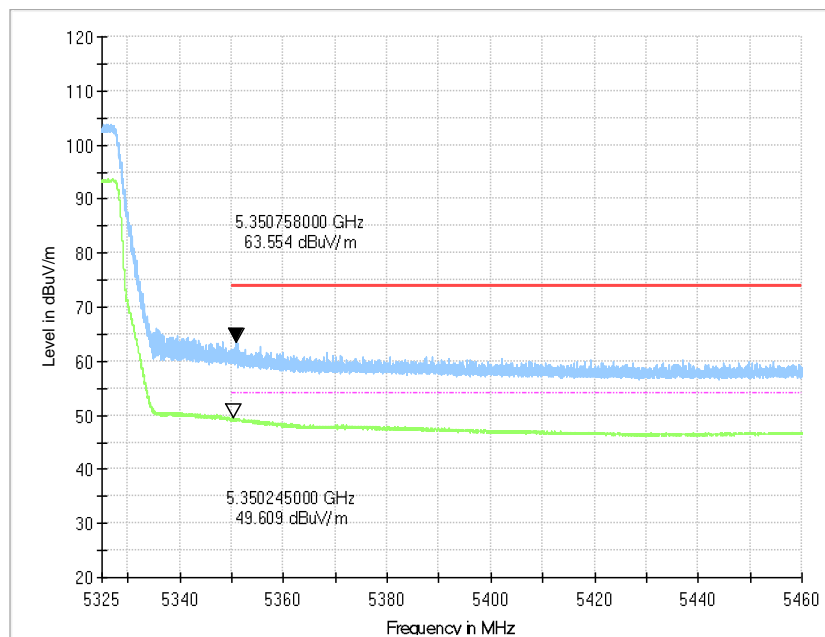
Fig.43 Band Edges (802.11n-HT40 Ch62, 5310MHz)
