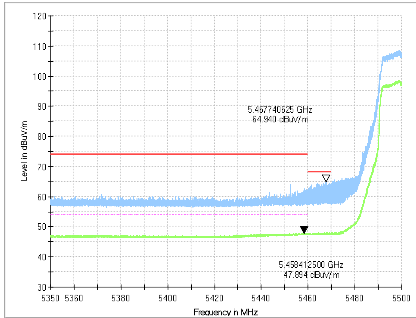
Fig.40 Band Edges (802.11n-HT20 Ch100, 5500MHz)
