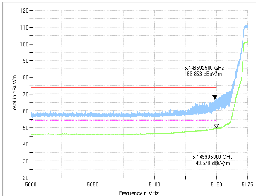
Fig.34 Band Edges (802.11a Ch36, 5180MHz)
