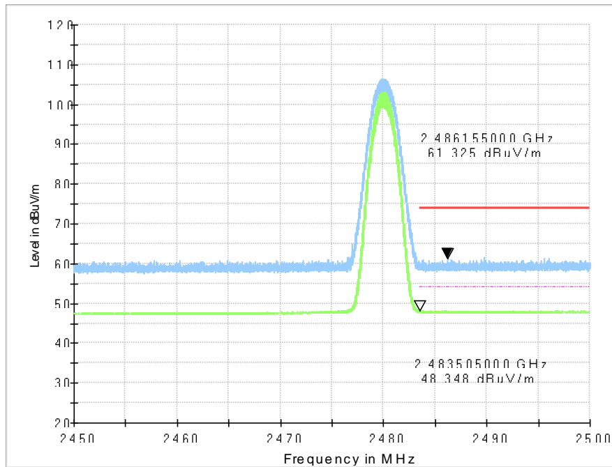
Fig.16. Frequency Band Edges: \pi/4 DQPSK, Channel 78, Hopping Off, 2.45 GHz - 2.50GHz
