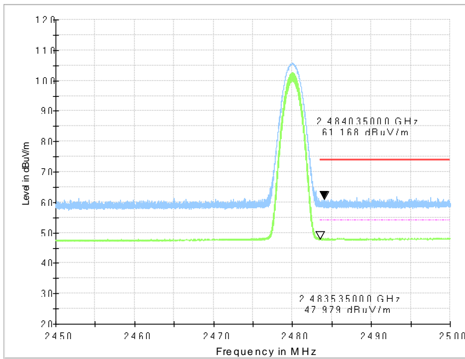
Fig.18. Frequency Band Edges: 8DPSK, Channel 78, 2.45 GHz - 2.50GHz
