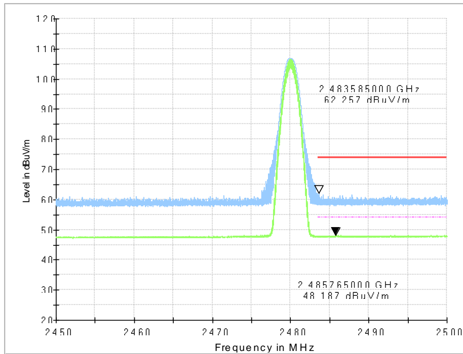
Fig.14. Frequency Band Edges: GFSK, Channel 78, Hopping Off, ch11, 2.45 GHz - 2.50GHz
