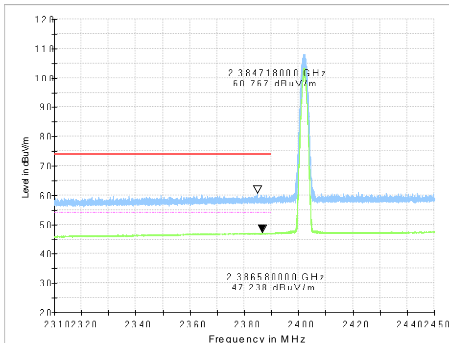
Fig.15. Frequency Band Edges: \pi/4 DQPSK, Channel 0, Hopping Off, 2.31 GHz - 2.45GHz
