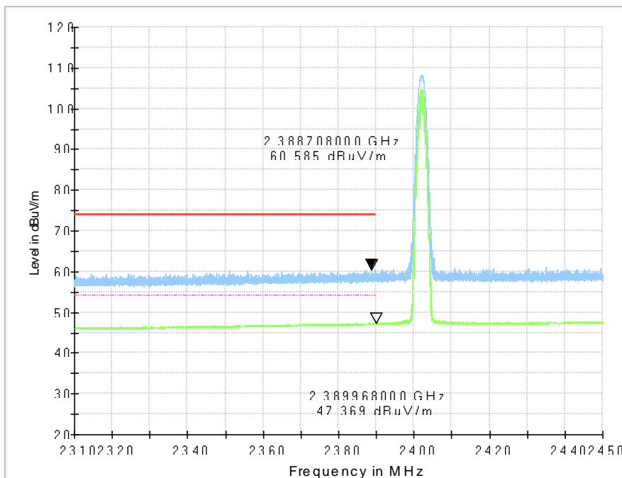
Fig.17. Frequency Band Edges: 8DPSK, Channel 0, 2.31 GHz - 2.45GHz
