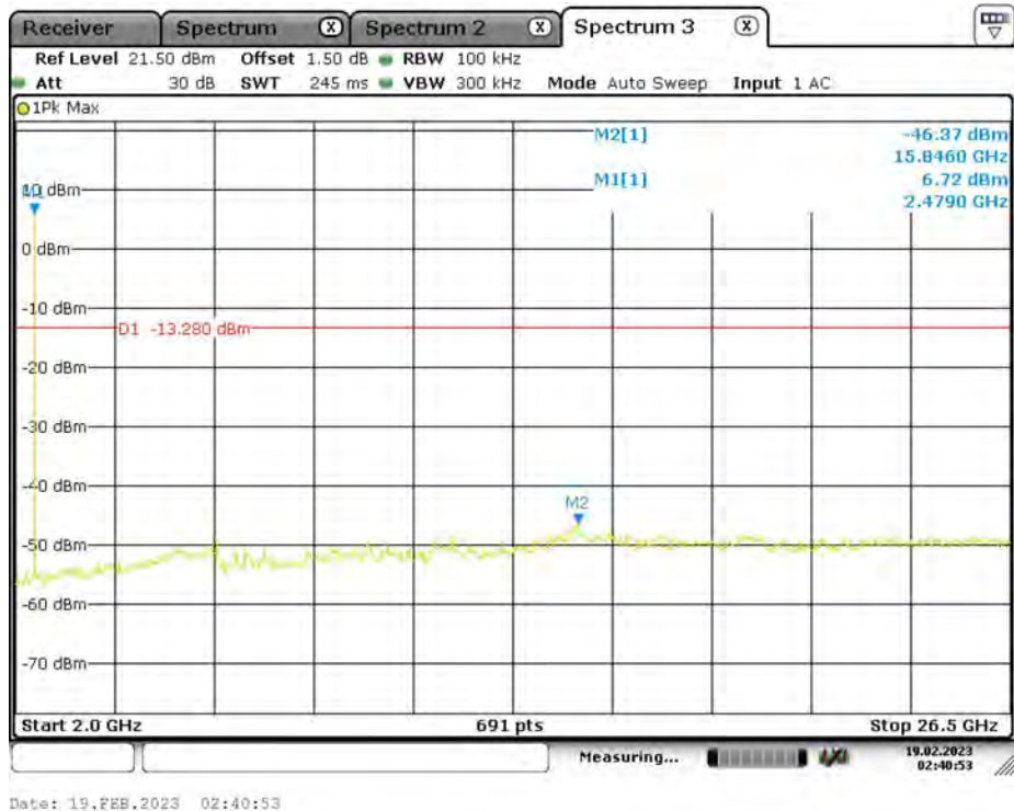
DH5_Ant1_2480_2000~26500
