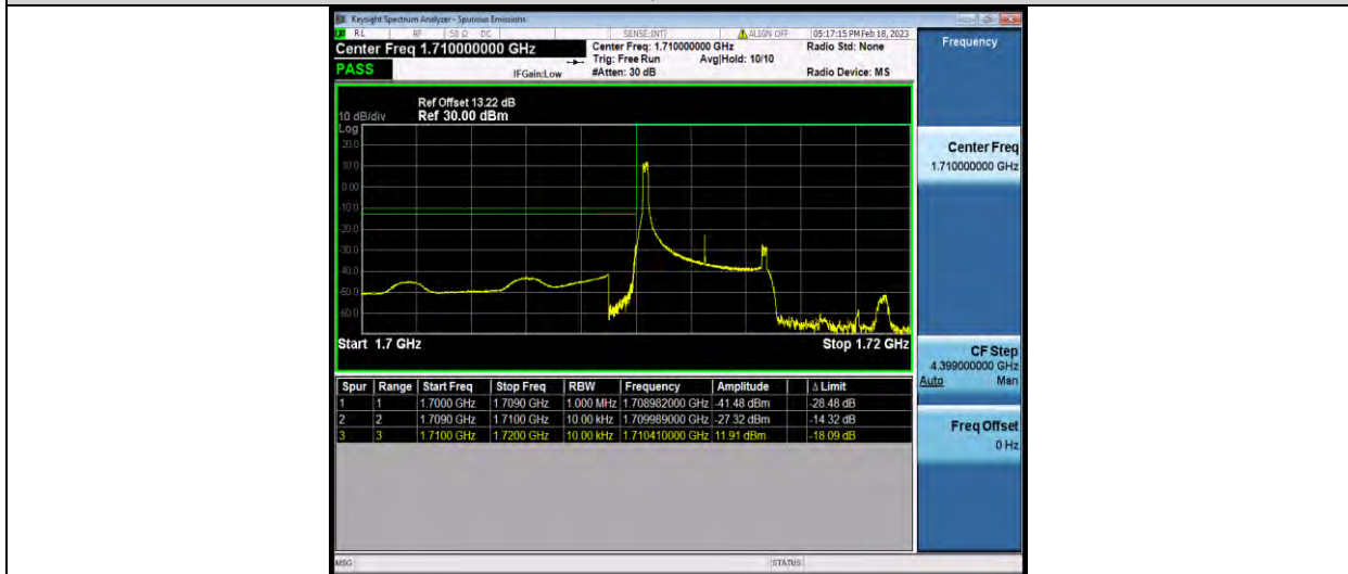
Band66-5MHz-QPSK-131997-25RB#0
