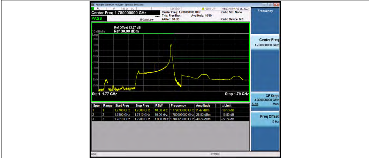
Band66-5MHz-QPSK-132647-25RB#0
