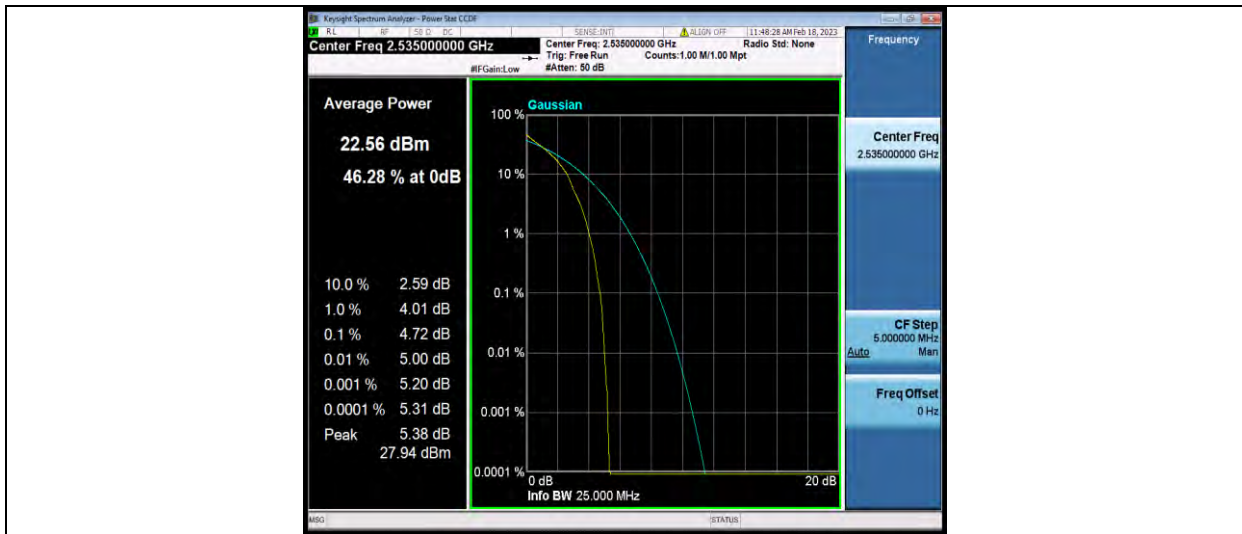
Band7-10MHz-QPSK-21100-50RB#0
