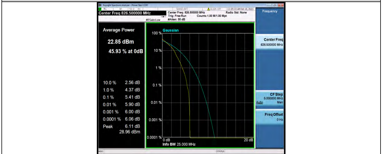
Band5-5MHz-QPSK-20425-25RB#0
