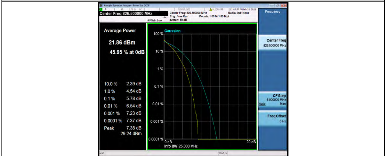
Band5-5MHz-QPSK-20525-1RB#0
