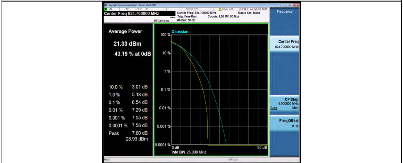
Band5-1.4MHz-16QAM-20525-1RB#0
