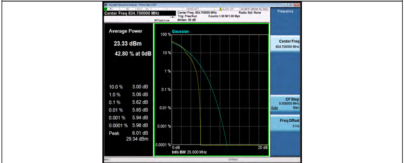
Band5-1.4MHz-16QAM-20407-6RB#0
