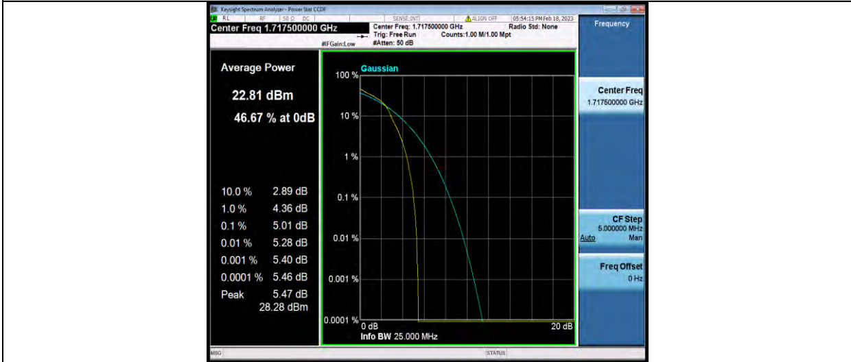
Band66-15MHz-16QAM-132047-75RB#0
