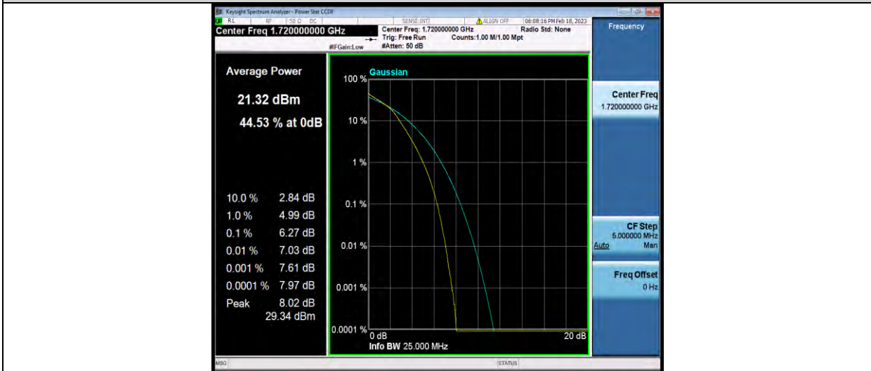
Band66-20MHz-16QAM-132322-1RB#0
