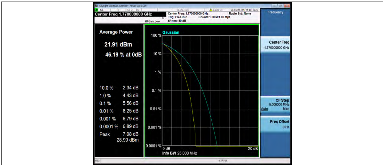
Band66-20MHz-16QAM-132072-1RB#0
