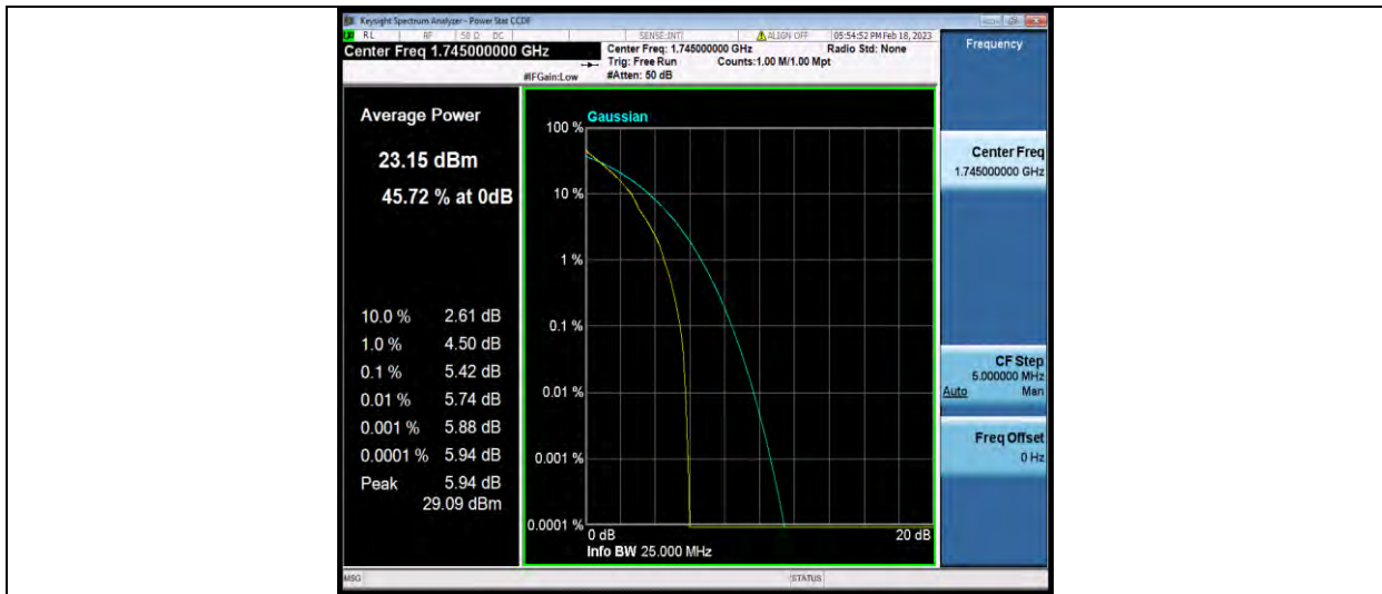
Band66-15MHz-QPSK-132322-75RB#0
