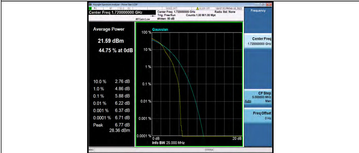
Band66-20MHz-16QAM-132072-100RB#0
