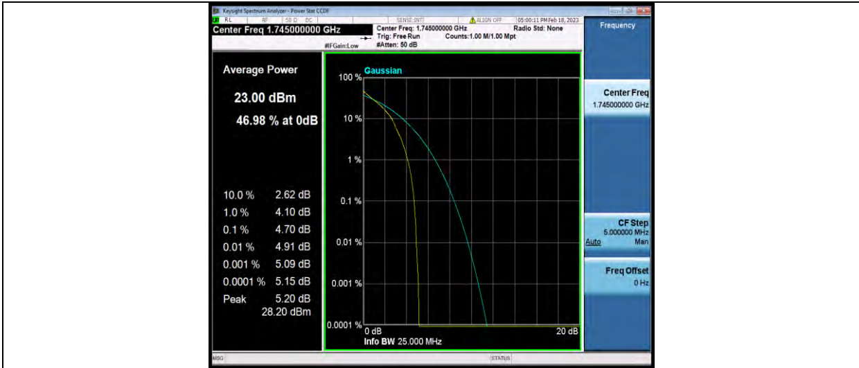
Band66-1.4MHz-QPSK-132322-6RB#0
