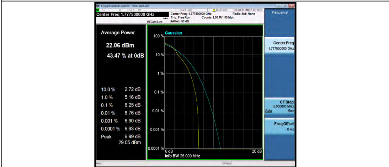
Band66-5MHz-16QAM-132647-25RB#0
