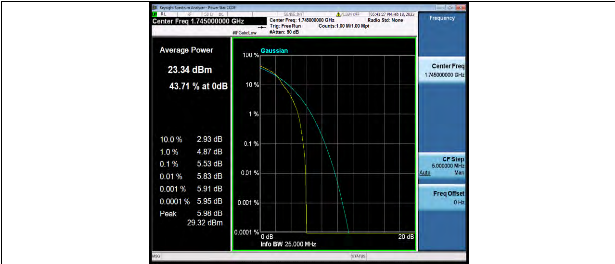
Band66-10MHz-16QAM-132322-50RB#0
