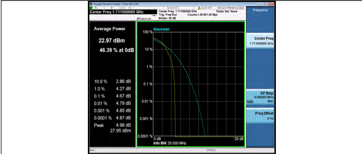
Band66-3MHz-16QAM-131987-15RB#0
