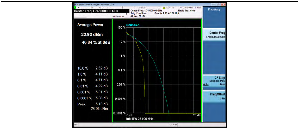
Band66-3MHz-QPSK-132322-15RB#0
