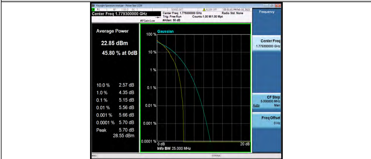
Band66-1.4MHz-QPSK-132665-6RB#0
