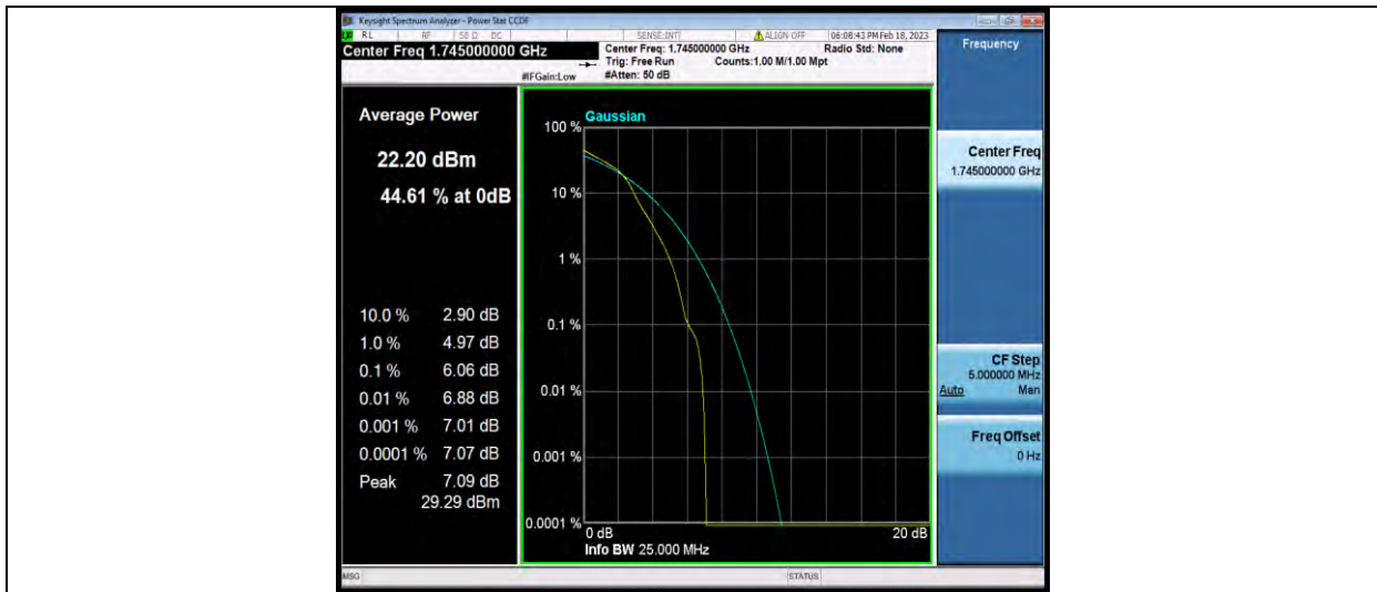
Band66-20MHz-16QAM-132322-100RB#0
