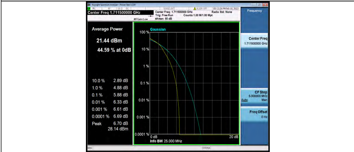
Band66-3MHz-16QAM-132322-1RB#0
