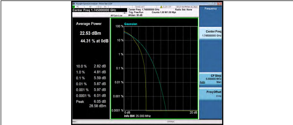
Band66-5MHz-16QAM-132322-25RB#0
