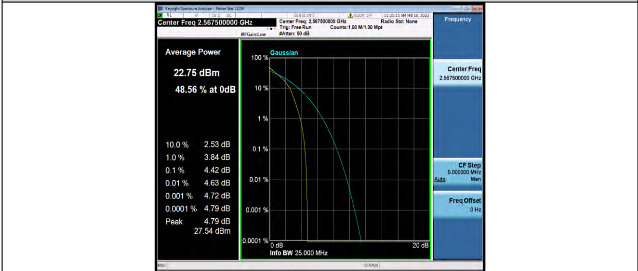
Band7-5MHz-QPSK-21425-25RB#0
