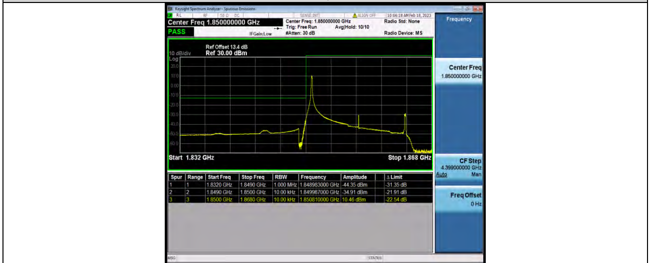
Band2-15MHz-16QAM-18675-75RB#0
