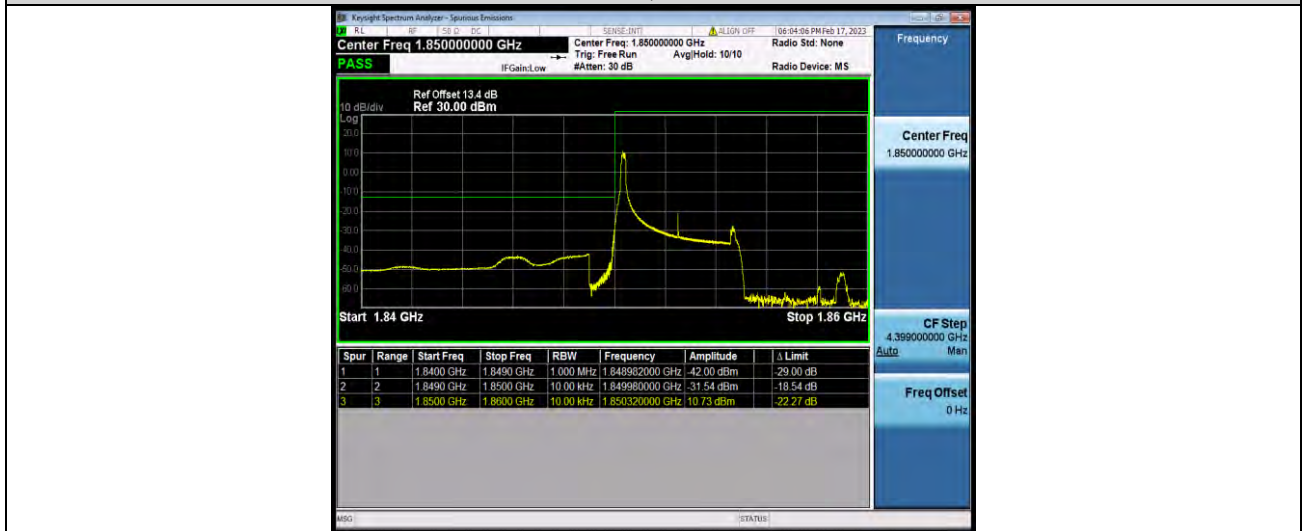
Band2-5MHz-16QAM-18625-1RB#24
