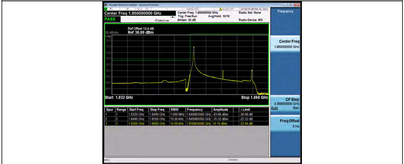
Band2-15MHz-QPSK-18675-75RB#0
