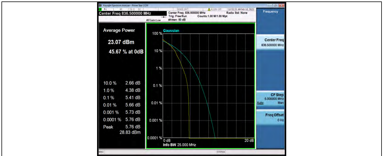
Band5-3MHz-QPSK-20525-15RB#0
