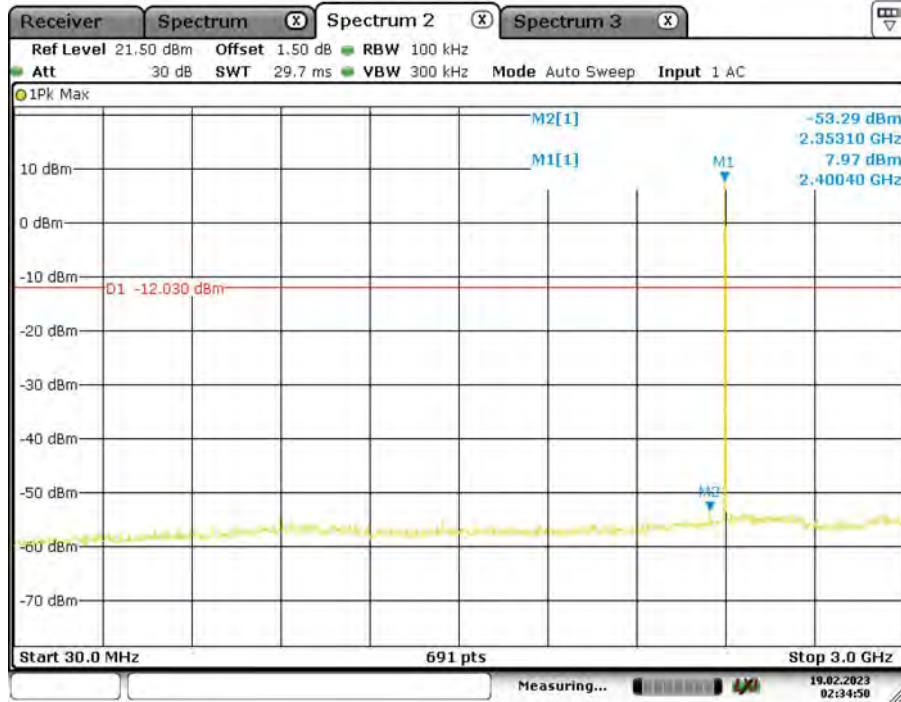
2DH5_Ant1_2402_30~3000
