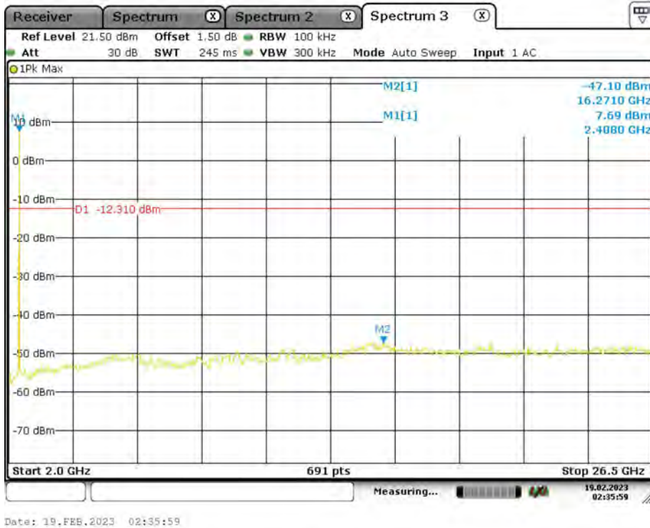
2DH5_Ant1_2402_2000~26500
