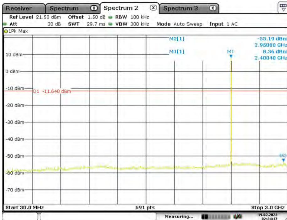
3DH5_Ant1_2402_30~3000
