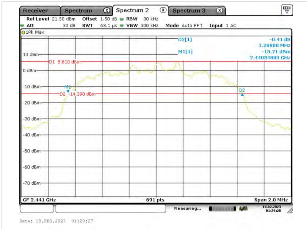
3DH5_Ant1_2441
