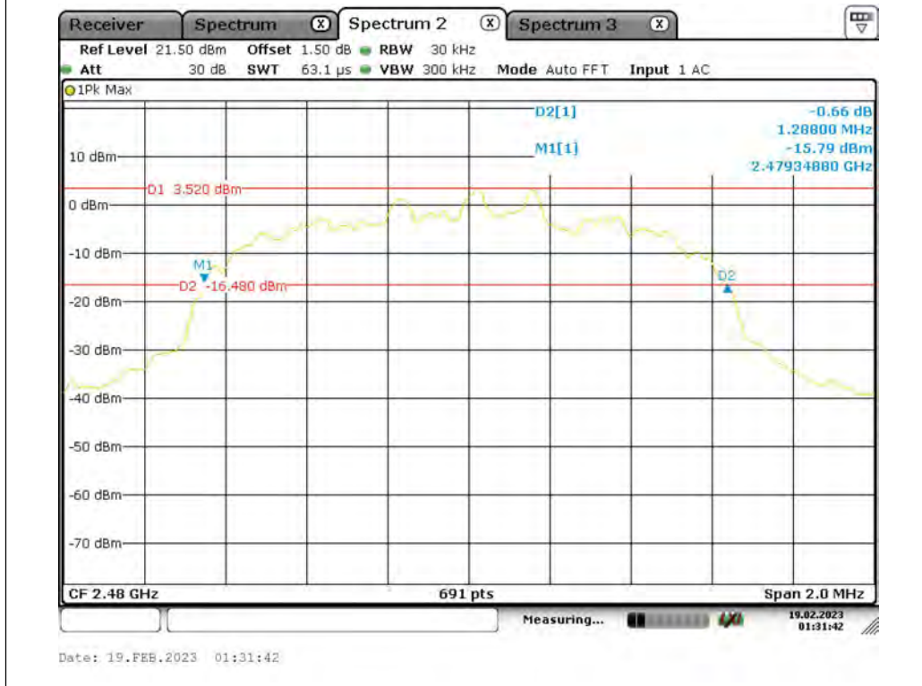
3DH5_Ant1_2480
