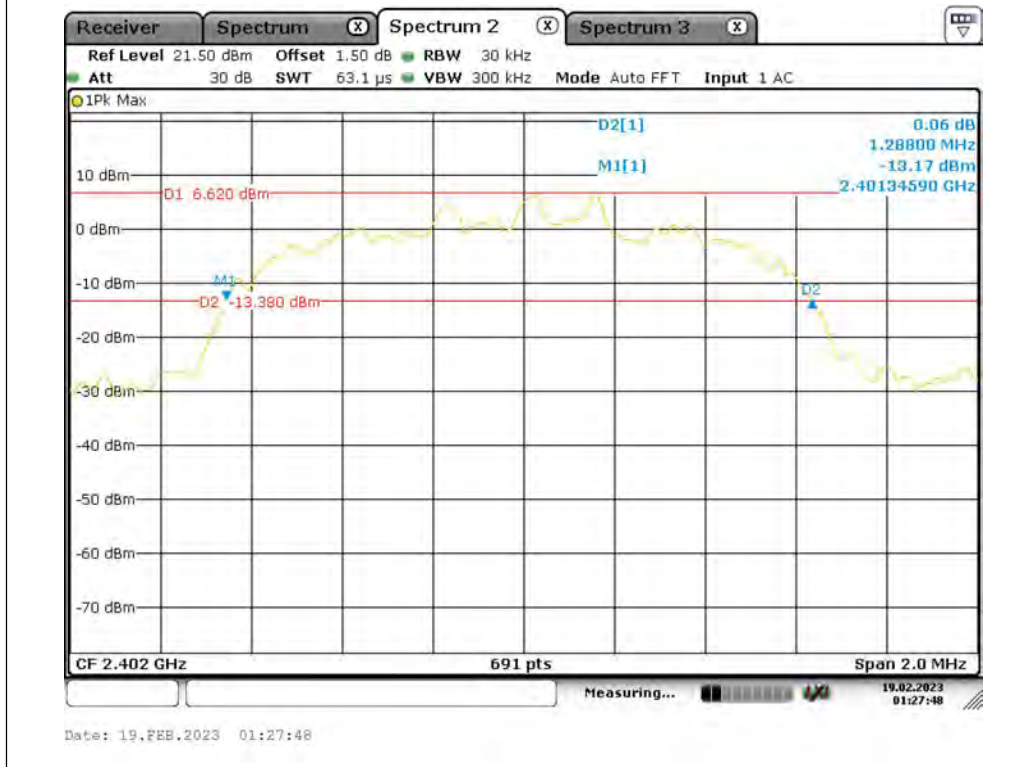
3DH5_Ant1_2402
