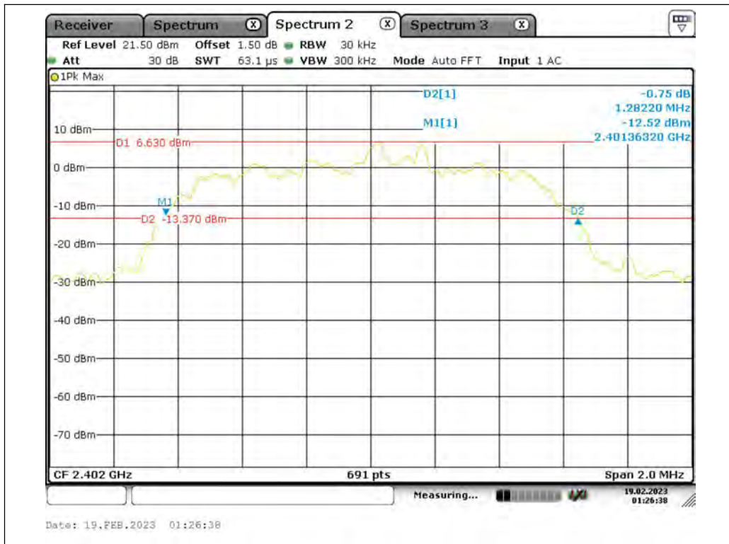
2DH5_Ant1_2402
