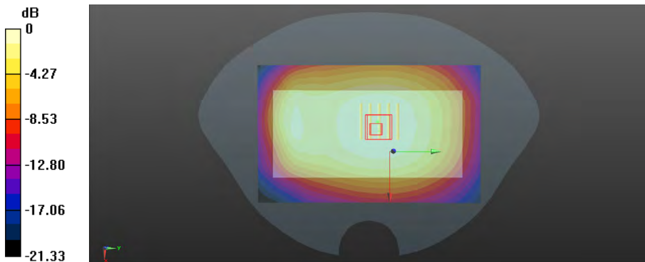
0 dB = 0.258 W/kg
