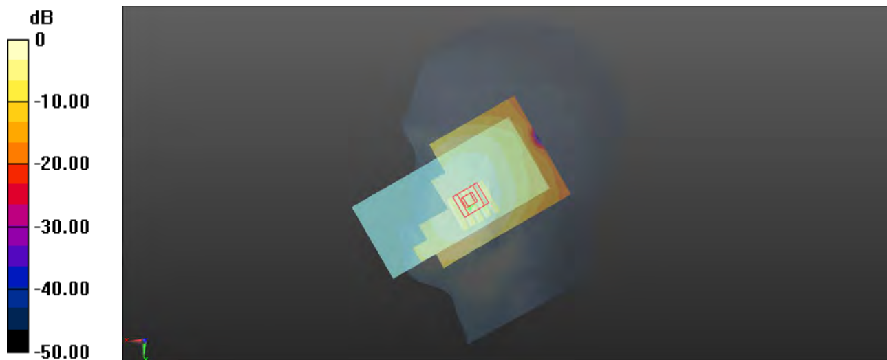
0 dB = 0.145 W/kg
